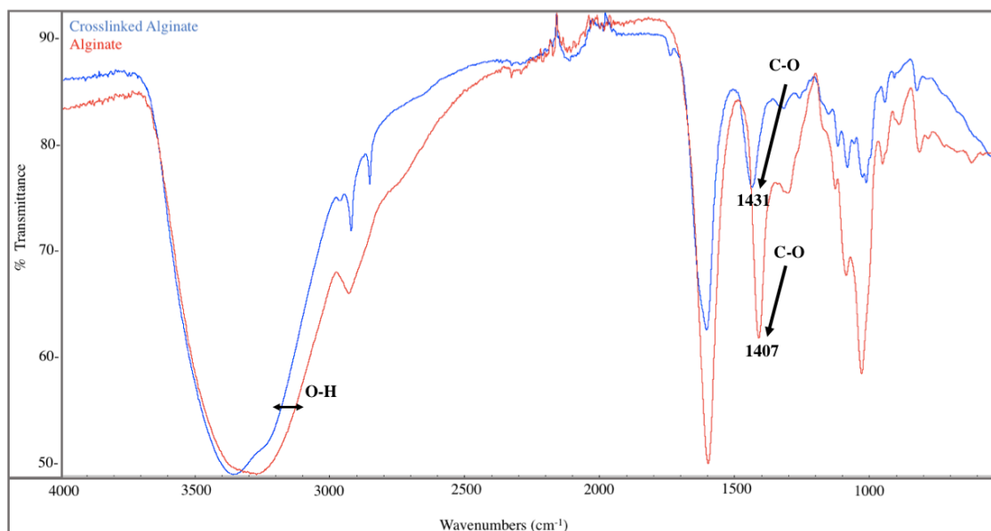
Figure 3.2.1 FTIR spectrum of sodium alginate scaffold (a) and crosslinked alginate scaffold with 1 M \text{CaCl}_2 (b)
