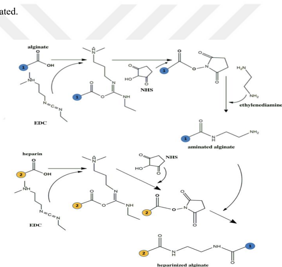
Figure 2.2.3.1 The mechanism of carbodiimide reactions for synthesize heparinized alginate
