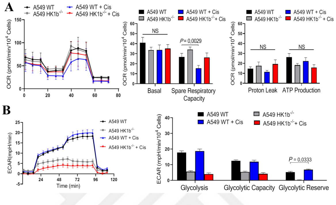
Figure 4.5.1HK1b KO role in cisplatin response on metabolism, A) OCR analysis of untreated or 6hrs cisplatin treated A549 WT and A549 HK1b -/- cells. Experiments were performed twice in quadruplicates for OCR. The results are presented as the mean \pm SEM and means compared with one-way ANOVA and Tukey's post hoc test. B) ECAR analysis of untreated or 6hrs cisplatin treated A549 WT and A549 HK1b -/- cells. Experiments were performed once for quintuple for ECAR. The results are presented as the mean \pm SEM and means compared with one-way ANOVA and Tukey's post hoc test
