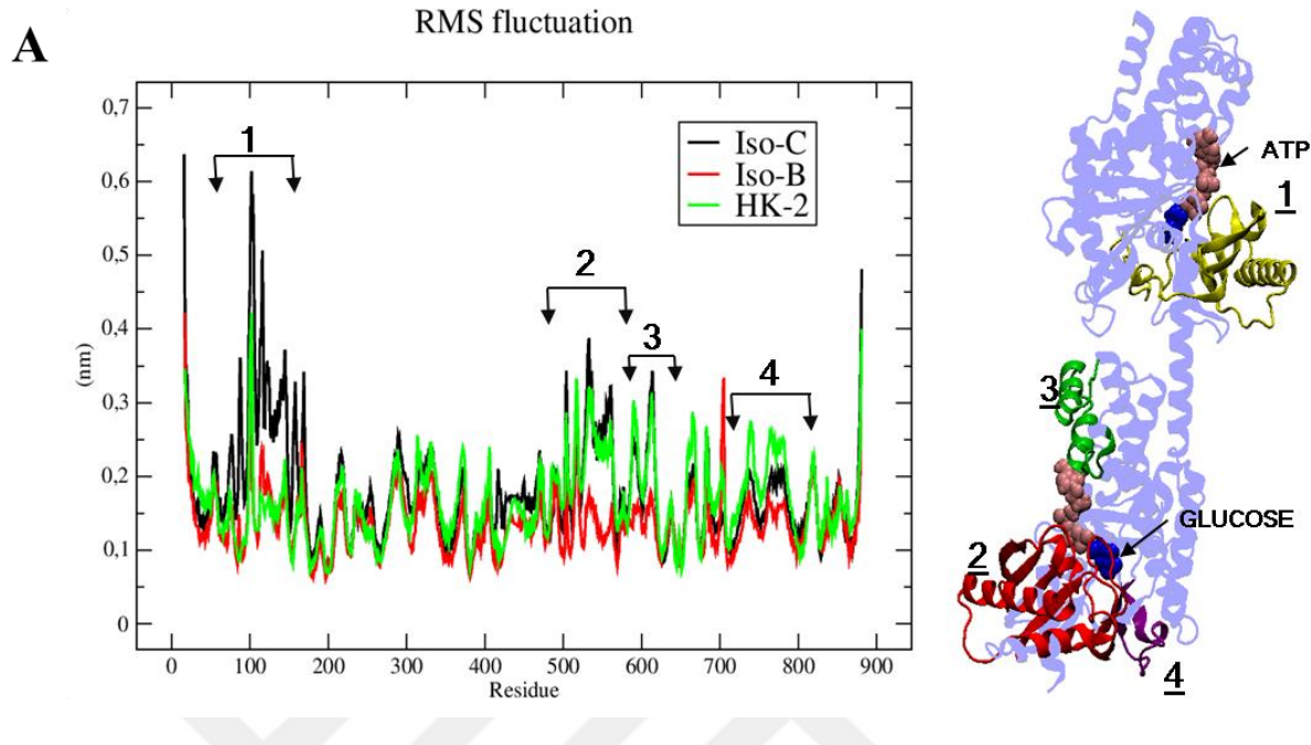
Figure 4.4.1 RMSF Plot shows four major regions fluctuating in HK1c and HK-2 while HK1b is more stable. Structure of HK1c is shown in the figure, first region (1) responsible for ligand binding in N-terminal and a part of small sub-domain (which is responsible for opening and closing of ligands binding pocket), second region (2) ligand binding site in C-terminal part of small sub-domain, third region (3) C-terminal part of large domain and involved in ATP binding, fourth region (4) near to Glucose binding site of C-terminal large domain.
