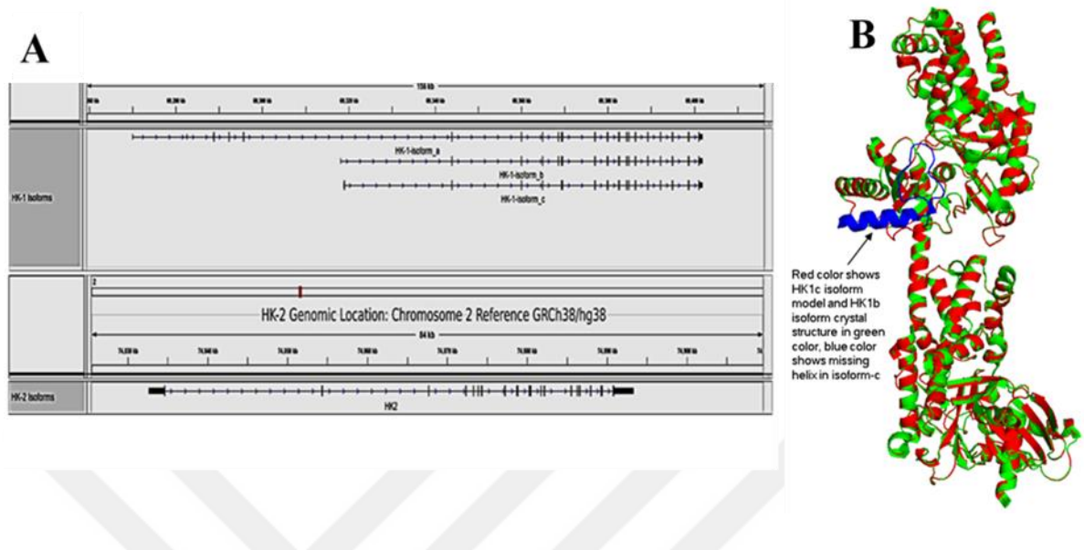
Figure 4.2.1 A) RefSeq gene annotations of HK1 isoforms (HK1a, HK1b and HK1c) and HK2. HK1a and HK1b isoforms possess one extra exon, which is missing in HK1c. B) Structural alignment between crystal structures of HK1b and HK1c model. The extra exon in HK1b, which is shown in blue, codes for 32-amino acid long alpha-helix that is part of the small sub-domain of N-terminus. For the sake of simplicity only one monomer is shown. HK1b isoform levels were elevated in NSCLC tumors compared with normal lung tissue.
