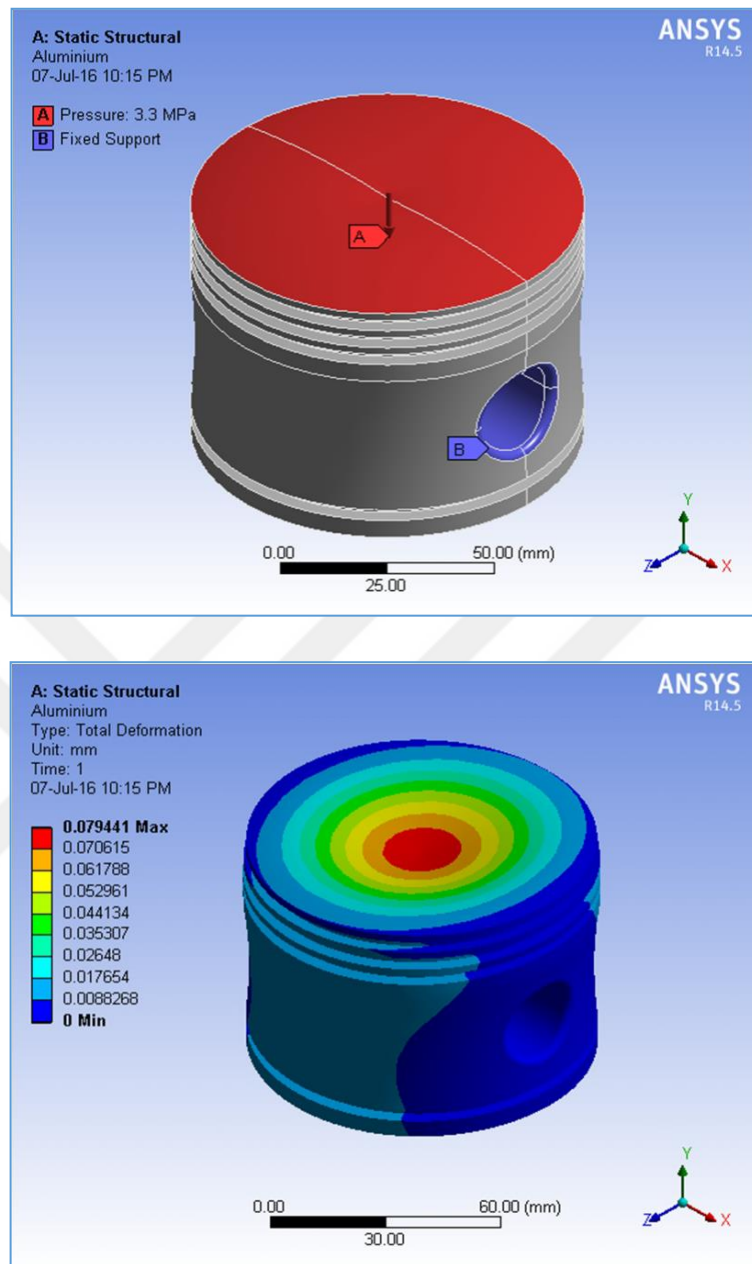
Figure 4.8. Total deformation on piston [52].
