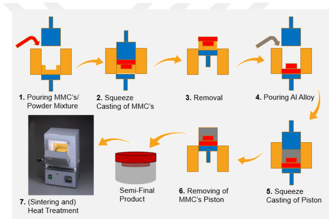
Figure 3.16. Production flow chart of squeeze cast pistons.
