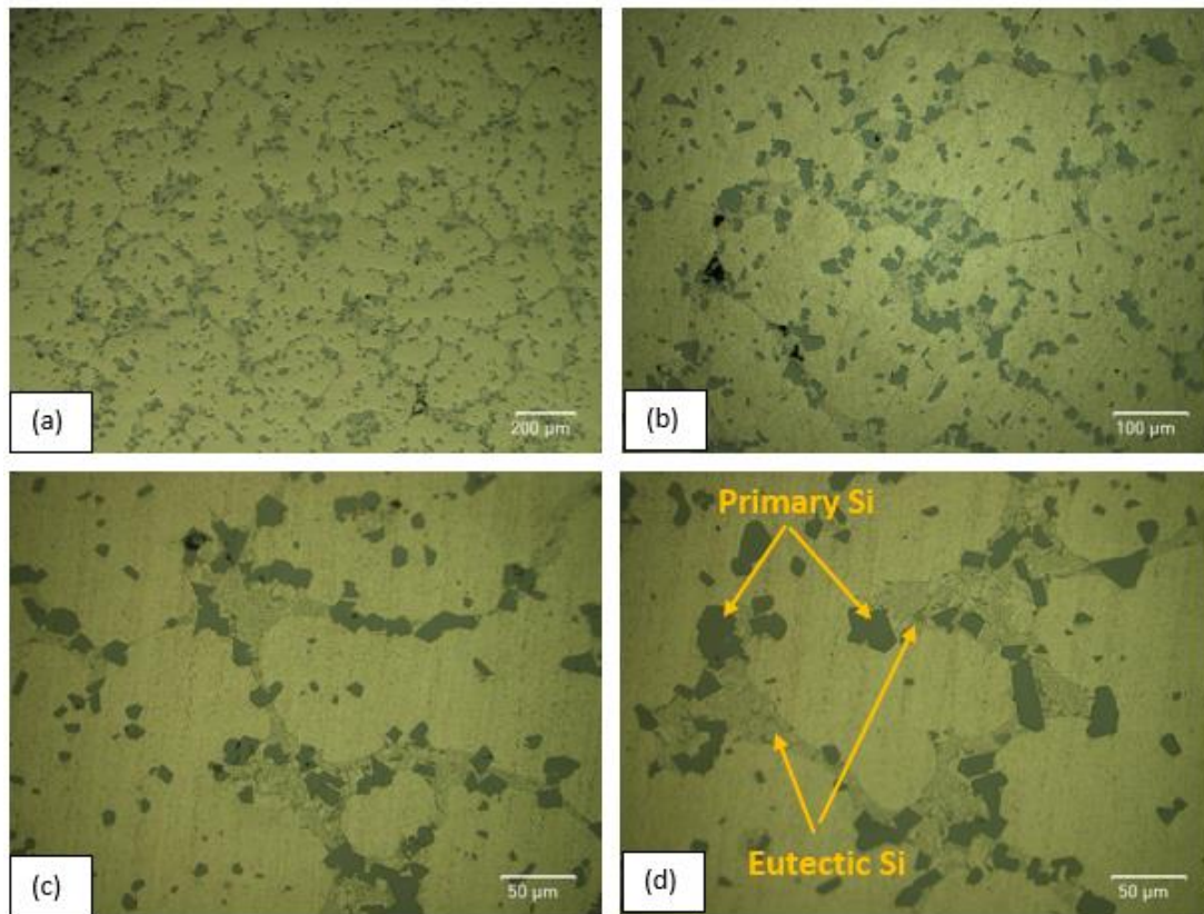
Figure 4.24. As-polished microstructures of the Al alloy part in different magnifications.
