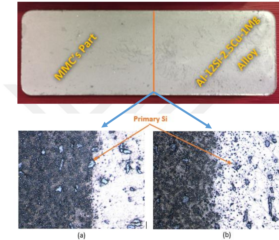
Figure 4.23. Microstructures of the transition part of (a) sample 2 and (b) sample 3 in 200x magnification.
