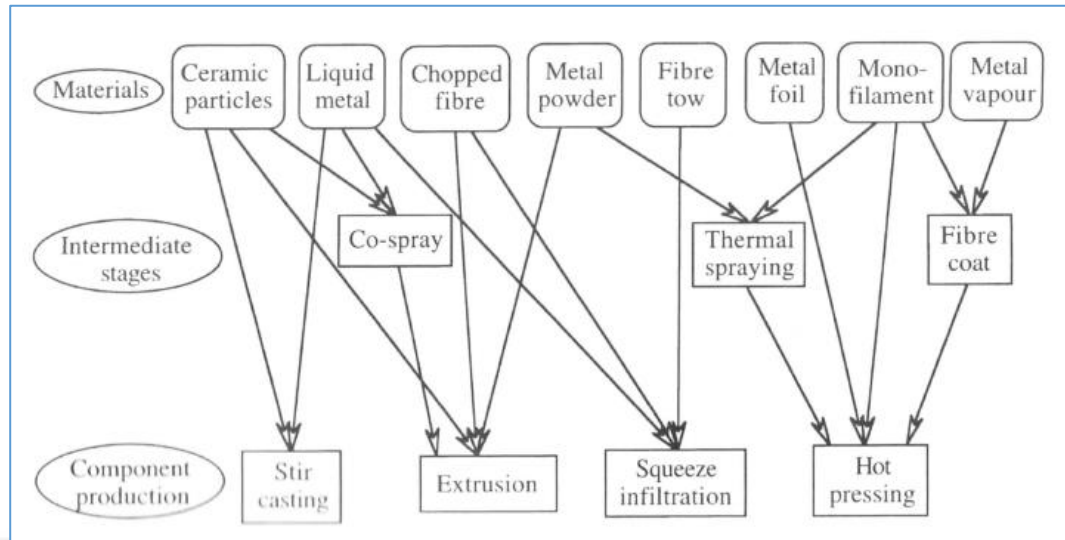
Figure 2.12. Schematic overview of the approaches of fabrication of metal matrix composites [14].
