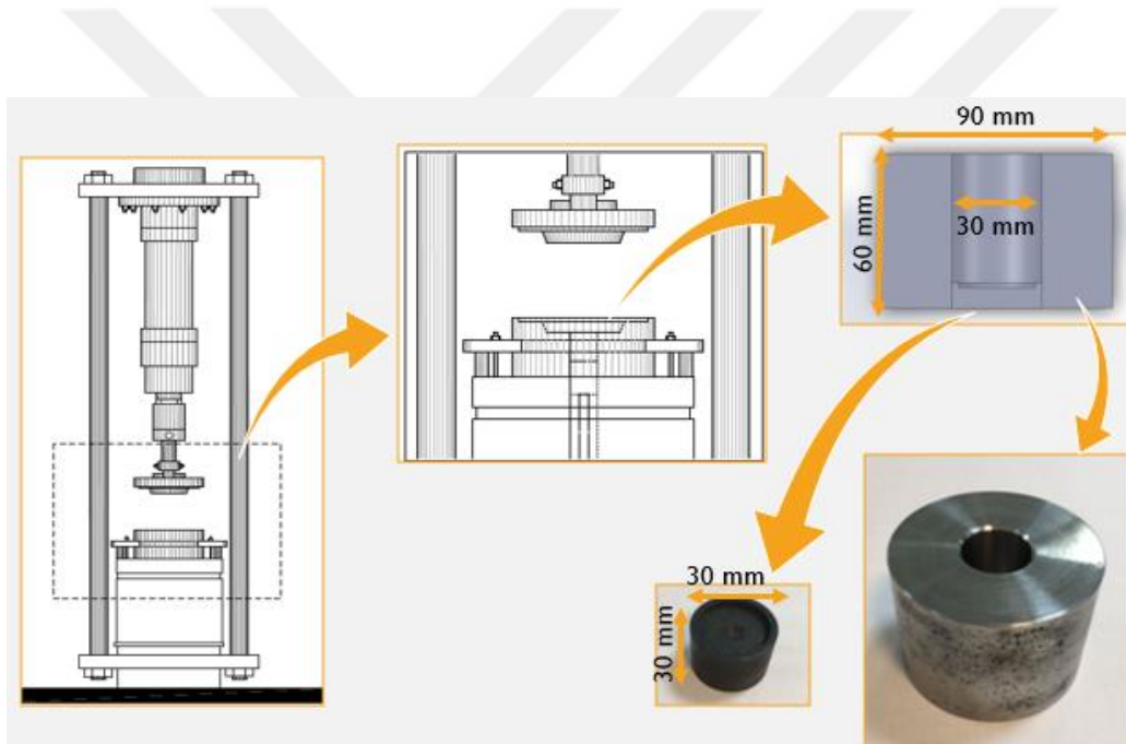
Figure 3.8. Final states of permanent molds used for squeeze casting near-net shape piston studied in this work.
