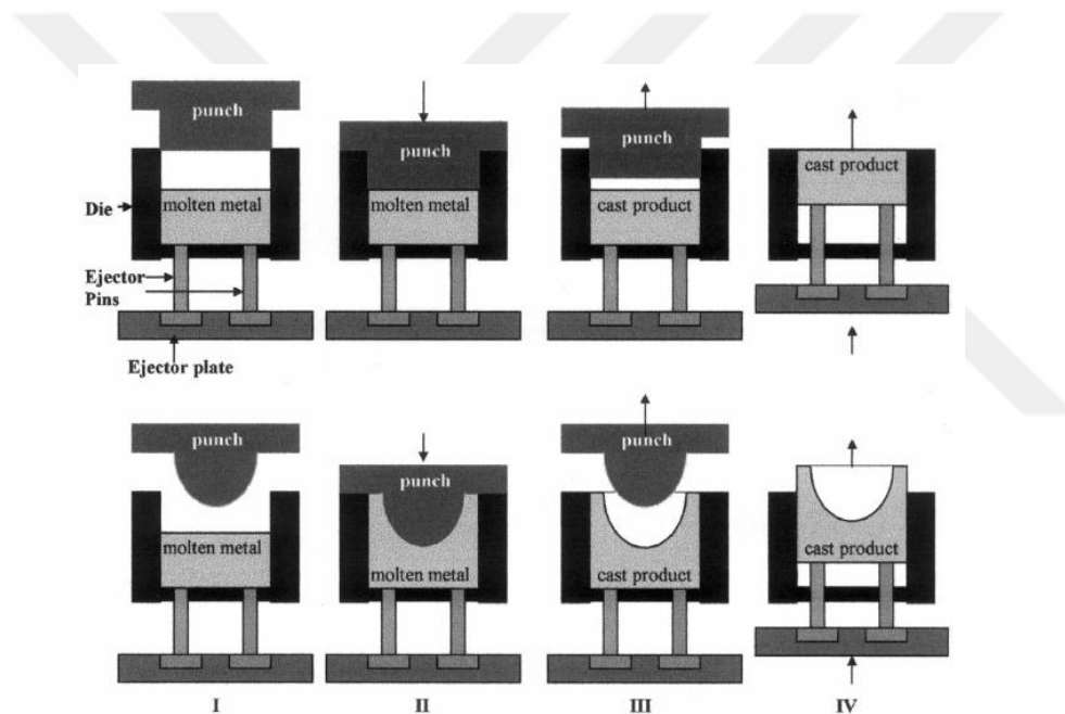
Figure 2.13. Schematic diagram to show two forms of the direct squeeze casting process. [30].
