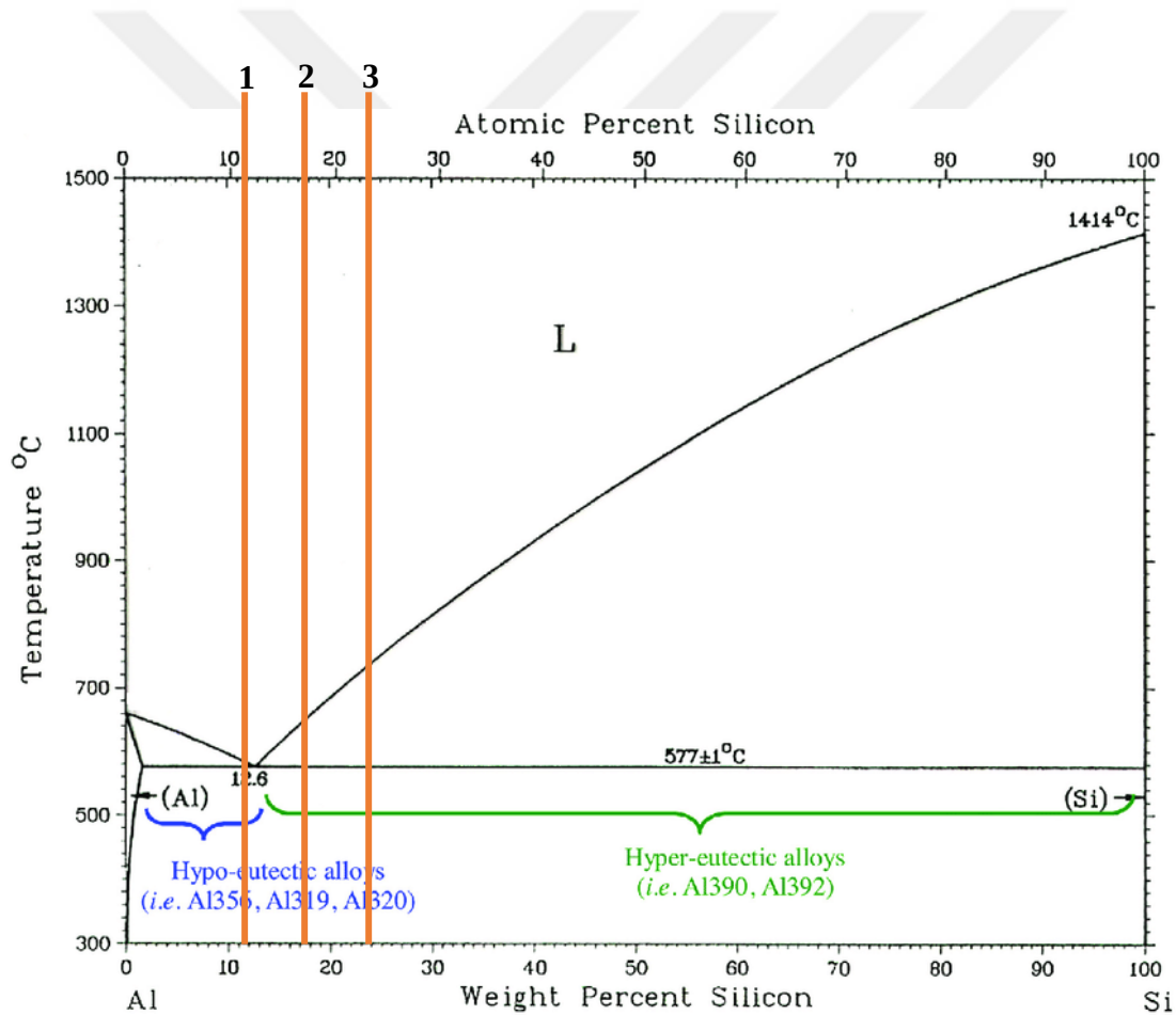
Figure 2.2. Al-Si phase diagram [5].
