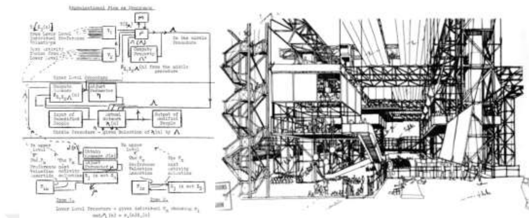
Figure 2.7: (Left) Computing diagram for the Fun Palace, (Right) Drawing of Fun Palace ( https://www.arkitektuel.com/fun-palace-cedric-price/ )
