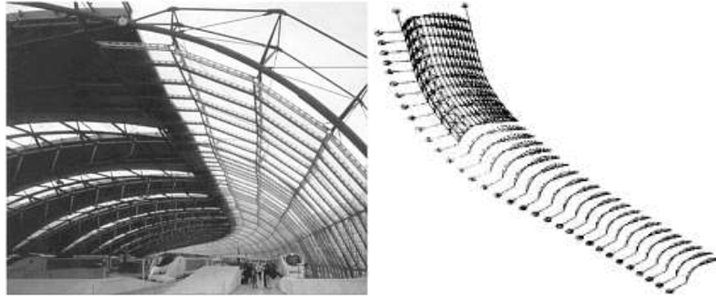
Figure 2.12: (Left) International Terminal, Waterloo Station (1993), London, UK, architect Nicholas Grimshaw and Partners. (Right) 36 dimensionally different, parametrically designed arches (Kolarevic, 2003)
