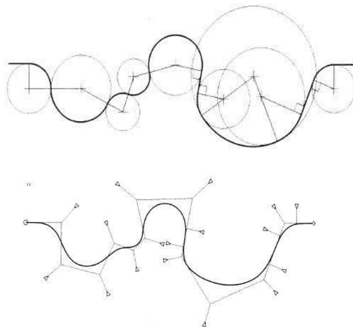
Figure 2.19: (Above) Curves defined by fixed radius and tangency (Below) Similar curve defined by digital geometry (Lynn, 1999)
