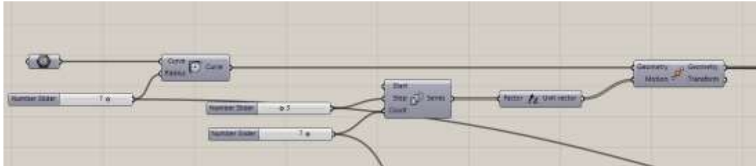
Figure 4.5: Example used Grasshopper code for rounding the corners of plan views and copy in the Z direction at regular interval
