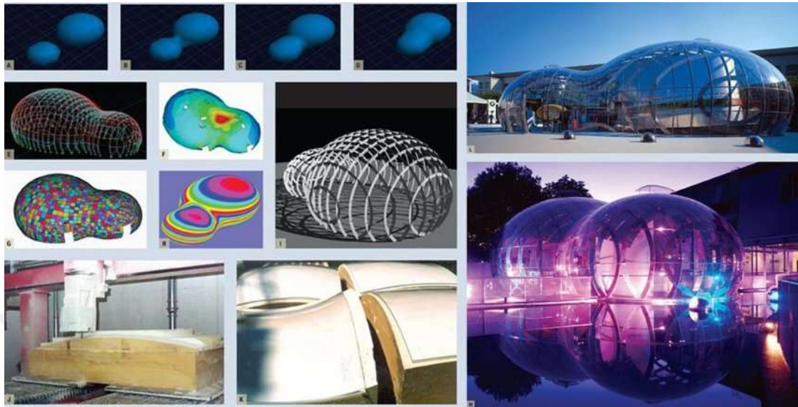
Figure 2.28: Construction of BMW Bubble pavilion, Franken Architekten ( https://www.researchgate.net/figure/BMW-Bubble-pavilion-by-Franken-Architects-18_fig5_334469158 )
