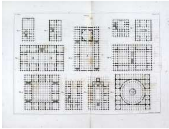
Figure 2.16: Durand's grid system for courtyards( https://www.designactionstudio.com/beyond-nature-1 )
