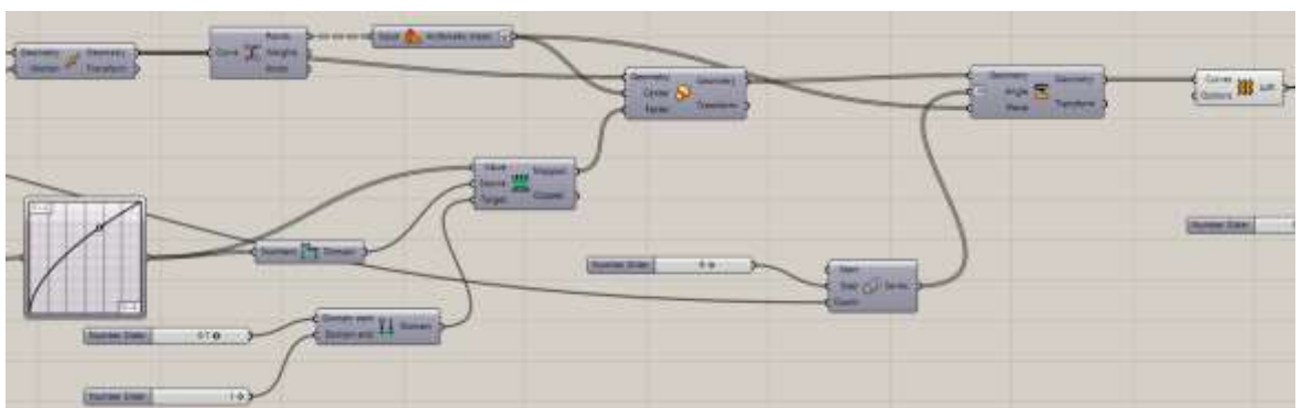
Figure 4.7: Example used Grasshopper code for scaling and rotating the copied curves and lofted surface
