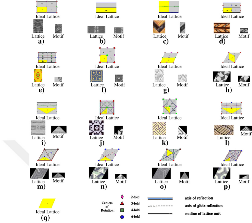
Figure 2.11: Ideal lattice [13], lattices and motifs for 17 Wallpaper Groups [14]:(a) pmm, (b) pm, (c) pg, (d) pmg, (e) cmm, (f) p4, (g) p2, (h) p3, (i) cm, (j) p4m, (k) p4g, (l) pgg, (m) p31m, (n) p6, (o) p3m1, (p) p6m and (q) p1.
