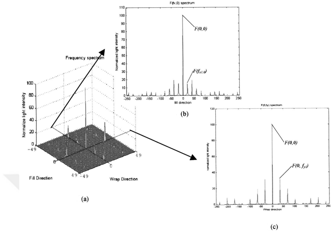
Figure 2.1: Frequency spectrum [3] (a) Portion of faultless fabric frequency magnitude spectrum. (b) Fill direction frequency spectrum. (c) Wrap direction frequency spectrum.
