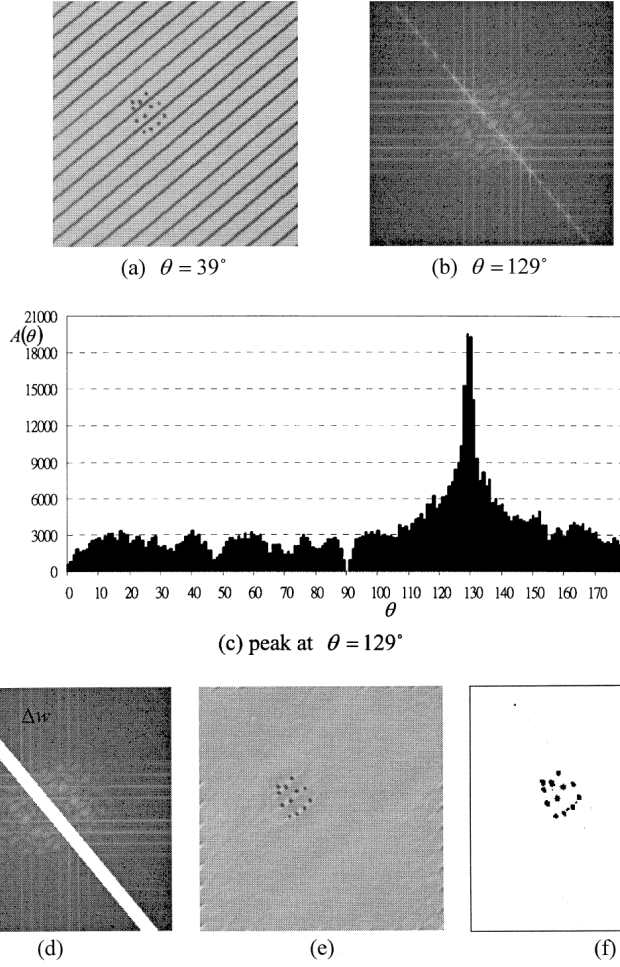
Figure 2.2: A line-structural texture example from [4] with dot-spot defect: (a) The original image; (b) The Fourier domain image; (c) The slope-angle histogram in the Hough space; (d) The notch that contains high-energy frequency components; (e) The restored image; (f) The detected dot spots displayed as a binary image.
