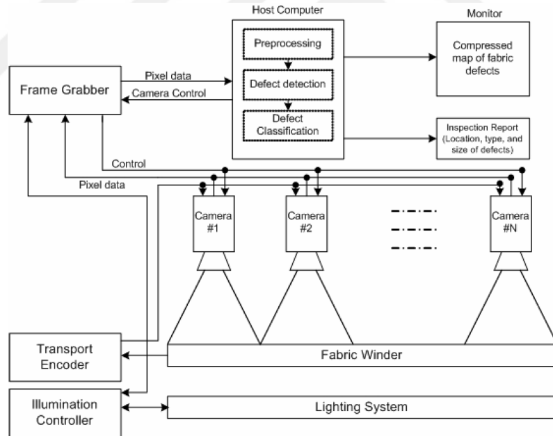
Figure 1.2: Architecture of a typical automated visual inspection system for textile web [2].
