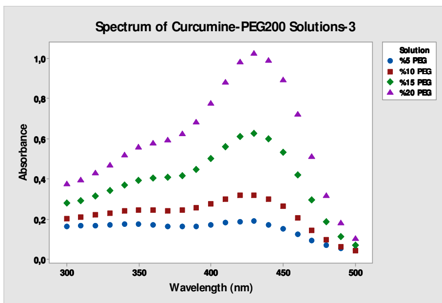
Figure 6.3: Spectrum of Curcumin-PEG200 Solutions, third group.
