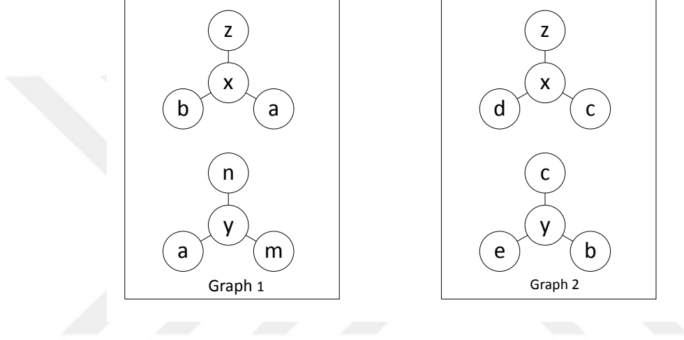
Figure 5.1: The neighbors of x and y in both graphs
