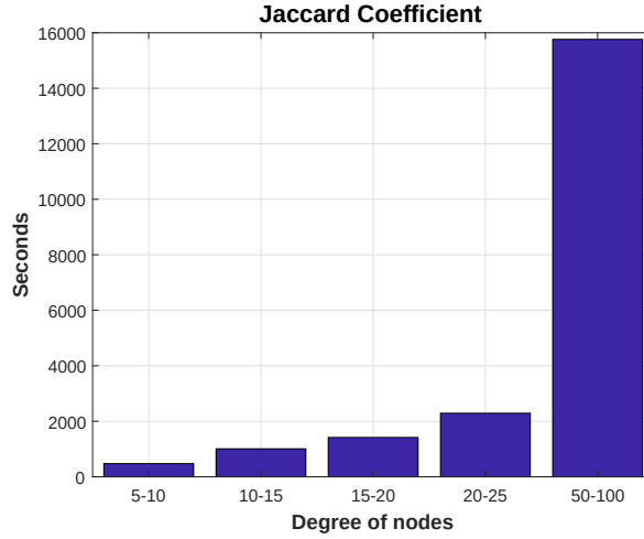
Figure 5.7: Performance of Jaccard's coefficient
