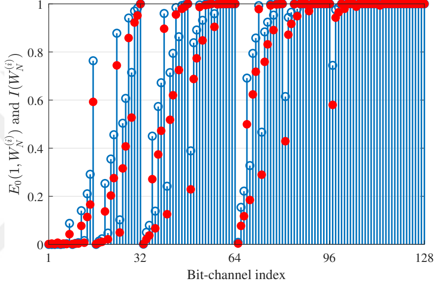
Figure 2.7: Bit-channel cutoff rates (solid circles) and bit-channel mutual information (hollow circles) at an SNR value of 2.5 dB.
