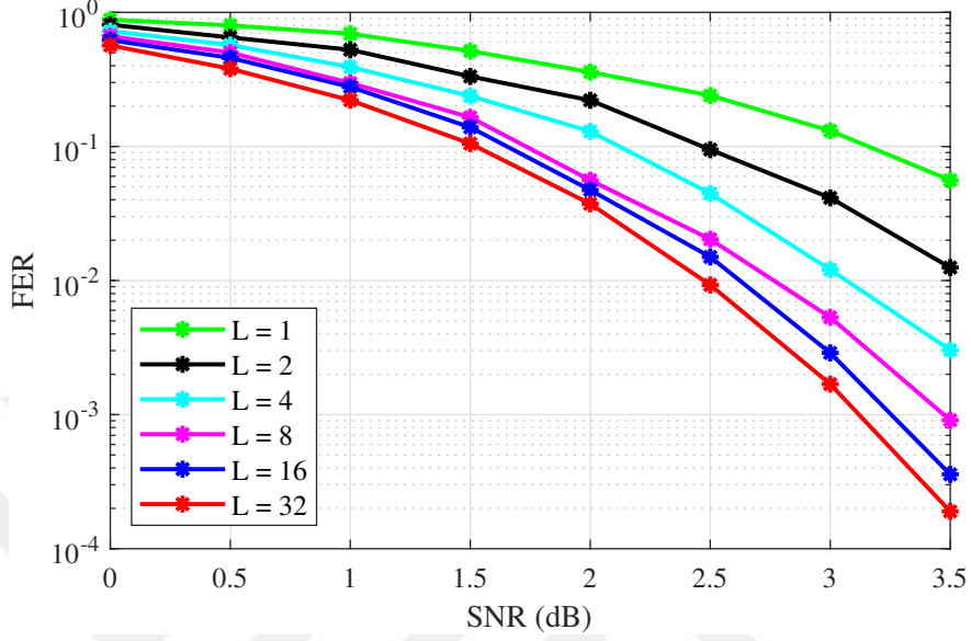
Figure 2.9: Performance of polar codes under list decoding.
