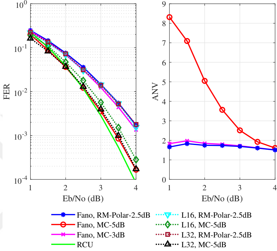
Figure 4.12: Error-correction performance and complexity of PAC(64, 32) codes.
