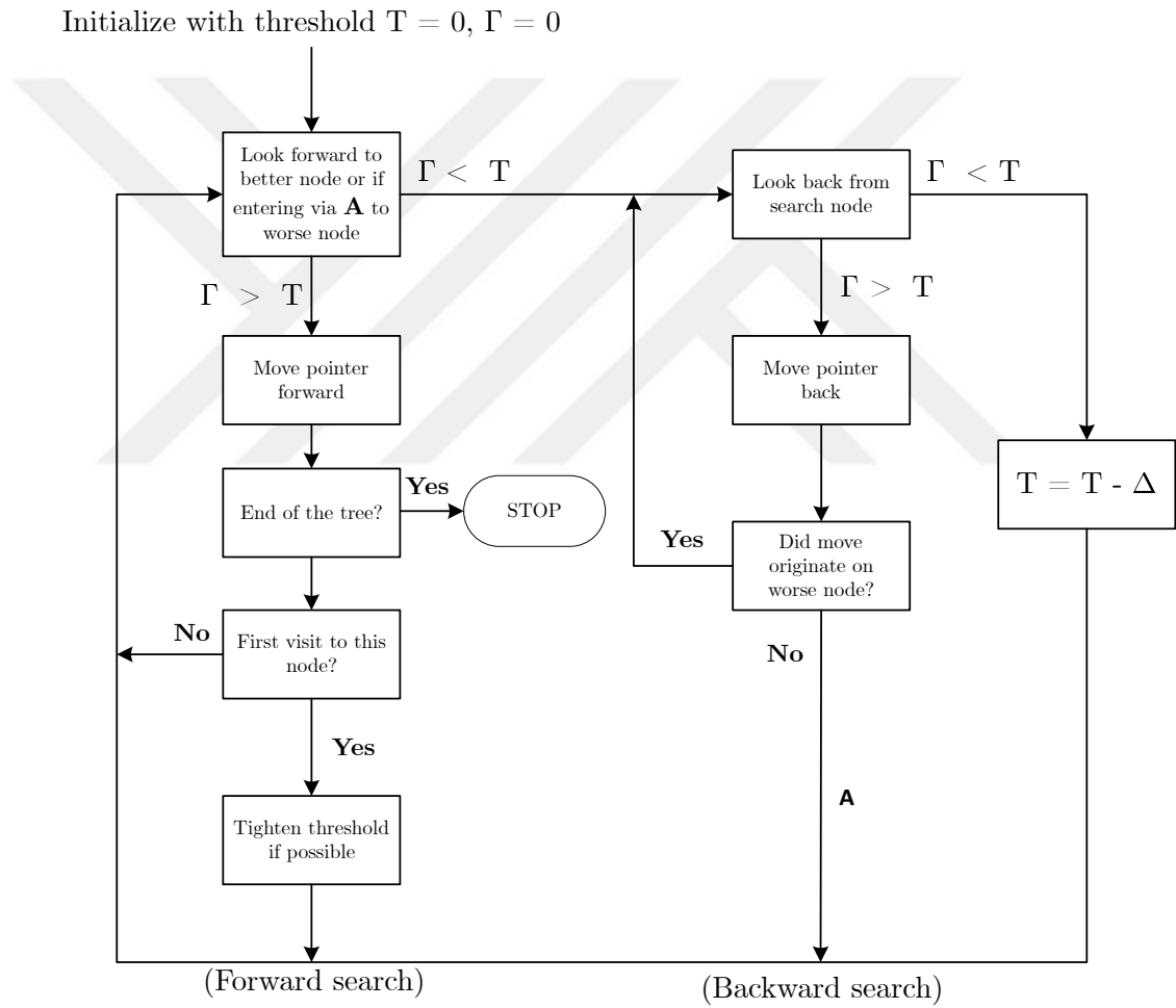
Figure 2.14: Flowchart of the Fano sequential decoding algorithm for a binary tree.
