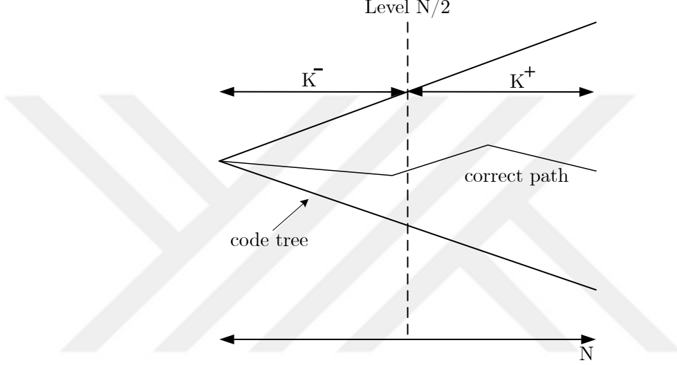
Figure 4.4: Decoding tree of PAC codes after one step polarization.
