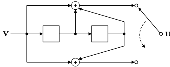
Figure 2.11: Convolutional encoder example.
