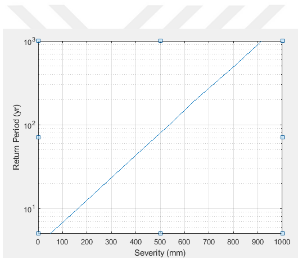
Figure 5.11 Drought Frequency line based on the annual synthetic data of Region 1
