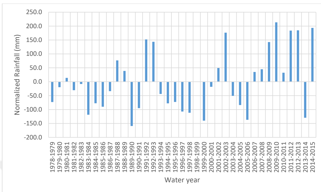
Figure 5.4 Normalized average observed annual rainfall data of Region 1
