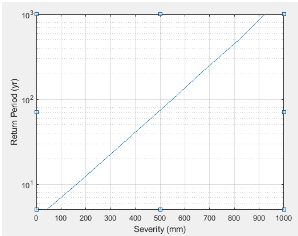
Figure 5.13 Drought Frequency line based on the annual synthetic data of Region 2
