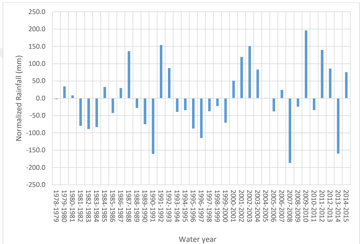
Figure 5.3 Normalized average observed annual rainfall data of North Cyprus
