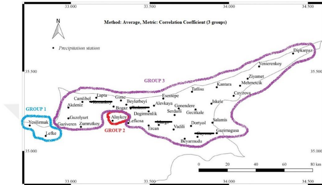
Figure C. 1 Average-Correlation combination with 3 clusters
