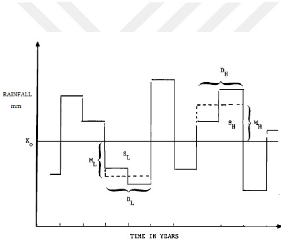
Figure 4.2 Main component of the runs of an annual series. Note. Reprinted from “On the Definition of Droughts”, by Dracup et al., 1980, Water Resources Research, 16(2), p.299.
