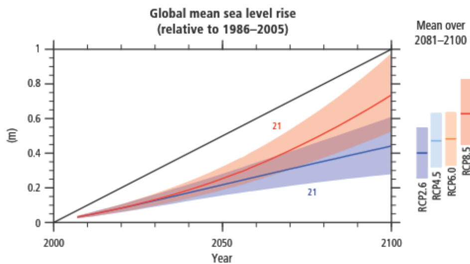
Figure 1.5. IPCC Climate Change: 2014 Synthesis Report Sea-level Rise Future Projections
