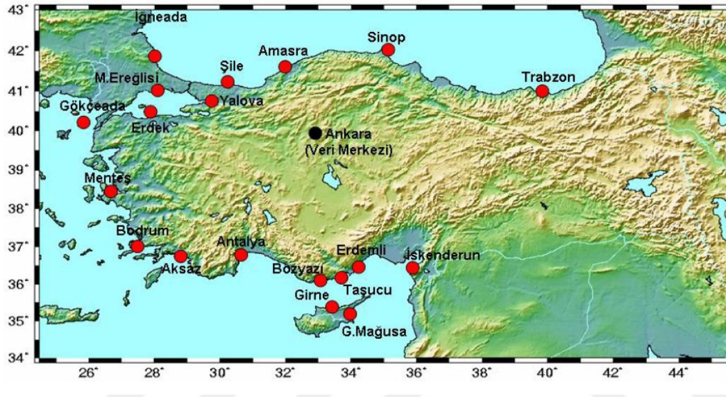
Figure 2.11. TUDES (Turkish National Sea Level Monitoring System) Stations in Turkey (Simav et al, 2012).
