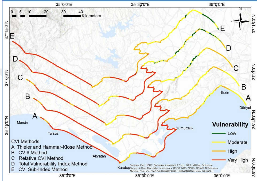
Figure 4.3. CVI methods comparison map of the Adana region (A: Thieler and Hammar Klose Method, (Thieler and Hammar-Klose, 2000), B: CVI 6 (Gornitz et al., 1997), C: Relative CVI method (Palmer et al., 2011), D: Total Vulnerability Index (Szlafsztein and Sterr, 2007), E: CVI Sub-Index method (McLaughlin and Cooper, 2010).
