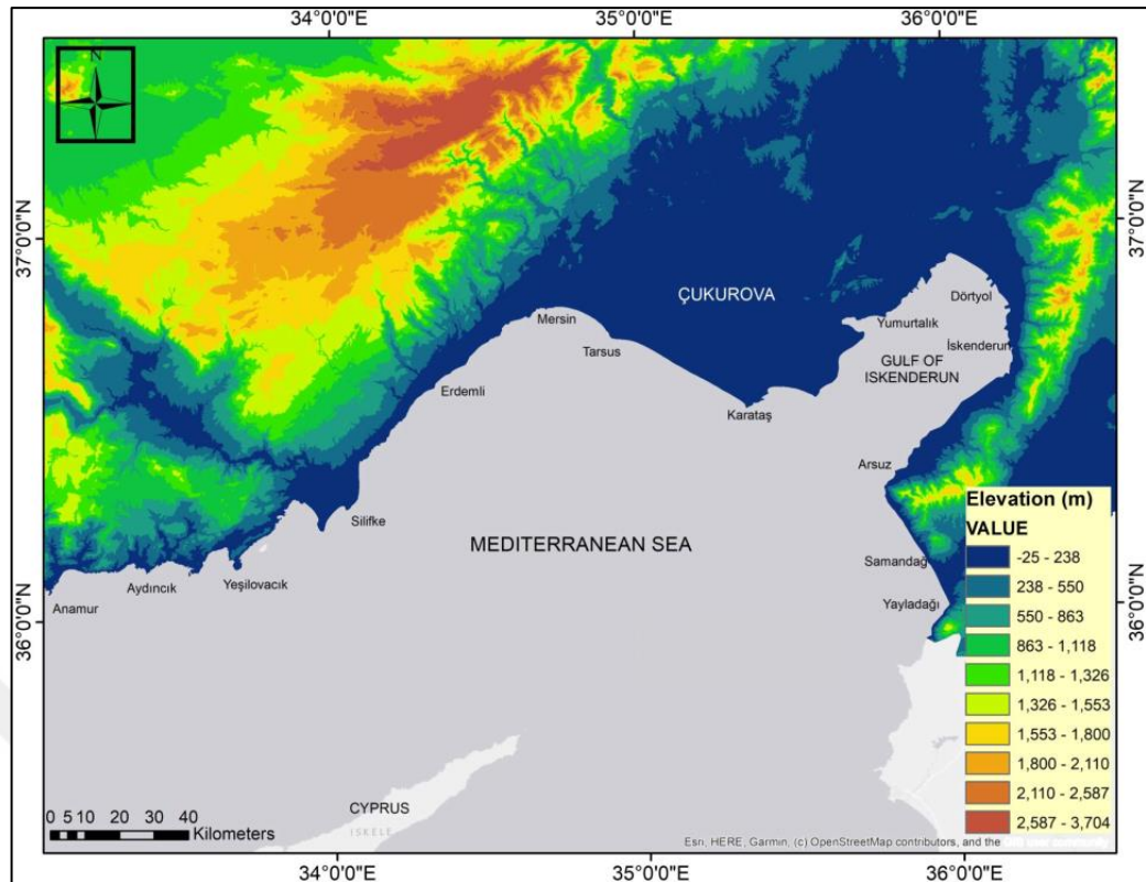
Figure 2.1. SRTM Digital Elevation Model Map
