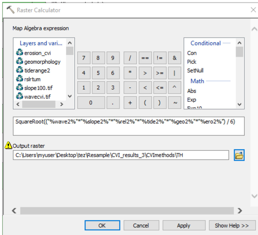
Figure 3.6 Raster calculator tool interface. The raster files that can be used for calculations are shown in the upper left. On the upper right, there are mathematical operators. The formula for the Thieler and Hammar-Klose method is shown in the middle row. The bottom line includes the output location.
