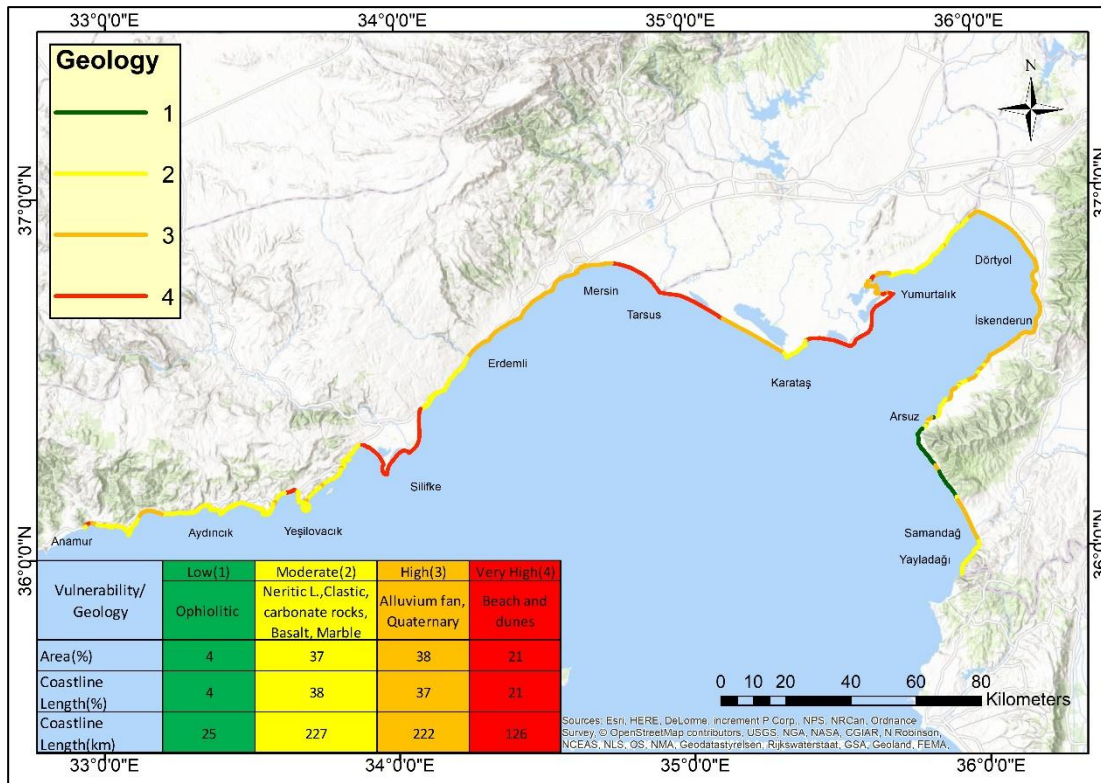
Figure 3.10. Geology classification map of the study area
