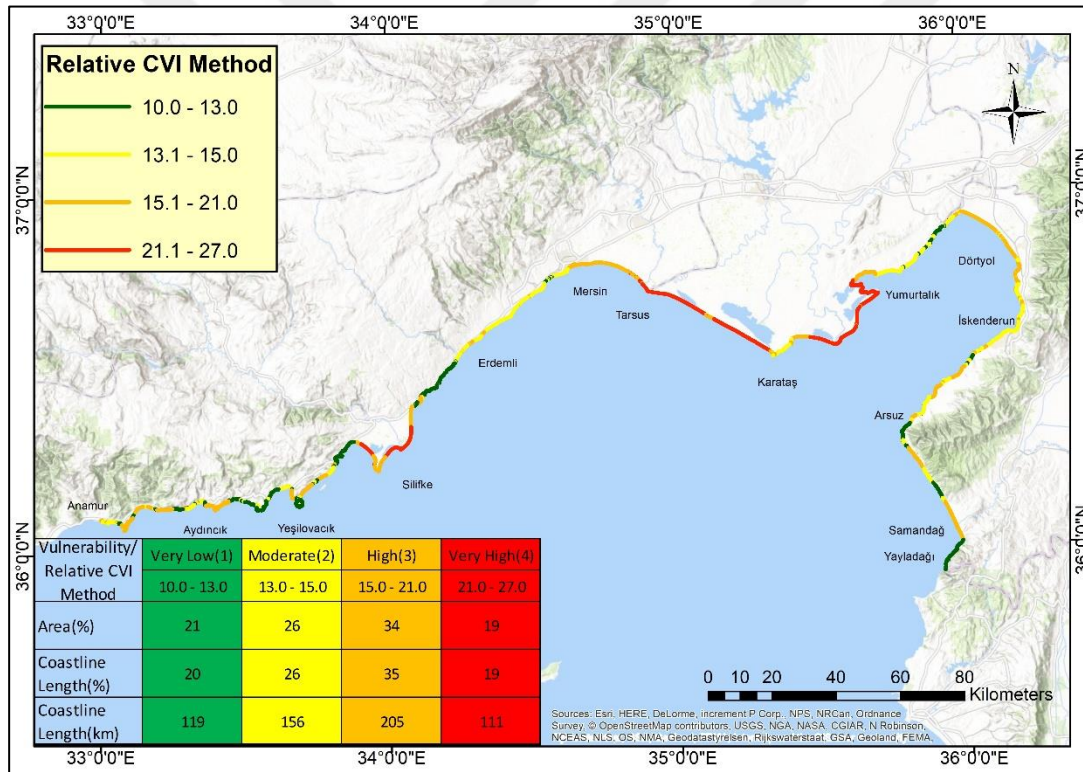
Figure 3.21. CVI map based on Relative CVI method.
