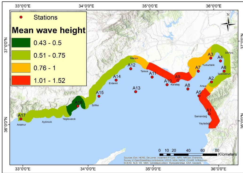
Figure 2.10. Location of 17 station in Buyruk, 2019 research and interpolated mean wave height model was digitized according to the data.
