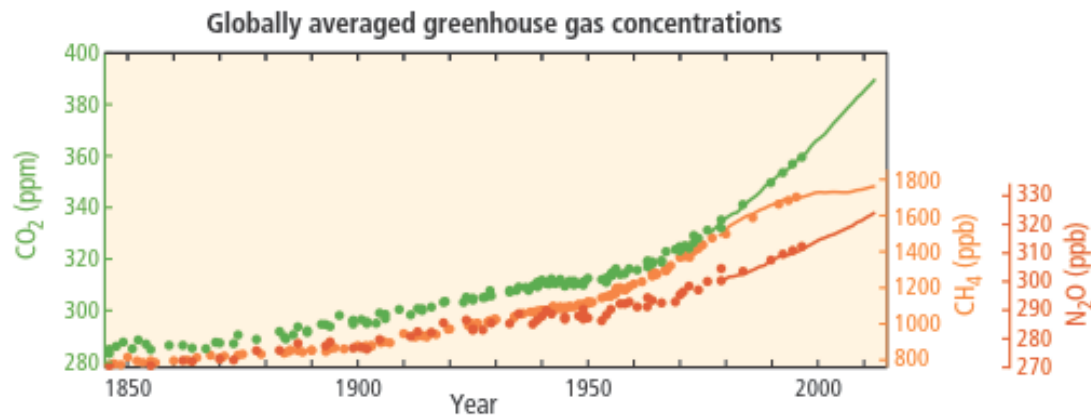
Figure 1.2. Atmospheric concentrations of the heat trapping gases. Green line and dots represent carbon dioxide (CO 2 ) concentration, orange line and dots represent methane (CH 4 ) concentration, red lines and dots represent nitrous oxide (N 2 O) concentration. Lines determined from direct atmospheric measurements. Dots determined from ice core data. (IPCC, 2014)
