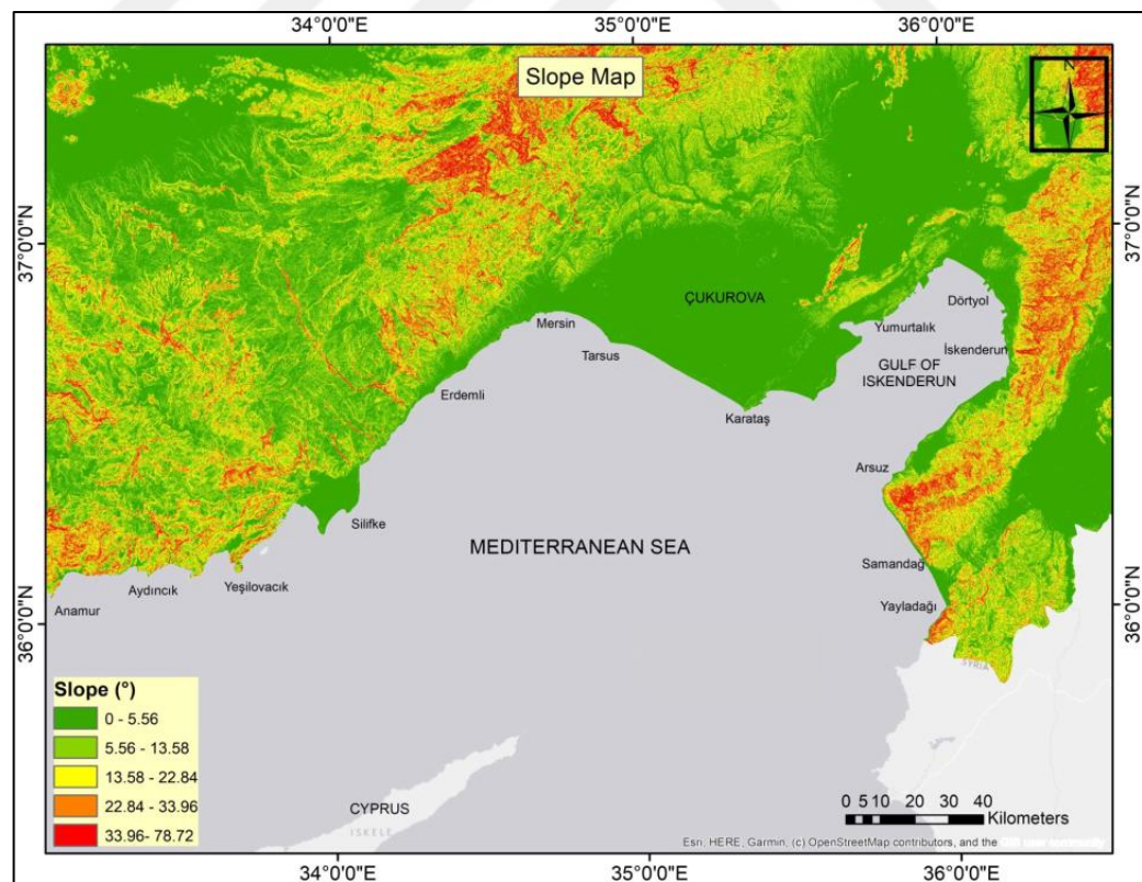
Figure 2.2. Slope Map of the Study Area
