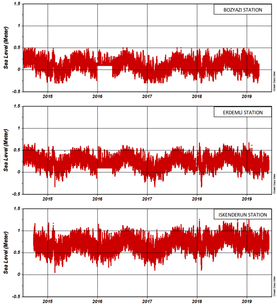
Figure 2.12. Sea level time series data in Bozyazı, Erdemli and İskenderun tide-gauge stations.
