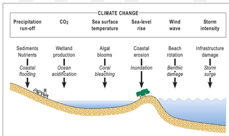
Figure 1.4. The potential impacts of the climate changes on coastal zones (Short and Woodroffe, 2009)
