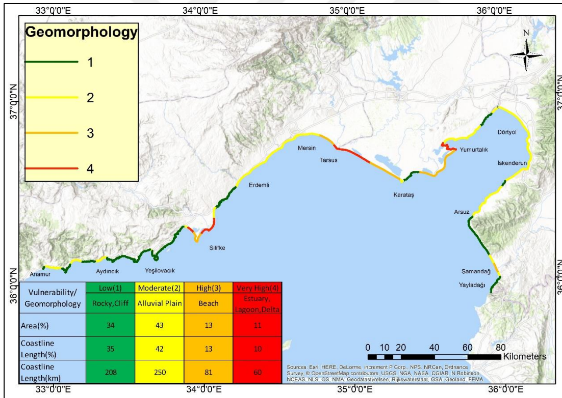
Figure 3.9. Coastal vulnerability map based on geomorphology. The geomorphological landforms and corresponding vulnerability classes are given in inset table.
