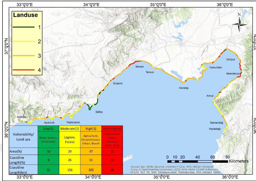
Figure 3.15. Land use classification map of the study area
