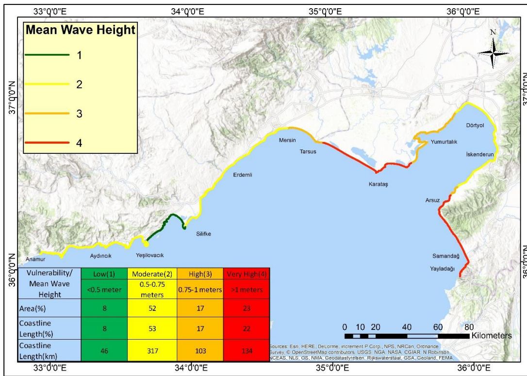
Figure 3.12. Coastal vulnerability classification based on mean wave height values.
