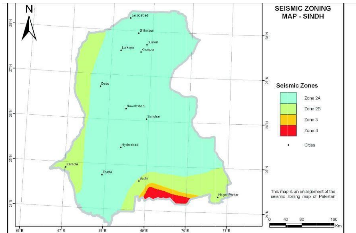
Figure 3. 5 Seismic Zoning Map of Sindh (BCP; 2007)
