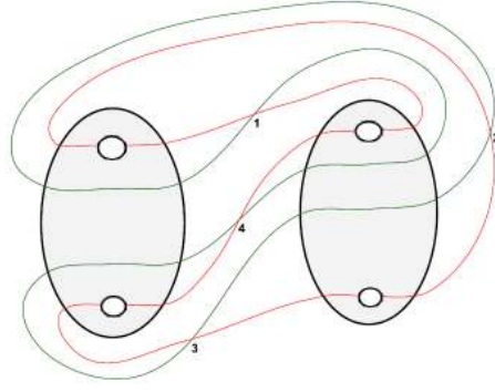
Figure 4.90 A model of the case when n_2 = 2 and s = 1 for \gamma .
