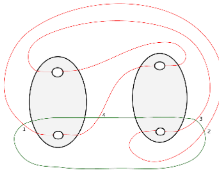
Figure 4.92 A model of the case when n_2 = 2 and s = 1 for \gamma' .
