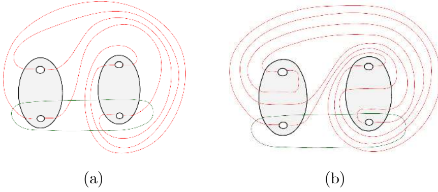
Figure 4.41 a) \Gamma_A after bypass along 3 - 4 - 5 , 7 - 8 - 9 , and 8 - 9 - 10 , b) \Gamma_A after bypass along 6 - 7 - 8 .
