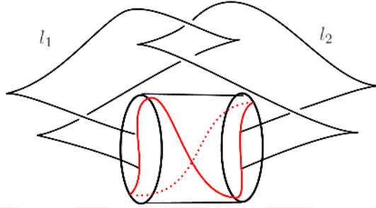
Figure 4.14 Model for a non-destabilizable tangle in B_{out} .
