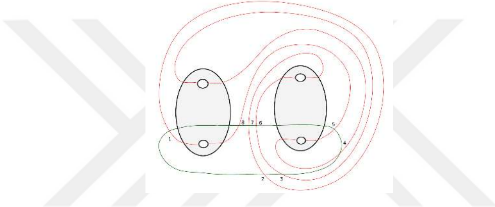
Figure 4.96 A model of the case when n_2 = 2 and s = 3 for \gamma' .
