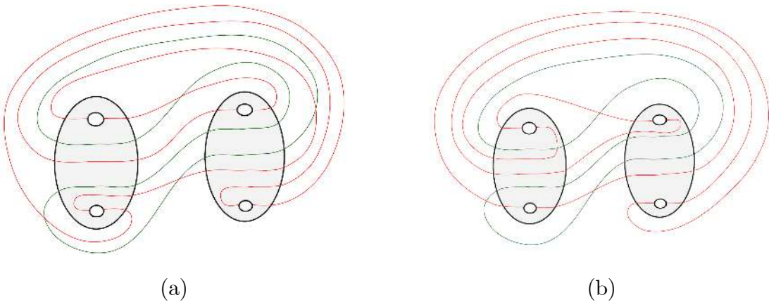
Figure 4.31 a) \Gamma_A after bypass along the arc 2 - 3 - 4 , b) \Gamma_A after bypass along the arc 4 - 1 - 2 .
