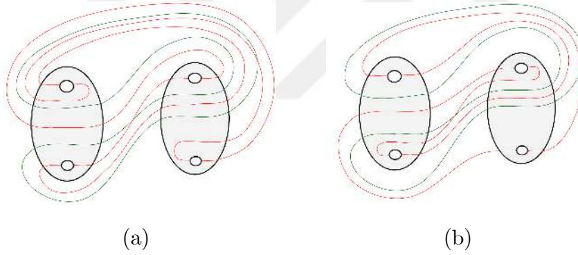
Figure 4.91 a) \Gamma_A after bypass along 1-2-3 , b) \Gamma_A after bypass along 3-4-1 .
