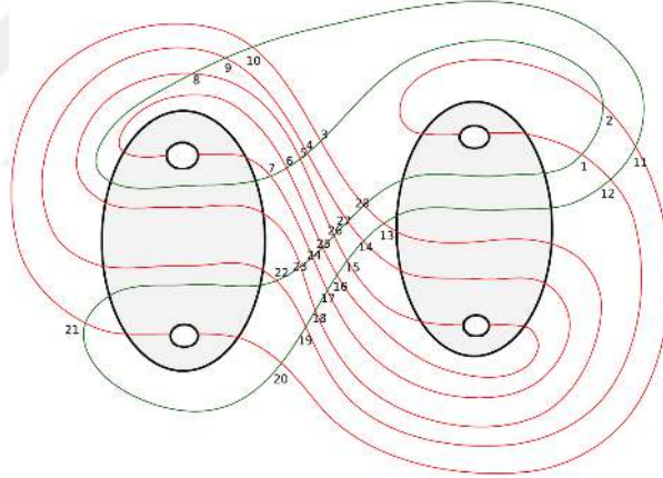
Figure 4.52 A model of the case when n_2 = 4 and s = -5 for \gamma .
