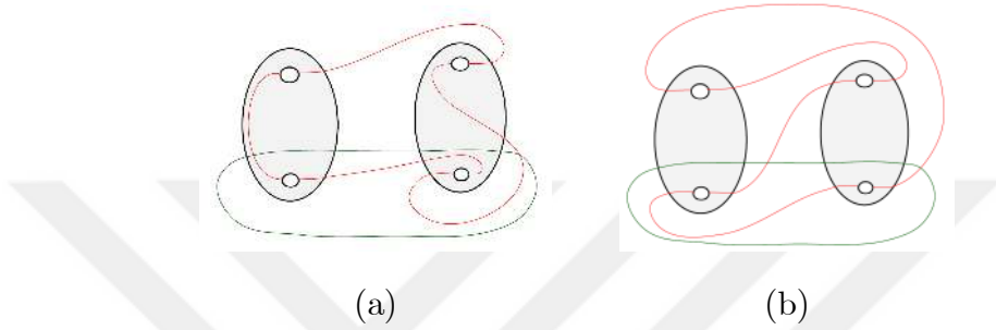
Figure 4.93 a) \Gamma_A after bypass along 2 - 3 - 4 , b) \Gamma_A after bypass along 4 - 1 - 2 .
