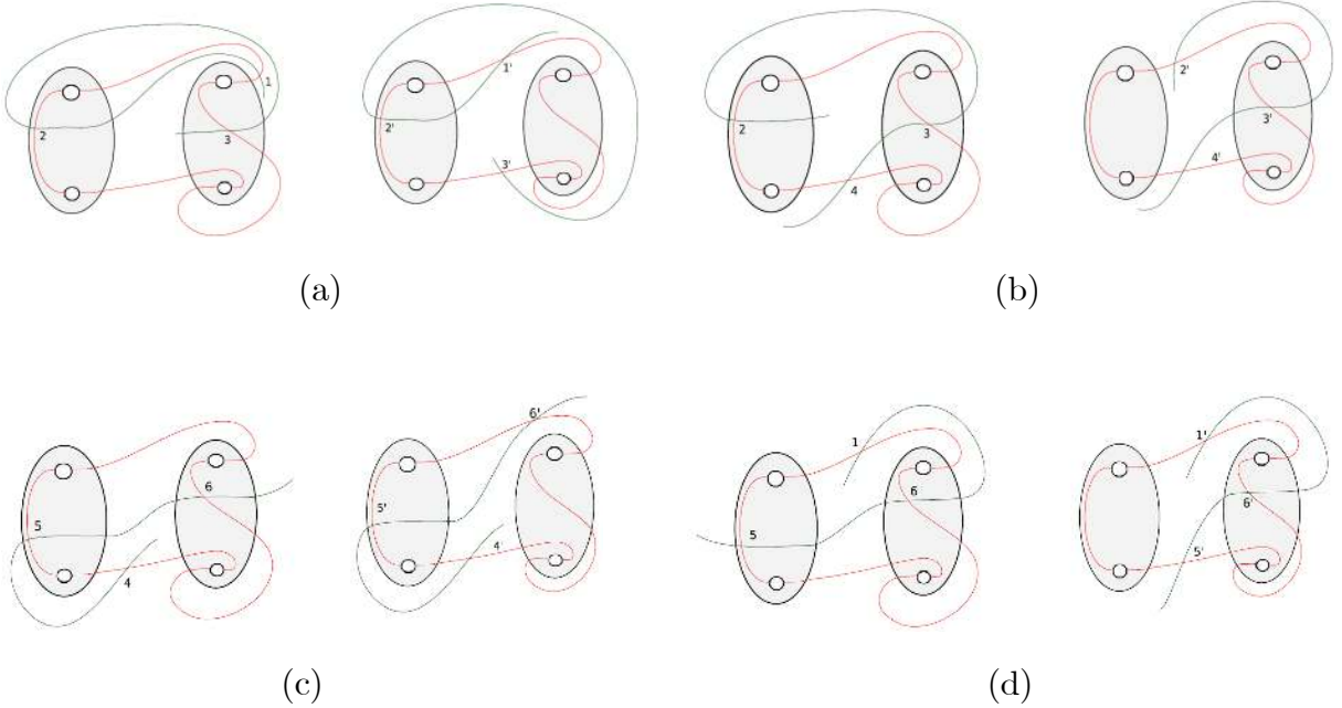
Figure 4.25 Getting a new bypass along a) 1' - 2' - 3' , b) 2' - 3' - 4' , c) 4' - 5' - 6' , d) 5' - 6' - 1' after using bypass rotation when s = 0 .
