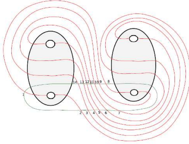
Figure 4.58 A model of the case when n_2 = 4 and s = -7 for \gamma' .
