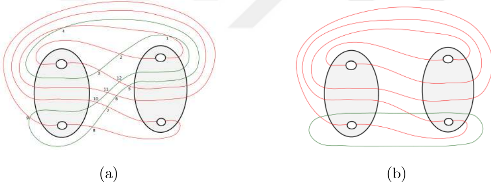
Figure 4.46 a) A model of the case when n_2 = 4 and s = -1 for \gamma , b) A model of the case when n_2 = 4 and s = -1 for \gamma' .
