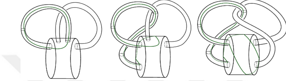
Figure 4.16 H^1 is on the left hand side and the disk D_1^1 in H^1 is bounded by the green curve. H is on the right hand side and the disk D_1 in H is bounded by the green curve.
