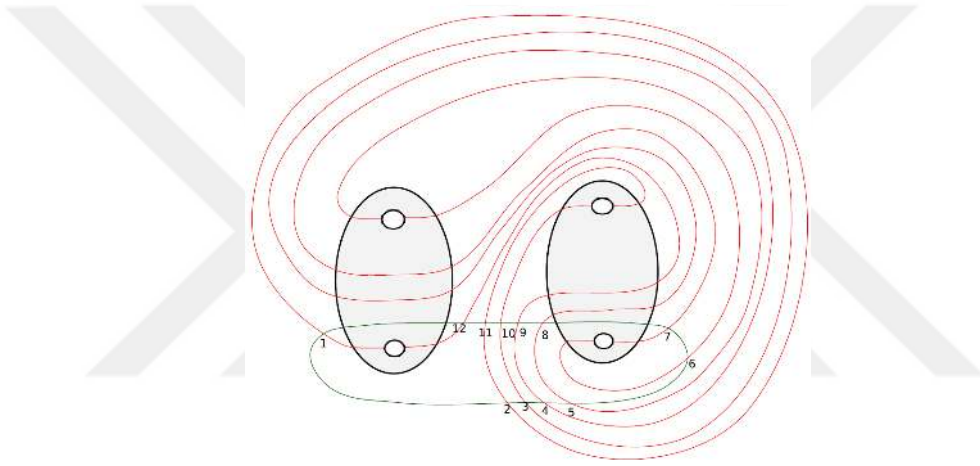
Figure 4.40 A model of the case when n_2 = 4 and s = 5 for \gamma' .
