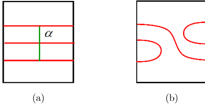
Figure 2.9 Result of a bypass attachment: (a) original surface \Sigma with attaching arc \alpha , (b) the surface \Sigma' = \Sigma \times \{1\} . The dividing curves \Gamma_\Sigma and \Gamma_{\Sigma'} are shown in red.
