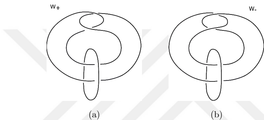
Figure 1.1 a) A Link diagram of the positive Whitehead link (mirror of the Whitehead link), b) A Link diagram of the (negative) Whitehead link.
