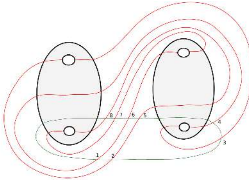
Figure 4.71 A model of the case when n_2 = 3 and s = 4 for \gamma' .
