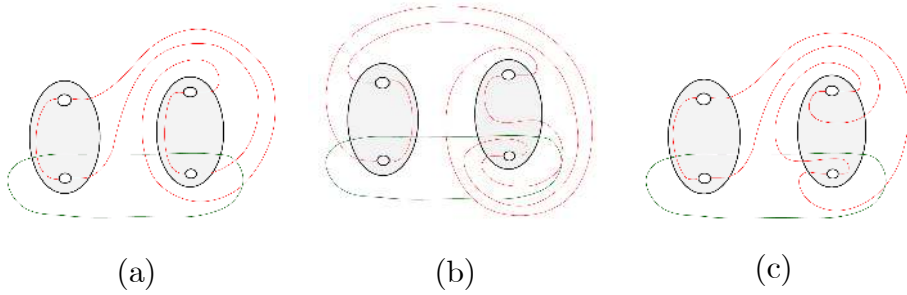
Figure 4.97 a) \Gamma_A after bypass along 2 - 3 - 4 , b) \Gamma_A after bypass along 4 - 5 - 6 , c) \Gamma_A after bypass along 5 - 6 - 7 .
