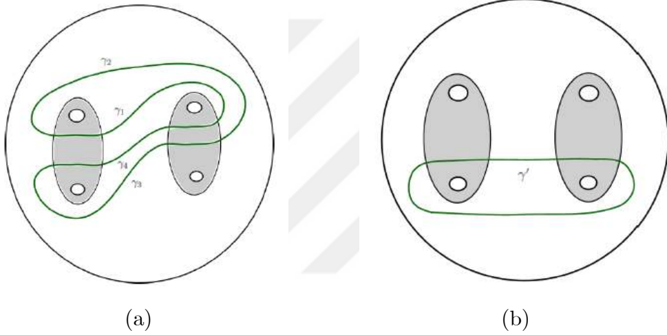
Figure 4.11 a) The curves \gamma_1, \gamma_2, \gamma_3, \gamma_4 obtaining from the intersection of the white annulus A and the green curve \gamma , b) The intersection of the white annulus A and the green curve \gamma' . The 2-sphere S with P'_1 and P'_2 shaded.
