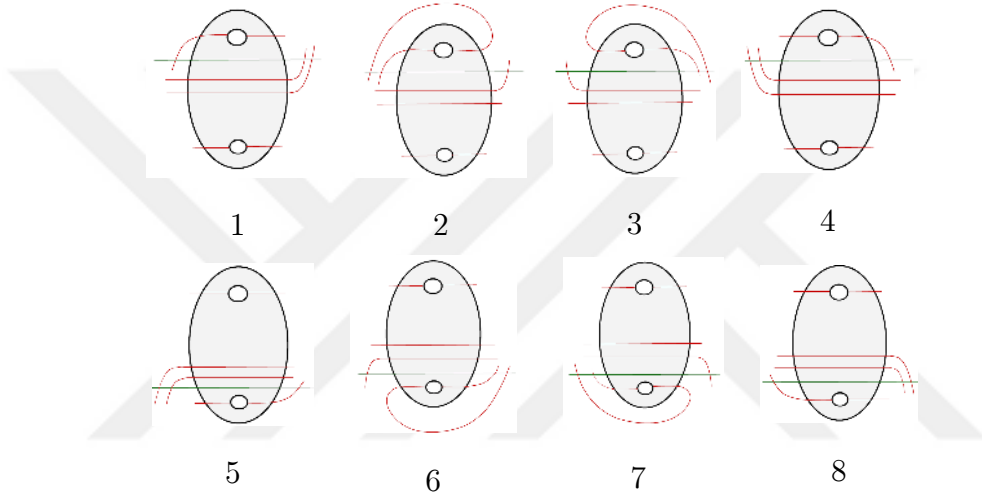
Figure 4.29 The 8 subcases if c \cap (P'_1 \cup P'_2) has one component when n_2 \geq 4 .
