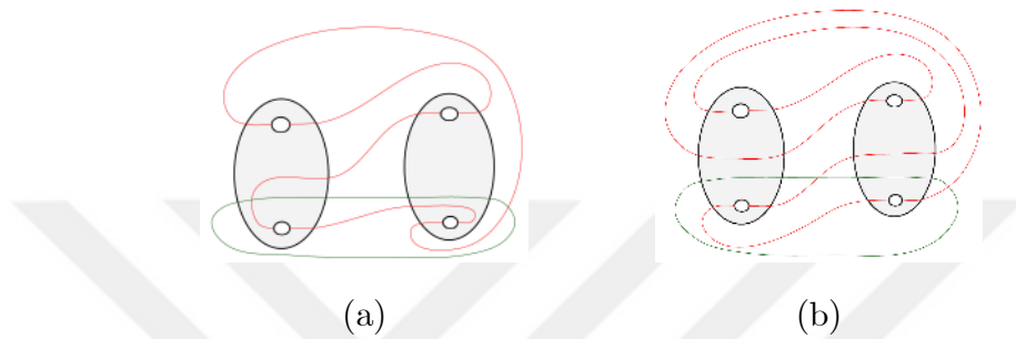
Figure 4.64 a) \Gamma_A after bypass along 2 - 3 - 4 , b) \Gamma_A after bypass along 4 - 1 - 2 .
