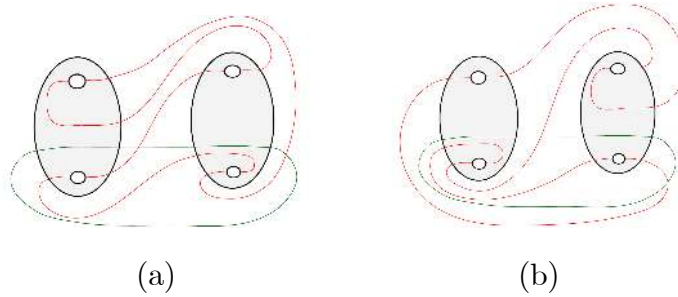
Figure 4.68 a) \Gamma_A after bypass along 1 - 2 - 3 , b) \Gamma_A after bypass along 3 - 4 - 1 .
