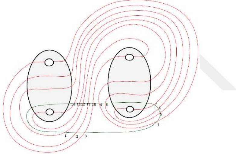
Figure 4.44 A model of the case when n_2 = 4 and s = 7 for \gamma' .
