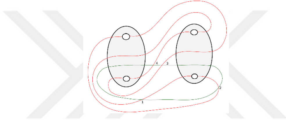
Figure 4.67 A model of the case when n_2 = 3 and s = 2 for \gamma' .
