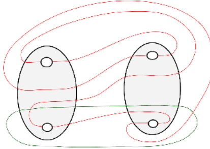
Figure 4.33 \Gamma_A after bypass along the arc 2 - 3 - 4 .
