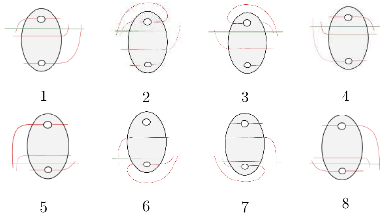
Figure 4.60 The 8 subcases if c \cap (P'_1 \cup P'_2) has one component when n_2 = 3 .
