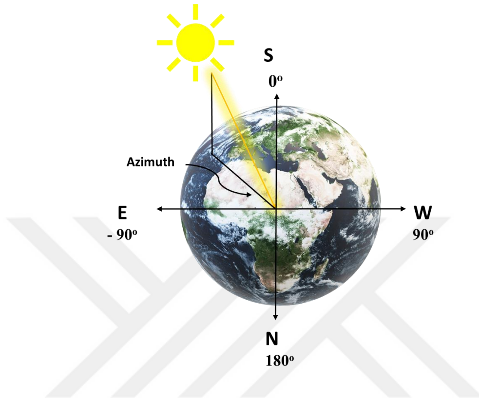
Figure 1.5: Definition of the sun's Azimuth angle
