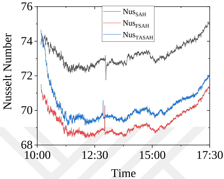
Figure 4.8: Nusselt Number of a flat SAH and SAH having fin.
