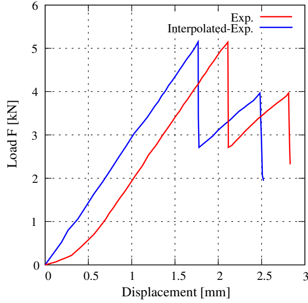
Figure 6.21: Force-displacement curve of [0_5/90_3] test specimen under transverse load and the interpolated experiment curve.
