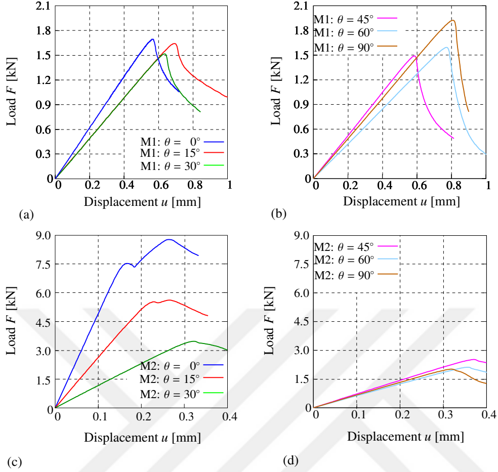
Figure 6.4: Relationships between load F and displacement u for Mode-I (M1) and Mode-II (M2) tests on single edge-notched specimens with various fiber angles, namely \theta = 0^\circ, 15^\circ, 30^\circ, 45^\circ, 60^\circ and 90^\circ : (a),(b) Mode-I; (c),(d) Mode-II.
