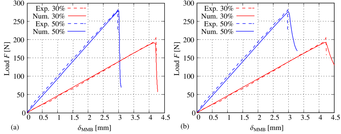
Figure 6.9: Experimental (dashed curves) and numerical (solid curves) results for the relationship between the load F and the loading point displacement \delta_{\text{MMB}} for UD laminates with 30% and 50% MMs: (a) \omega_{f_0} = 1 ; (b) \omega_{f_0} = 30 .
