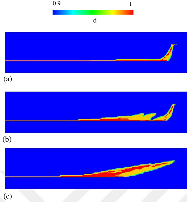
Figure 6.27: Influence of the ratio between \text{ply-}g_c^{\text{iso}} and \text{int-}g_c^{\text{iso}} to the crack path (a) \text{Ply-}g_c^{\text{iso}} = 2.0 , (b) \text{Ply-}g_c^{\text{iso}} = 1.25 , (c) \text{Ply-}g_c^{\text{iso}} = 0.7 .
