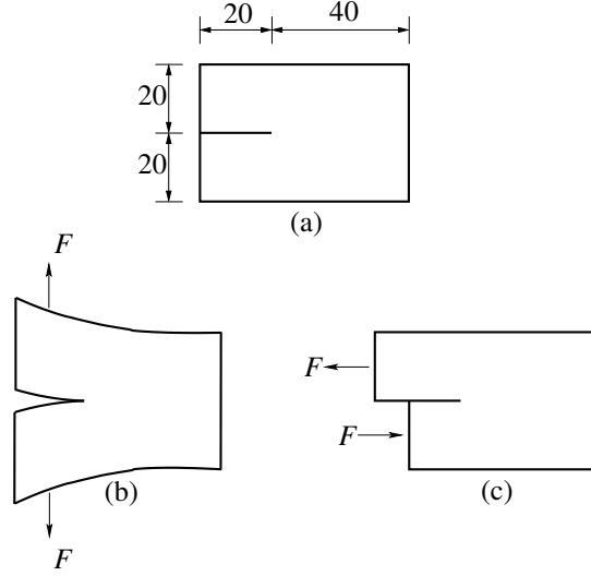
Figure 6.1: Single edge-notched specimen with Mode-I and Mode-II loading: (a) dimensions of the specimen with a notch; (b) Mode-I load case; (c) Mode-II load case. All dimensions are in millimeter.
