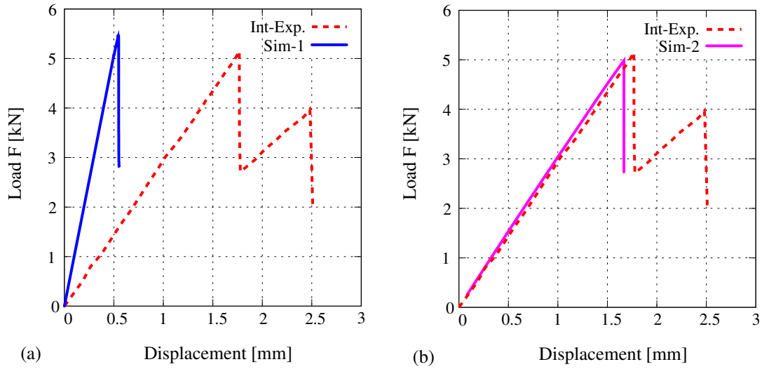
Figure 6.23: Force-displacement curve (a) simulation with fixed boundary conditions, (b) simulation with relaxed boundary conditions.
