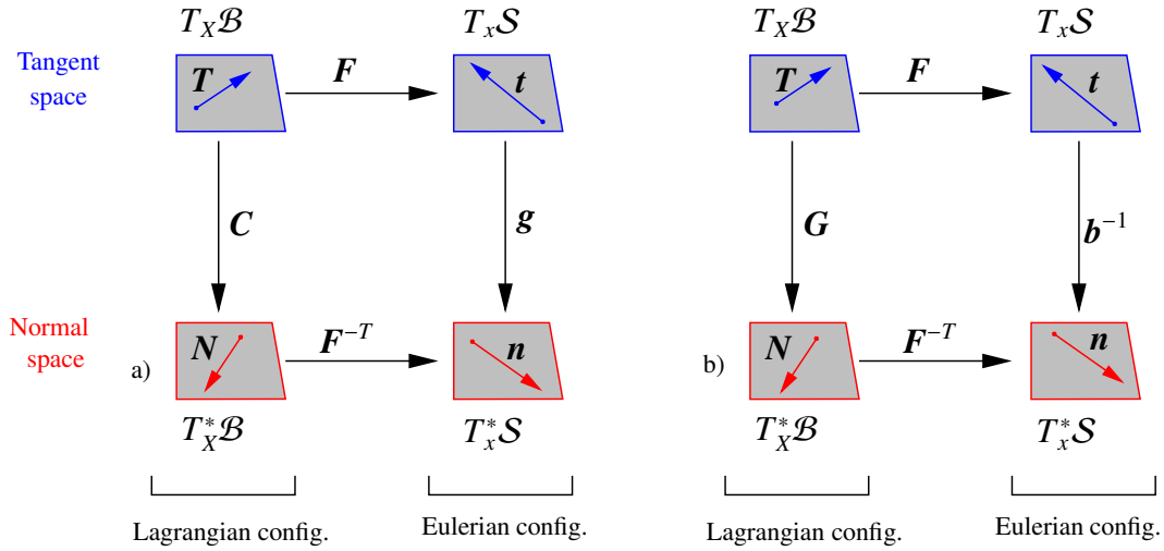
Figure 2.3: Definition of metric tensors. a) current metric in Lagrangian configuration C = F^T g F ; b) reference metric in Eulerian configuration b^{-1} = F^{-T} G F^{-1} .
