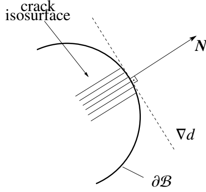
Figure 3.5: Crack isosurface formed perpendicular to the surface for isotropic material.
