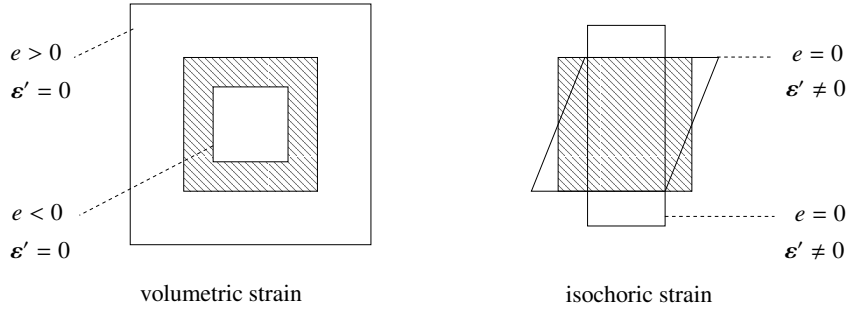
Figure 2.9: Volumetric and isochoric deformations.
