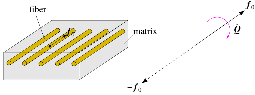
Figure 2.5: Fiber orientation in UD FRP composite with the direction of transverse isotropy \mathbf{f}_0 and rotation tensor \hat{\mathbf{Q}} around \mp \mathbf{f}_0 .
