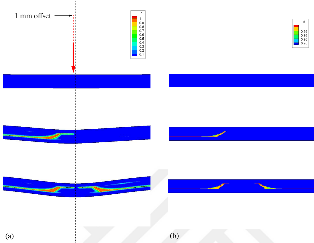
Figure 6.29: Evolution of the crack phase-field d for the asymmetric loading of the beam with 1 mm offset from the centreline. (a) deformed and (b) undeformed configuration .
