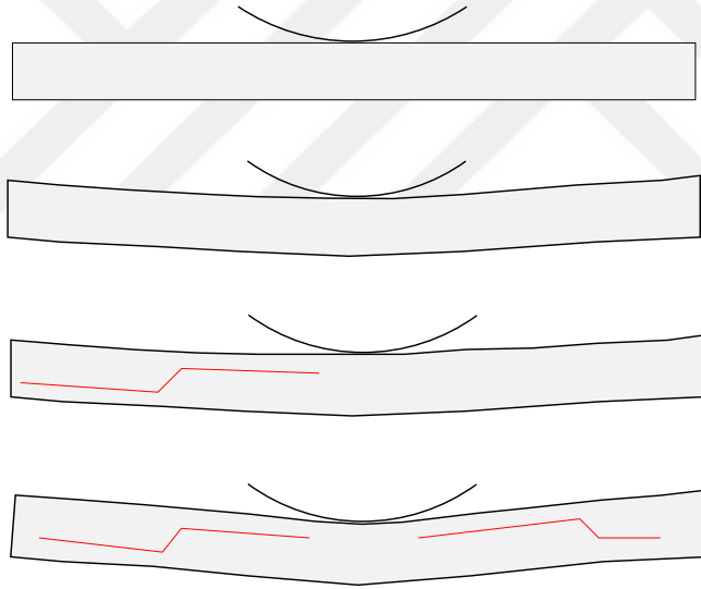
Figure 6.22: Sketch of crack formation in [0_5/90_3] test specimen under transverse load based on the crack images in [10].
