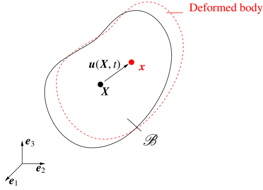
Figure 2.8: Displacement map. The continuum body is denoted as \mathcal{B} and the displacement field is shown as \mathbf{u}(\mathbf{X}, t) .
