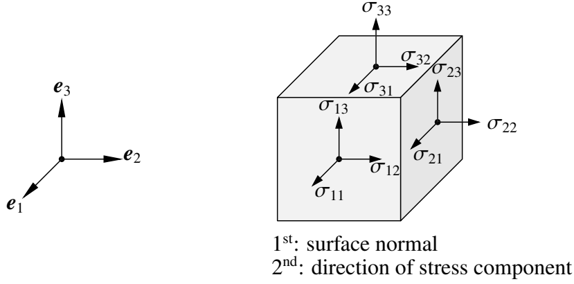
Figure 2.13: Stress components on the surfaces of the cube. The first indice of the stress component indicates the surface normal, second indice defines the direction of the stress component.
