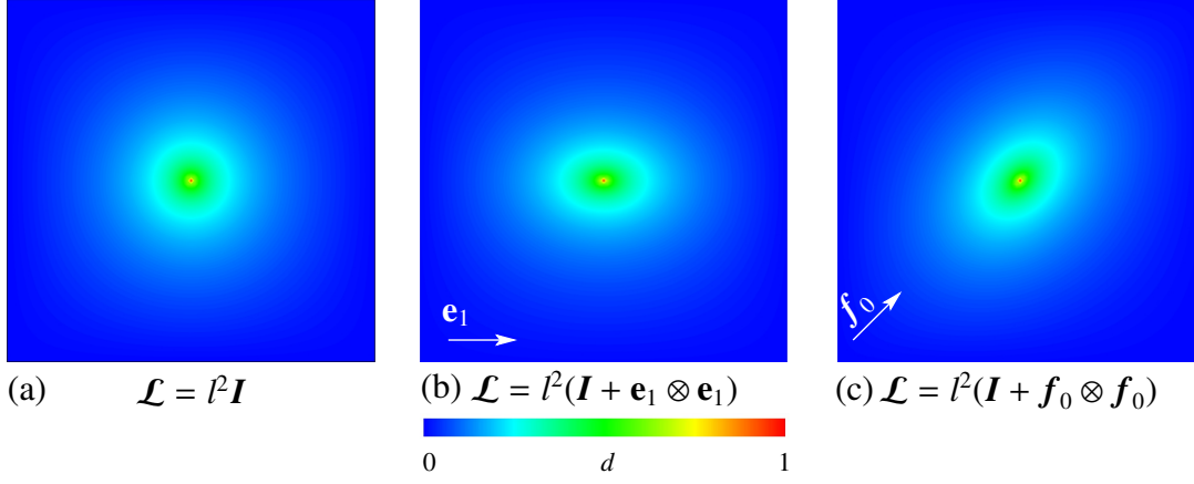
Figure 3.4: Damage field on a square block: (a) isotropic damage field, (b) anisotropic damage field with fiber orientation \theta = 0^\circ stated by the unit base vector \mathbf{e}_1 , (c) anisotropic damage field with fiber orientation \theta = 45^\circ given by the unit vector \mathbf{f}_0 .
