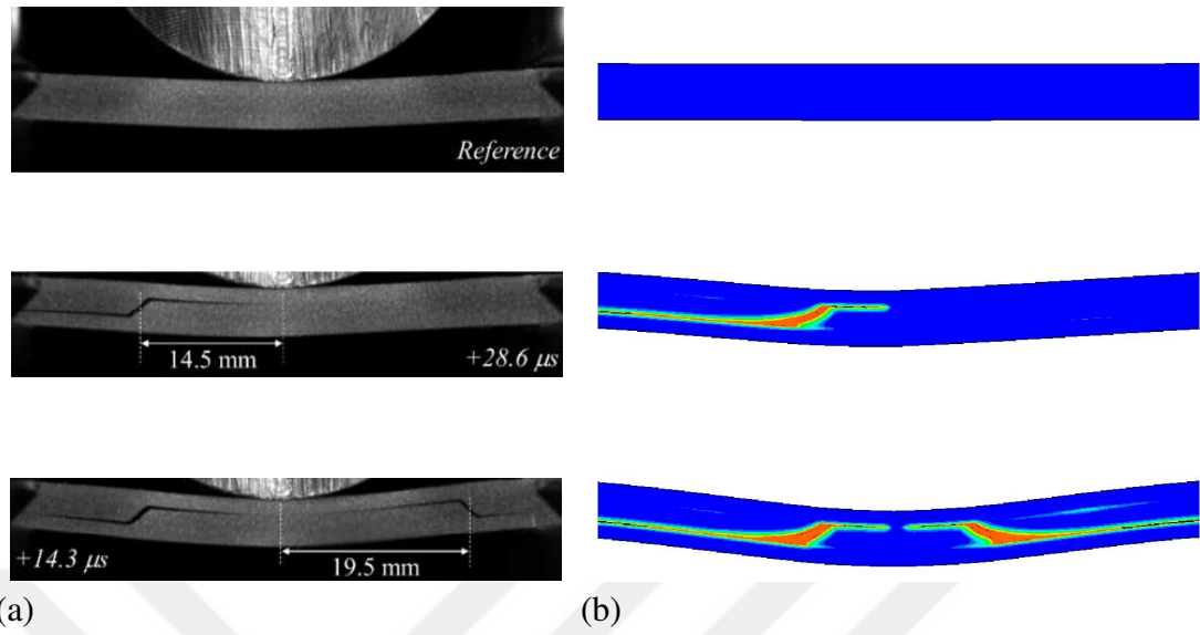
Figure 6.30: Comparison with the real test results (a) test results from Bozkurt [10], (b) analysis results in the deformed configuration.
