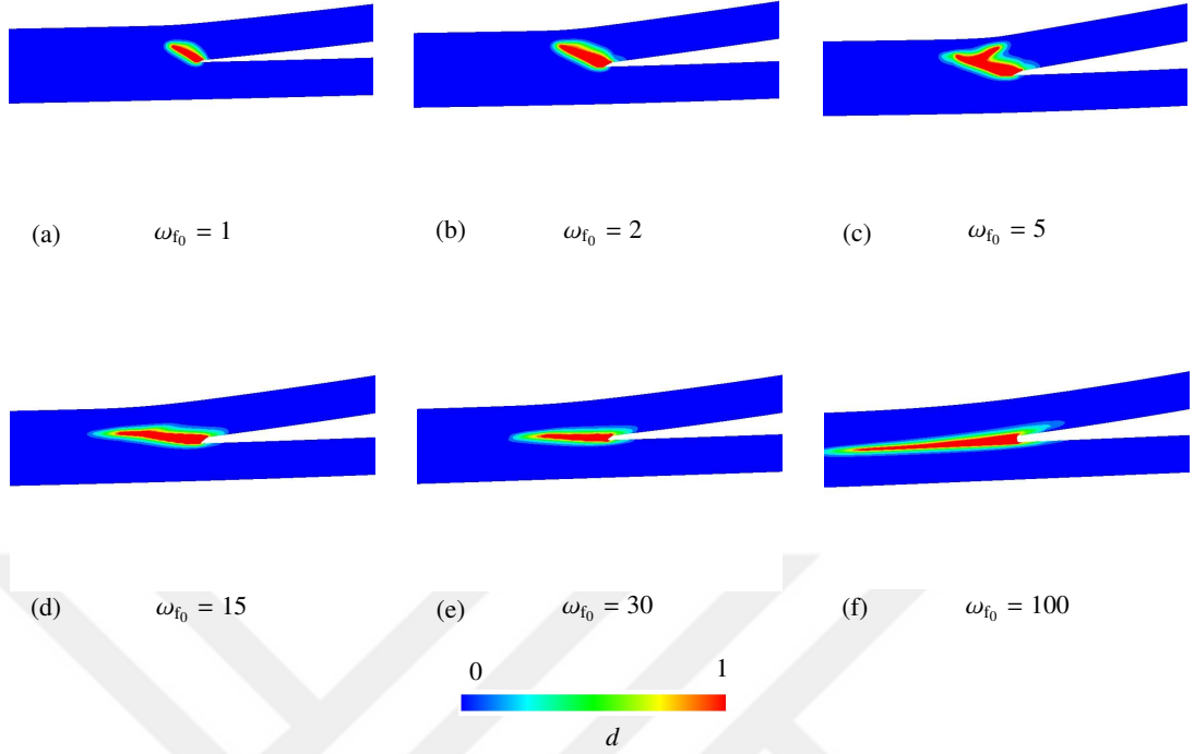
Figure 6.14: Effect of \omega_{f_0} to evolution of the crack phase-field d is examined for the case of mode mixture 30% (a) \omega_{f_0} = 1 ; (b) \omega_{f_0} = 2 , (c) \omega_{f_0} = 5 , (d) \omega_{f_0} = 15 , (e) \omega_{f_0} = 30 , (f) \omega_{f_0} = 100
