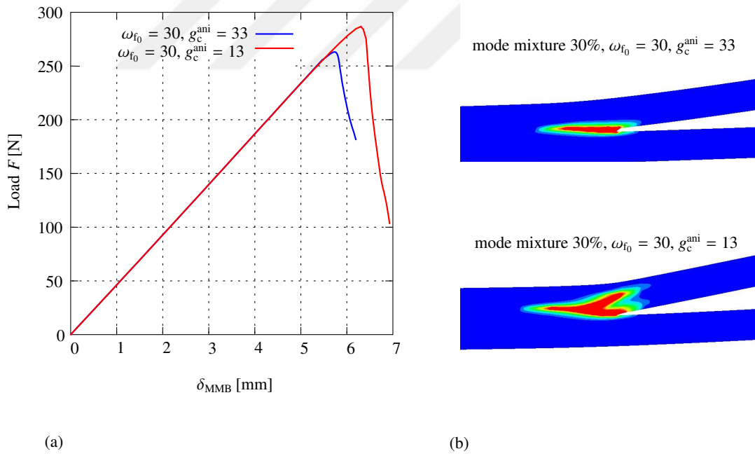
Figure 6.16: Influence of g_c^{\text{ani}} for high anisotropic geometric resistance ( \omega_{f_0} = 30 ) (a) force displacement curves, (b) crack paths.
