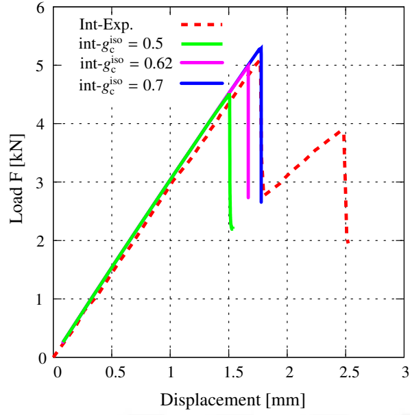
Figure 6.25: Force-displacement curve of [0_5/90_3] beam with relaxed boundary conditions for different \text{int-}g_c^{\text{iso}}
