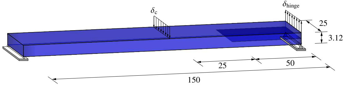
Figure 6.11: Dimensions of the specimen with a 50 mm film placed in the mid-plane serving as a delamination initiator. Also shown are the boundary conditions and displacement at the hinge and the middle of the specimen, i.e. \delta_{\text{hinge}} and \delta_c . All dimensions are in millimeters.
