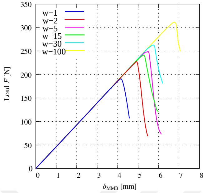
Figure 6.15: Influence of anisotropy parameter \omega_{f_0} on force–displacement response. MMB case for mode mixture 30% is performed with respect to different anisotropy parameters.
