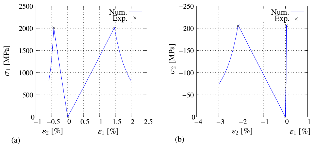
Figure 6.19: Numerical prediction versus experimental data for an Hexcel/3501-6 epoxy lamina (a) tension in the fiber direction; (b) compression in the transverse to fiber direction.
