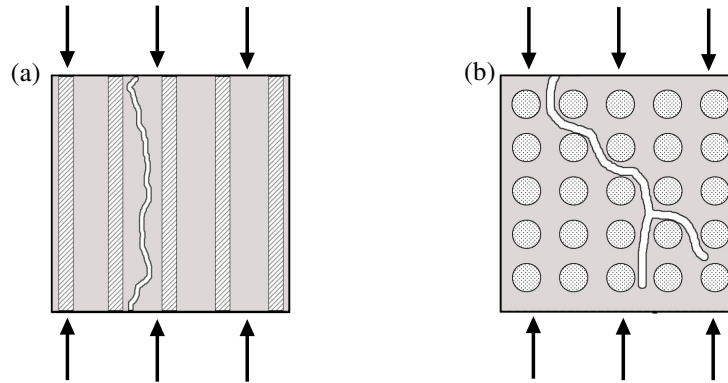
Figure 1.3: Shear failure (a) in longitudinal compression and (b) in transverse compression
