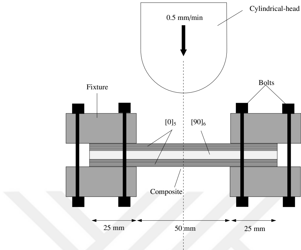
Figure 6.18: Geometrical sketch of the real fixture and the test specimen given in Bozkurt et al. [10].
