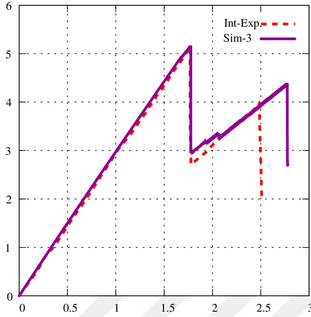
Figure 6.28: [0_5/90_3] beam test data and the corresponding analysis result with relaxed boundary conditions and updated material parameters.
