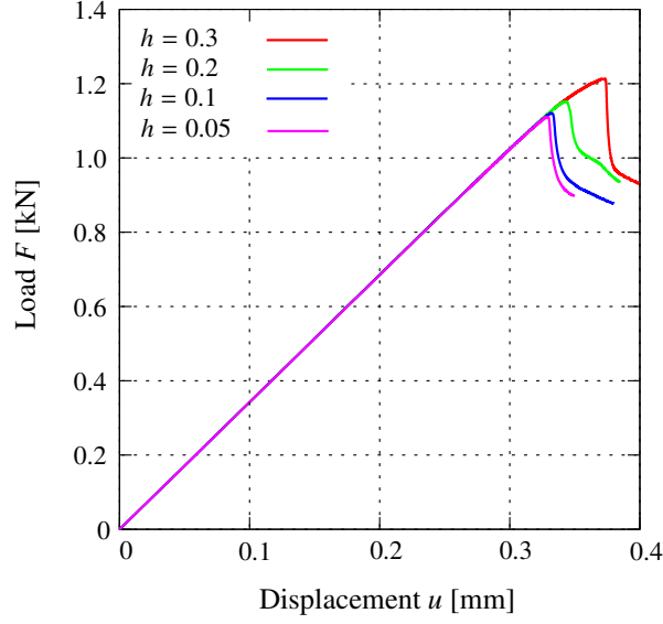
Figure 6.5: Load–displacement curves for different mesh sizes
