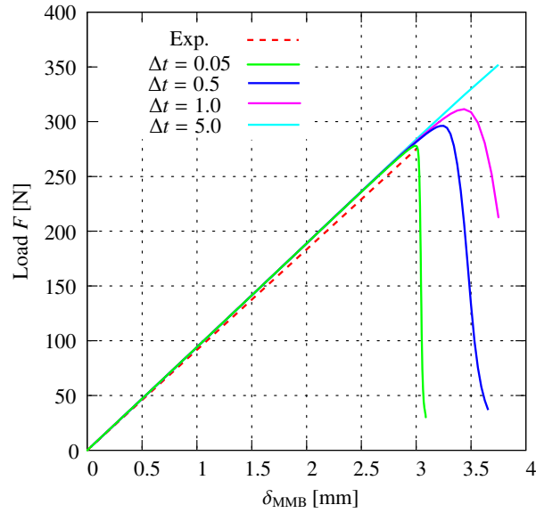
Figure 6.12: Force-displacement curve with respect to large and small time increments, and the influence of \Delta t on the crack initiation.
