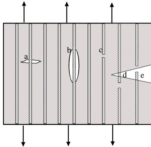
Figure 1.1: Possible micro-failure modes in longitudinal tension; a) matrix-crack, b) matrix-debonding, c) fiber-cracture, d) bridging e) fiber-pull-out
