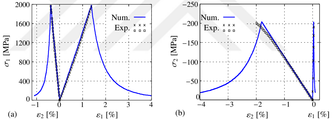
Figure 6.2: Numerical prediction versus experimental data for an AS4/3501-6 epoxy lamina – stress \sigma versus strain \varepsilon in the 1 (horizontal) and 2 (vertical) direction: (a) tension in the 1 direction; (b) compression in the 2 direction.
