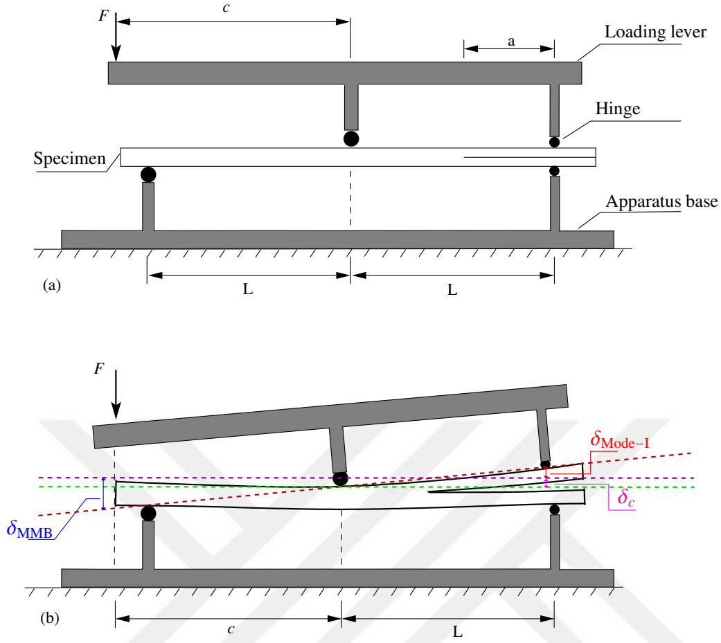
Figure 6.6: (a) Geometrical sketch of the MMB testing device with the specimen in the undeformed configuration; (b) in the deformed configuration with the corresponding displacements (reconstructed from Crews & Reeder [14]).
