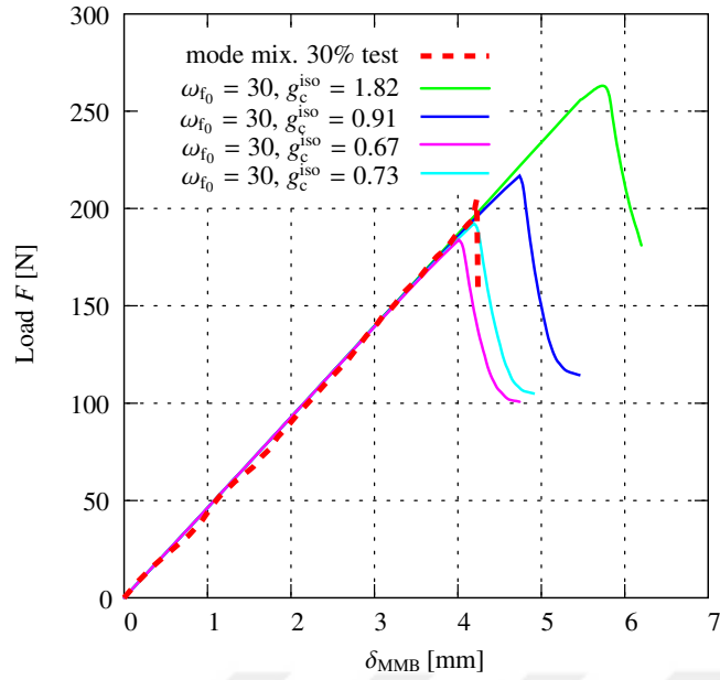
Figure 6.17: Influence of g_c^{\text{iso}} on failure load for high anisotropic geometric resistance ( \omega_{f_0} = 30 ).
