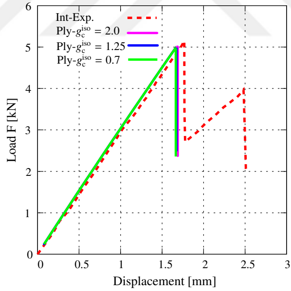
Figure 6.26: Force-displacement curve of [0_5/90_3] beam with relaxed boundary conditions for different \text{ply-}g_c^{\text{iso}}
