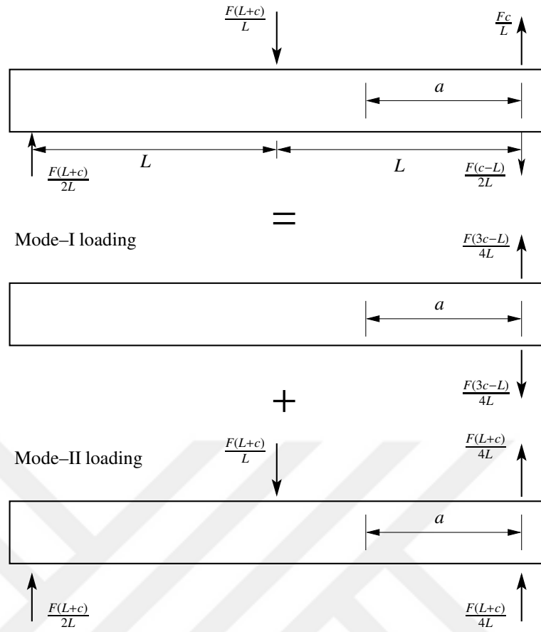
Figure 6.7: Illustration of loading of the MMB test specimen decomposed according to Mode-I and Mode-II cases (reconstructed from Crews & Reeder [14]).
