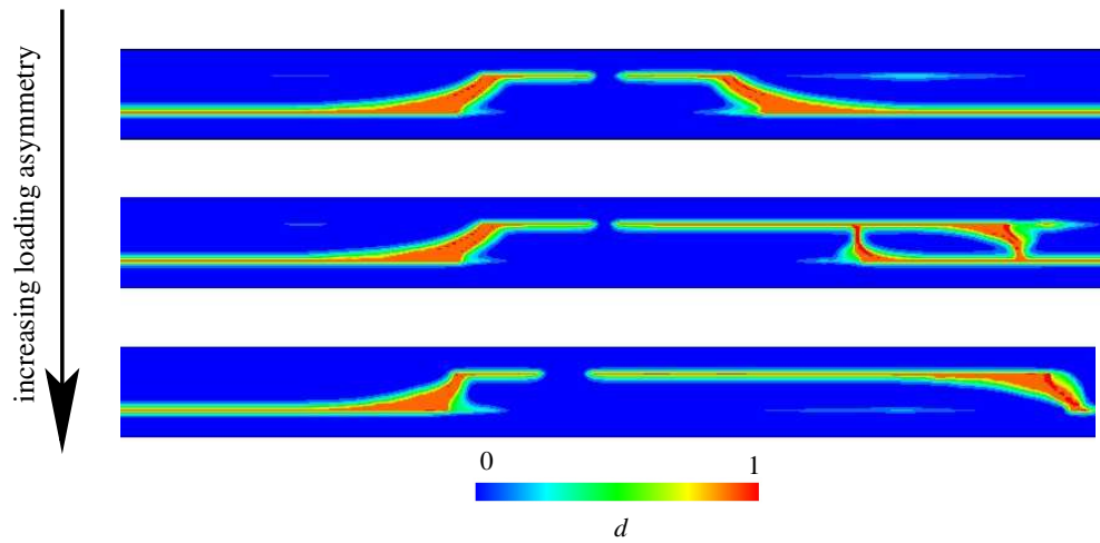
Figure 6.31: Evolution of the diagonal crack in relation with the increasing asymmetric loading.
