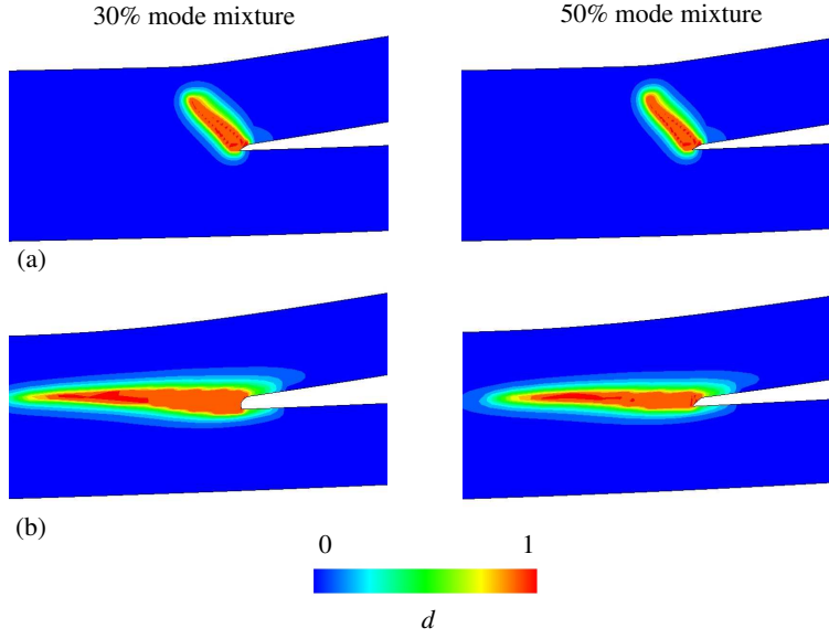
Figure 6.13: Evolution of the crack phase-field d with respect to the mode mixture of 30% (left panels) and 50% (right panels) for two anisotropy parameters: (a) \omega_{f_0} = 1 ; (b) \omega_{f_0} = 30 .
