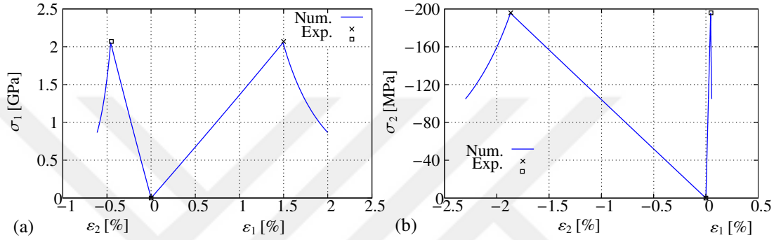
Figure 6.10: Numerical prediction versus experimental data for an APC2 lamina – stress \sigma versus strain \epsilon in the 1 (horizontal) and 2 (vertical) direction: (a) tension in the 1 direction; (b) compression in the 2 direction.
