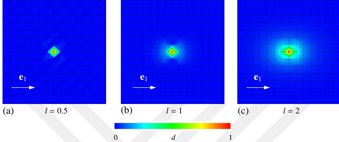
Figure 3.6: Damage field on a 14 \times 14 square block with a single fiber family with d = 1 in the middle point and element size h = 1 : (a) l = 0.5 , (b) l = 1 and for (c) l = 2 , along with w_{f_0} = 1 for all three cases .
