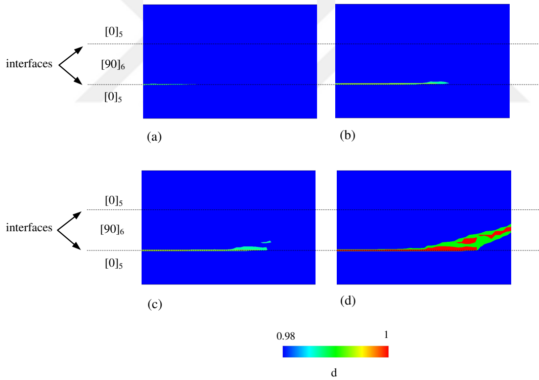
Figure 6.24: Evolution of the crack ( d=1 ) in a sequence (a), (b), (c), (d)
