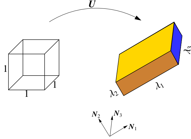
Figure 2.4: Deformation of unit volume element
