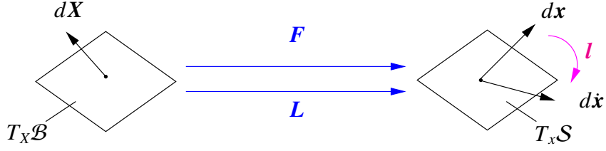
Figure 2.6: Material and spatial velocity gradient mapping.
