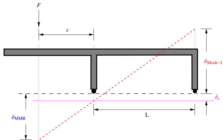
Figure 6.8: Displacements of the loading arm [42].
