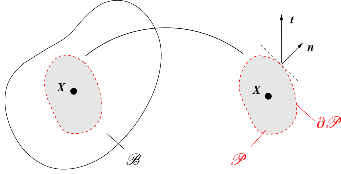
Figure 2.12: Left-hand side is the body \mathcal{B} , right-hand side is the cut-out part \mathcal{P} \subset \mathcal{B} of the body. The surface of the cut-out part is denoted as \partial\mathcal{P} .
