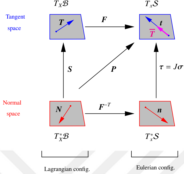
Figure 2.11: Definition of stress tensors and traction vectors in large strain.
