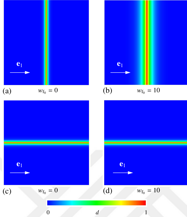
Figure 3.8: Damage field on a square block with a single fiber family whose orientation is characterized by the unit base vector \mathbf{e}_1 : (a),(b) for a vertical centroidal crack; (c),(d) for a centroidal horizontal crack where w_{f_0} = 0 in the first column and w_{f_0} = 10 in the second column.
