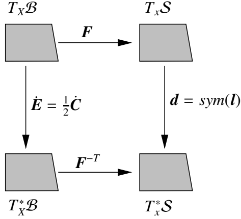
Figure 2.7: Rates of deformation and strain measures.
