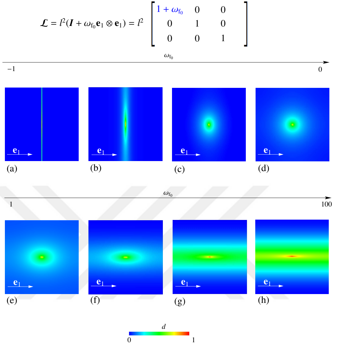
Figure 3.7: Damage field on a 100 \times 100 square block: (a) \omega_{f_0} = -1 , (b) \omega_{f_0} = -0.99 , (c) \omega_{f_0} = -0.5 , (d) \omega_{f_0} = 0 , (e) \omega_{f_0} = 1 , (f) \omega_{f_0} = 5 , (g) \omega_{f_0} = 30 , (h) \omega_{f_0} = 100 , with fiber orientation \theta = 0^\circ stated by the unit base vector \mathbf{e}_1 , h = 1 and, length scale parameter l = 60 .
