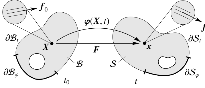
Figure 3.1: Nonlinear deformation of a solid. The reference configuration \mathcal{B} \in \mathbb{R}^3 and the spatial configuration \mathcal{S} \in \mathbb{R}^3 ; \varphi : \mathcal{B} \times \mathbb{R} \mapsto \mathbb{R}^3 is the nonlinear deformation map which maps the material point position X \in \mathcal{B} onto the spatial position \mathbf{x} = \varphi(X, t) \in \mathcal{S} , at time t \in \mathbb{R}_t .
