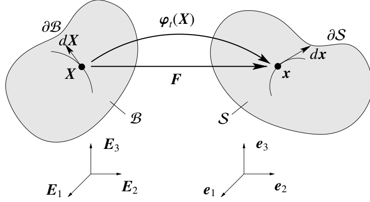
Figure 2.1: Left-hand side is the (undeformed) reference configuration \mathcal{B} with a boundary description \partial\mathcal{B} , right-hand side is the deformed configuration \mathcal{S} with a boundary \partial\mathcal{S} as a result of deformation \varphi .
