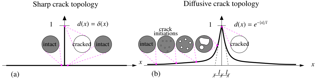
Figure 3.3: Sharp and regularized crack topology. (a) Sharp crack at x = 0 modelled by Kronecker delta function d(x) = \delta(x) , (b) regularized crack topology at x = 0 described by d(x) = e^{-|x|/l} with a length scale parameter l which controls the breadth of crack .
