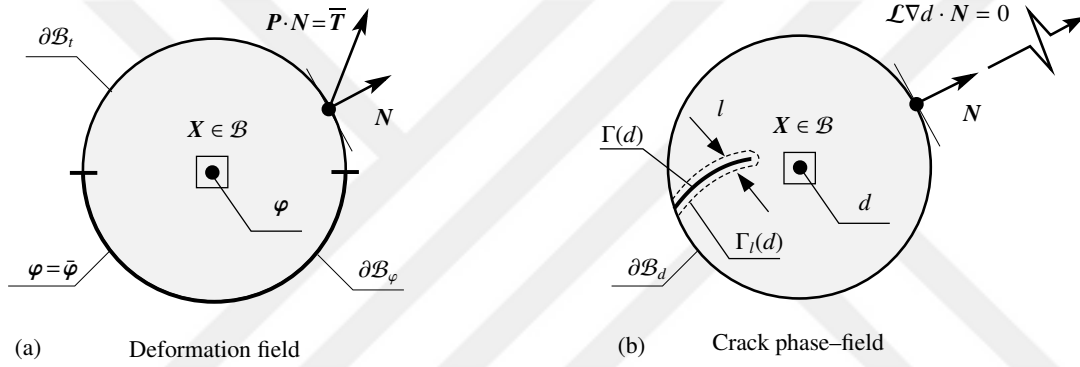
Figure 3.2: Multi-field problem: (a) mechanical problem of deformation along with Dirichlet and Neumann-type boundary conditions, that is \varphi = \bar{\varphi} and \mathbf{P} \cdot \mathbf{N} = \bar{\mathbf{T}} , respectively; (b) evolution of the crack phase-field problem with the Neumann-type boundary condition \mathcal{L} \nabla d \cdot \mathbf{N} = 0 .
