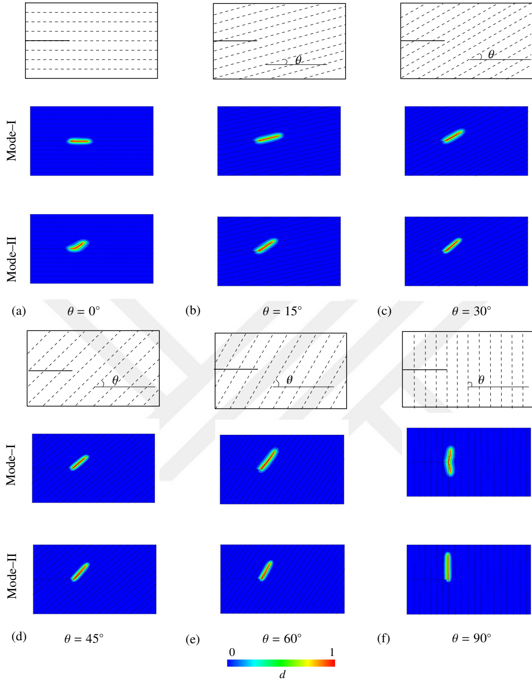
Figure 6.3: Evolution of the crack phase-field d for Mode-I and Mode-II tests in single edge-notched specimens with different fiber angles \theta : (a) \theta = 0^\circ ; (b) \theta = 15^\circ ; (c) \theta = 30^\circ ; (d) \theta = 45^\circ ; (e) \theta = 60^\circ ; (f) \theta = 90^\circ .
