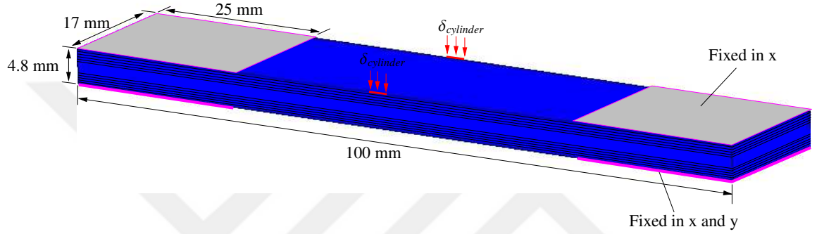
Figure 6.20: Test specimen dimensions and boundary conditions.
