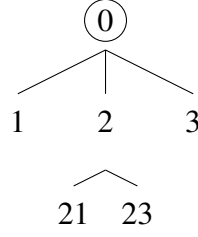
Figure 3.1: A rooted tree
