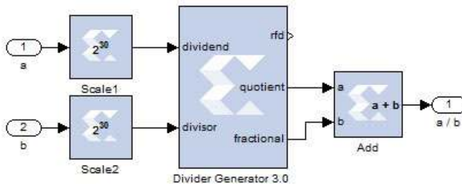
Figure 4.7: Divider Block
