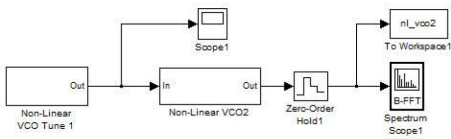
Figure 5.16: Nonlinear Input Sweep of Nonlinear VCO
