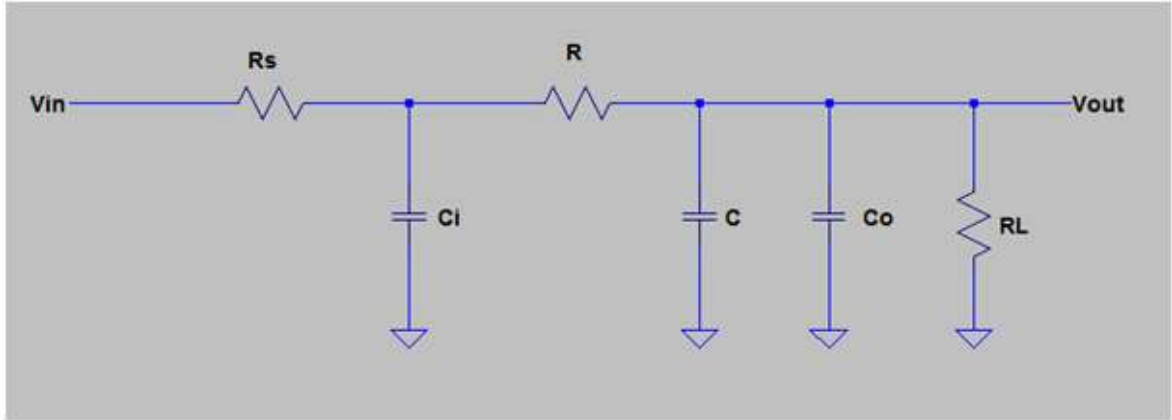
Figure C.1: Original Circuit
