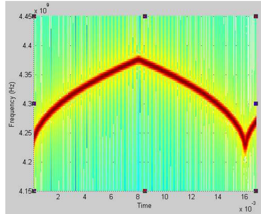
Figure 5.12: Output Spectrogram of VCO for Simulation shown in Figure 5.10
