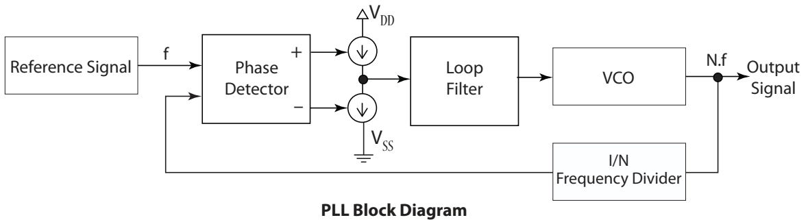
Figure 2.2: Typical Charge-Pump PLL Block Diagram
