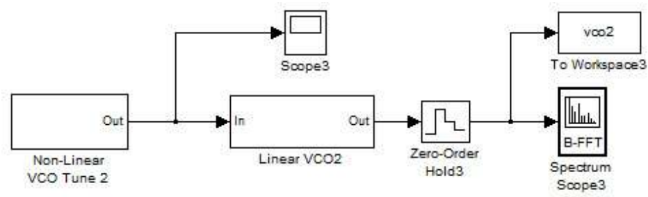
Figure 5.13: Nonlinear Input Sweep of Linear VCO
