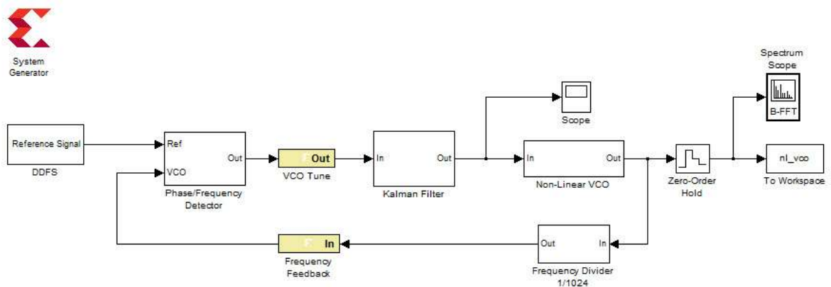
Figure 5.21: System Block Diagram of Partial Controller Implementation
