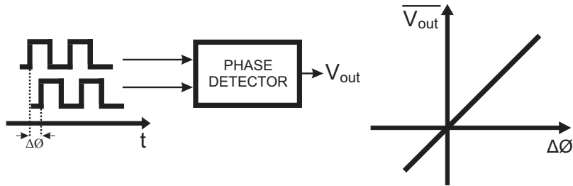
Figure D.2: Characteristic of an Ideal Phase Detector
