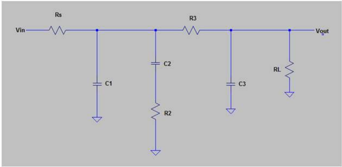
Figure C.3: Original Circuit
