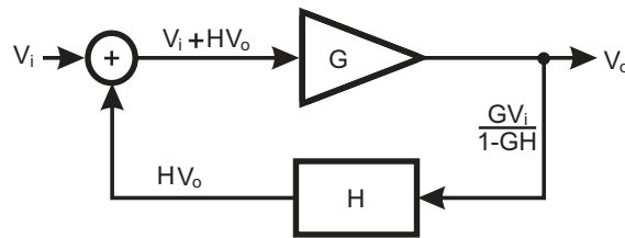
Figure 2.7: VCO Model
