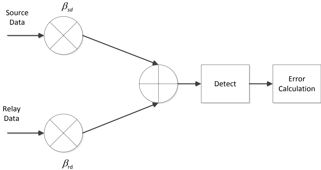
Figure 4. 9 Destination model
