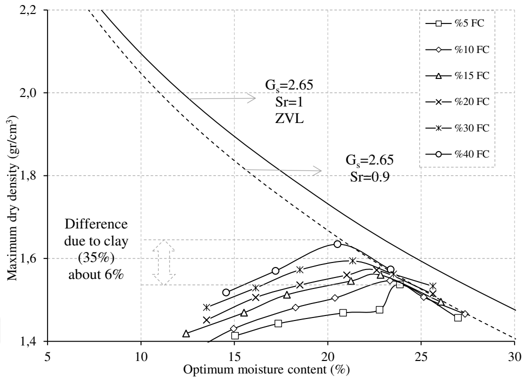
Figure 4.3 Variation of OMC with MDD for the clay with 0.15-0.30 mm CSS
