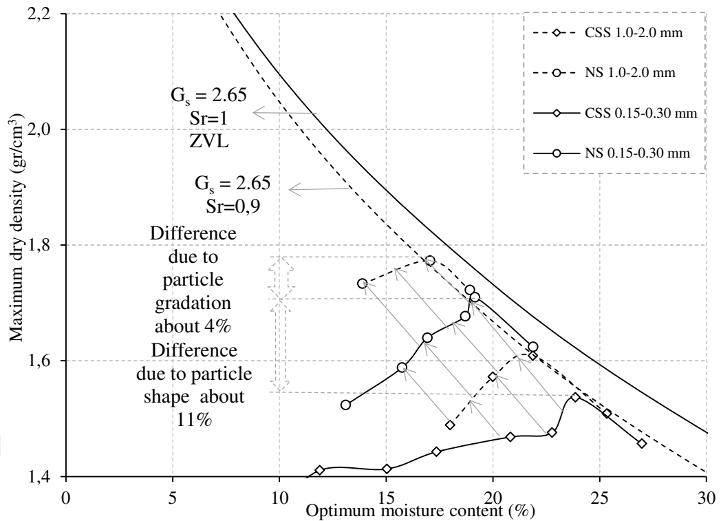
Figure 4.5 Variation of OMC with MDD for %5 the fines with different sand
