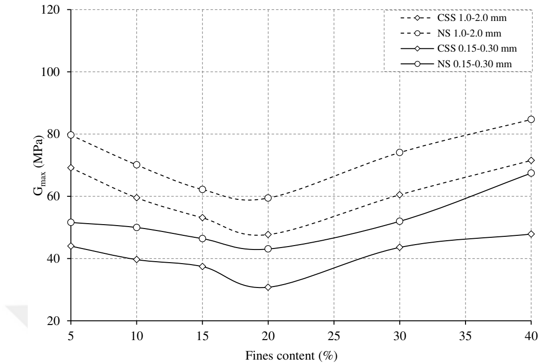
Figure 4.21 Variation of fines content with G_{\max} for 17 frequency with different mixtures
