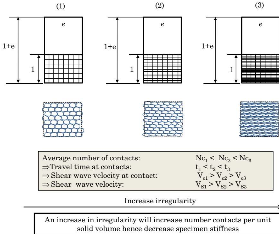
Figure 4.24 Hypothesis for the effect of particle shape on G_{\max} (Bui, 2007)
