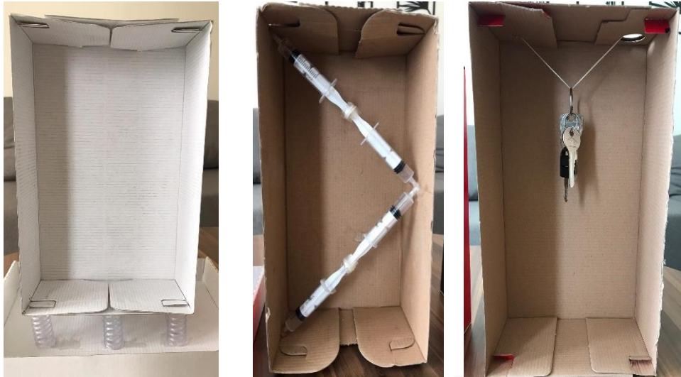
Figure 4.30. The teacher's products with the base isolation, the seismic damper and the tuned mass damper technologies
