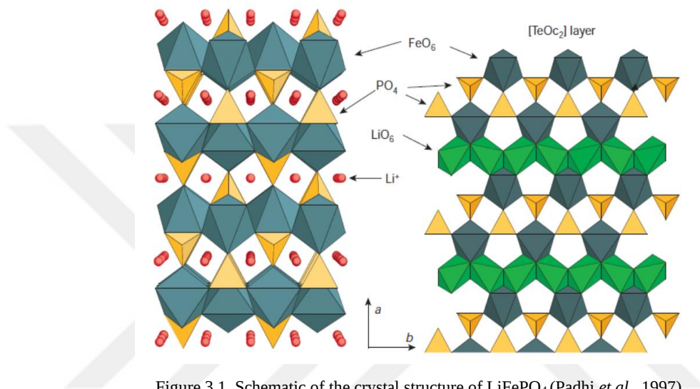
Figure 3.1. Schematic of the crystal structure of \text{LiFePO}_4 (Padhi et al. , 1997).
