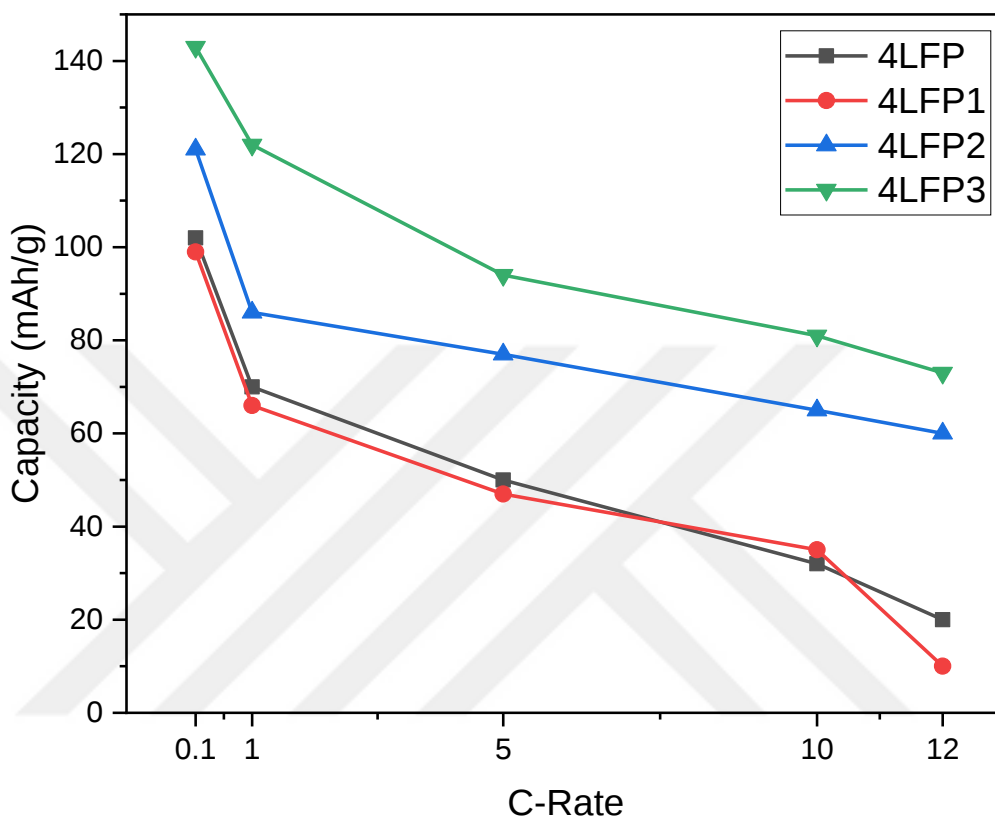
Figure 5.11. The discharge capacity of the \text{LiFePO}_4/\text{C} samples was compared based on the various sucrose introduction methods (4LFP1, 4LFP2, and 4LFP3).
