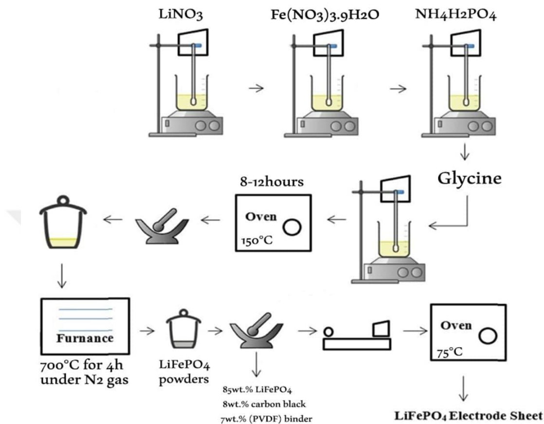
Figure 4.1. Flow diagrams of LiFePO 4 powder products.
