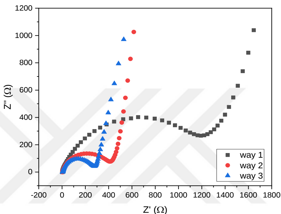
Figure 5.12. A variety of sucrose introduction methods were used to obtain EIS of \text{LiFePO}_4 electrodes.
