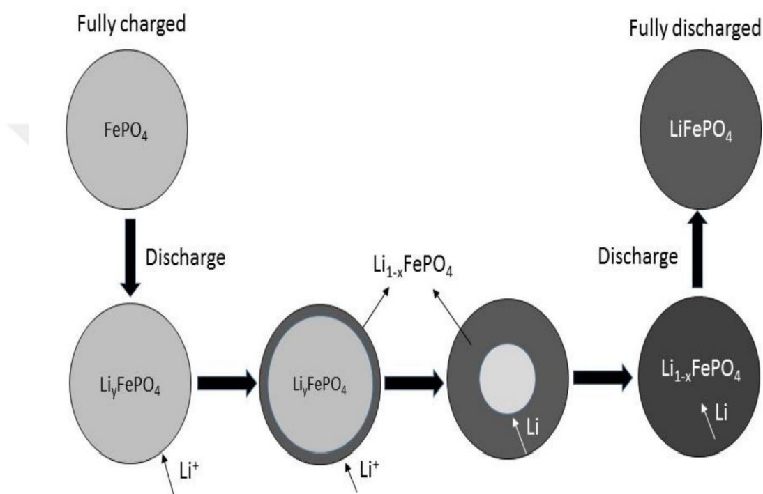
Figure 3.2. \text{Li}^+ insertion process (discharge process).
