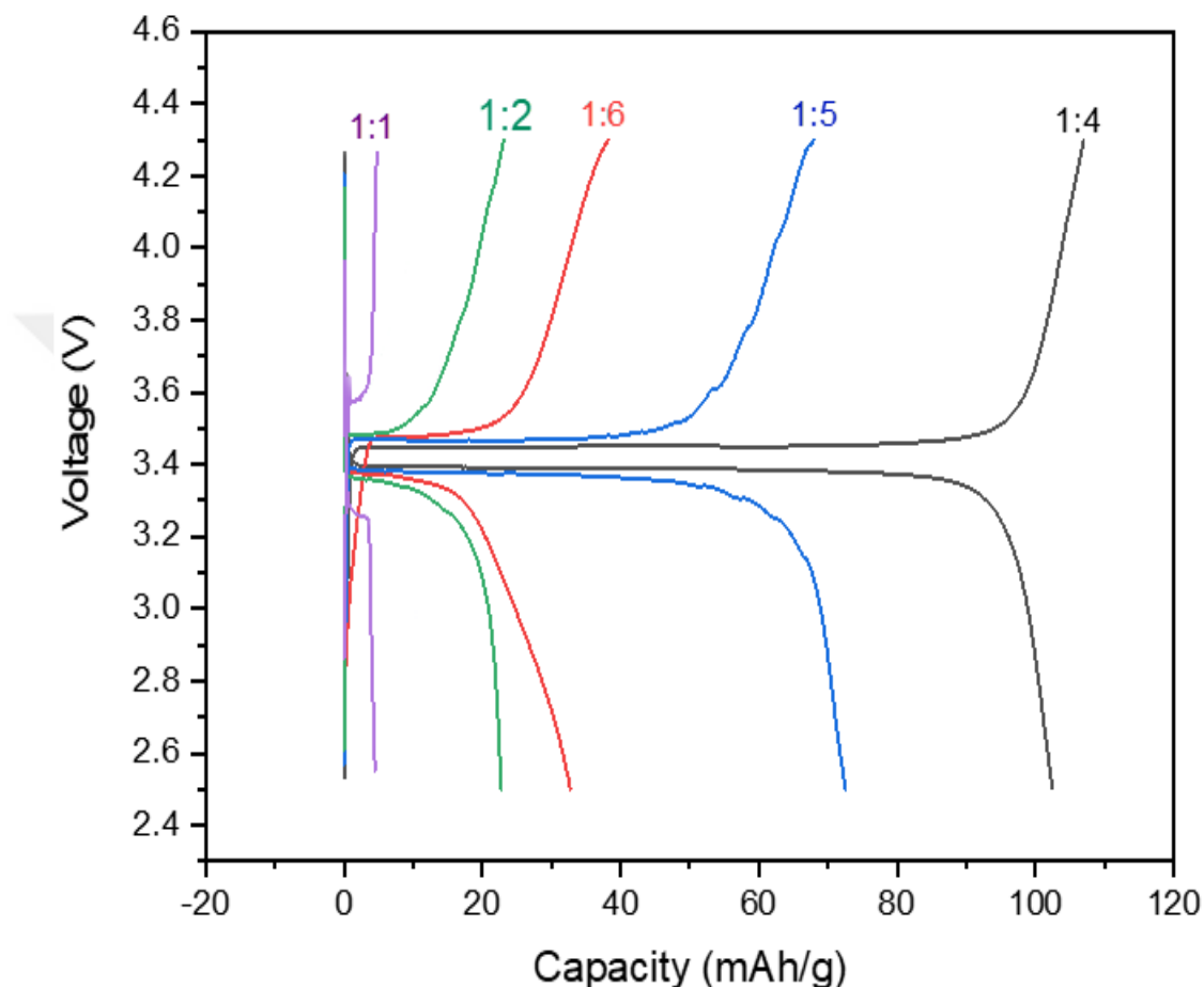
Figure 5.5. The voltage profiles for the first cycle charging and discharging (with a rate of 0.1 C) for different \text{LiFePO}_4 samples synthesized with varied glycine concentrations at a 0.1C rate.
