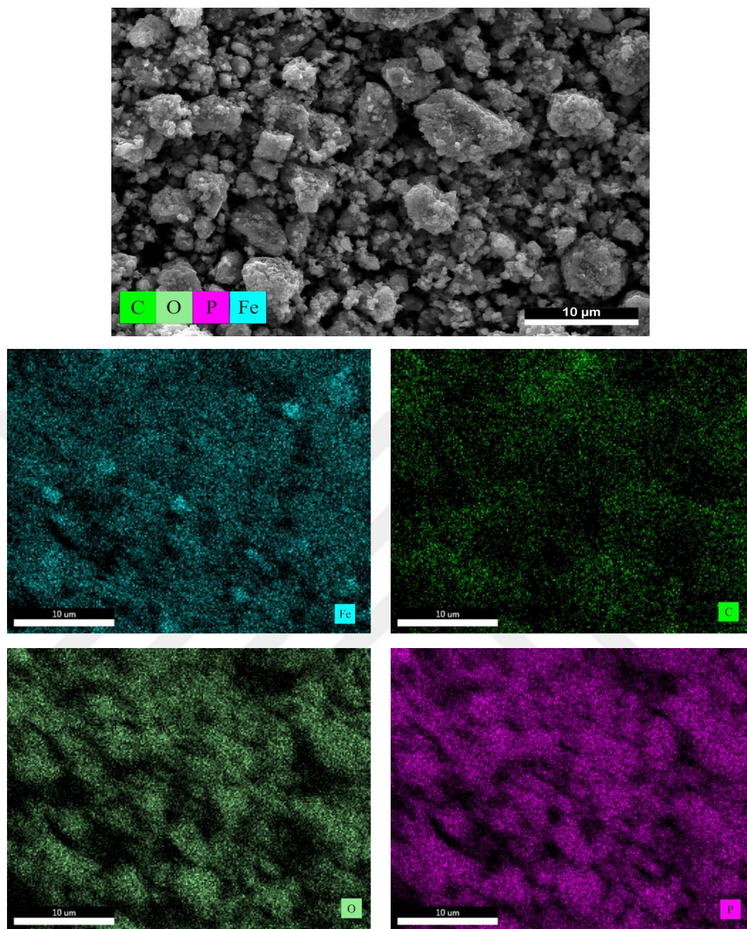
Figure 5.10. EDS mapping images of \text{LiFePO}_4/\text{C} .
