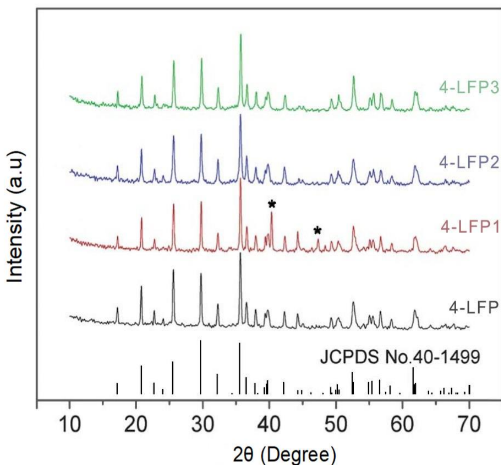
Figure 5.8. \text{LiFePO}_4 XRD patterns, produced by multiple sucrose introduction methods (*: \text{Fe}_2\text{P} ) for four different samples (4LFP, 4LFP1, 4LFP2 and 4LFP3)(*: \text{Fe}_2\text{P} ).
