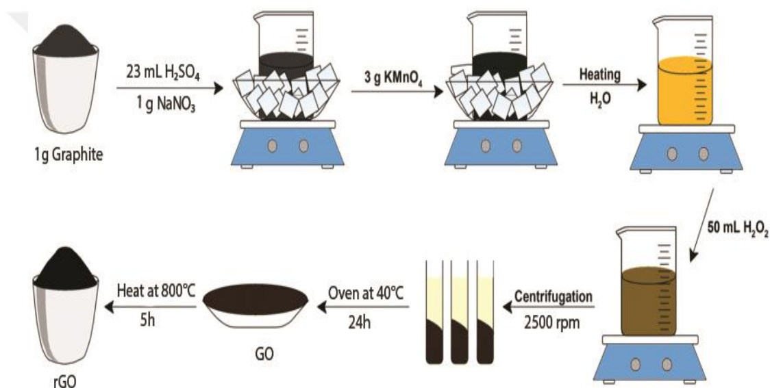
Figure 4.3. The schematic diagram of sample preparation process.
