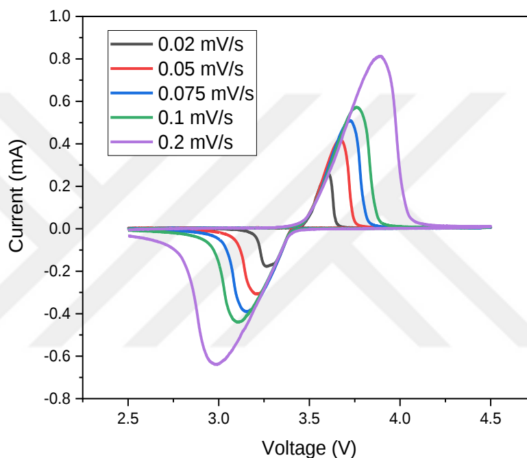
Figure 5.15. Cyclic voltammetry curves of LiFePO 4 /C sample at various scan rates (from inner to outer: 0.02, 0.05, 0.075, 0.1, 0.2 mV/s).
