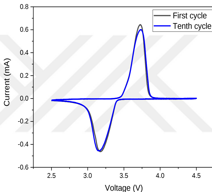
Figure 5.14. Cyclic voltammetry curves of \text{LiFePO}_4/\text{C} sample produced in way 3 first and tenth cycles at 0.1 mV/s.
