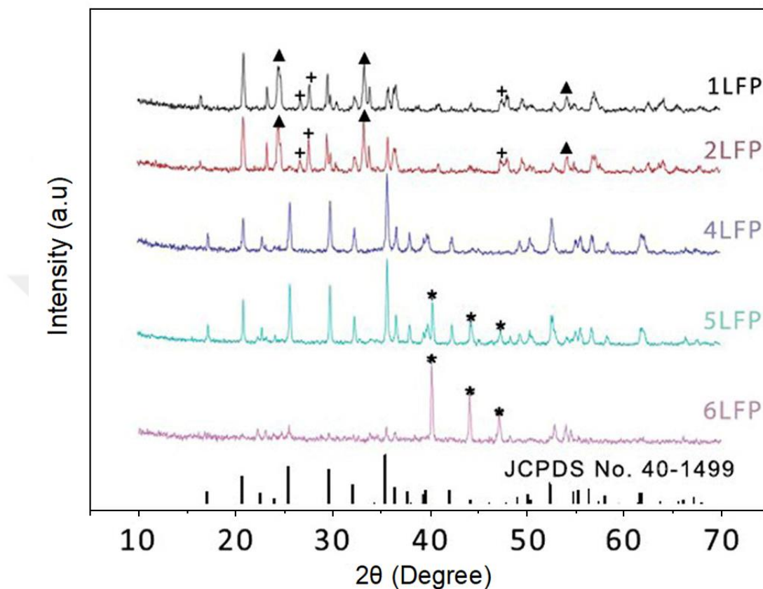
Figure 5.2. The XRD patterns of \text{LiFePO}_4 powders synthesized with various quantities of glycine ( ▲: \text{Fe}_2\text{O}_3 , +: \text{Li}_3\text{Fe}_2(\text{PO}_4)_3 ; *: \text{Fe}_2\text{P} ).
