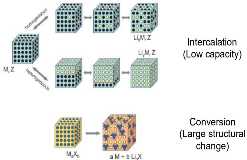
Figure 2.1. Electrochemical energy storage: intercalation and conversion reactions (Palacin, 2009).
