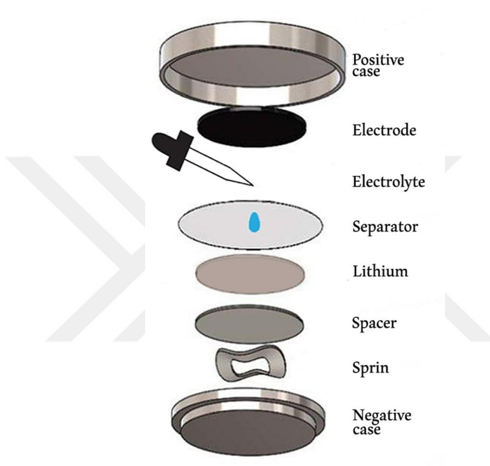
Figure 4.7. Coin cell configurations.
