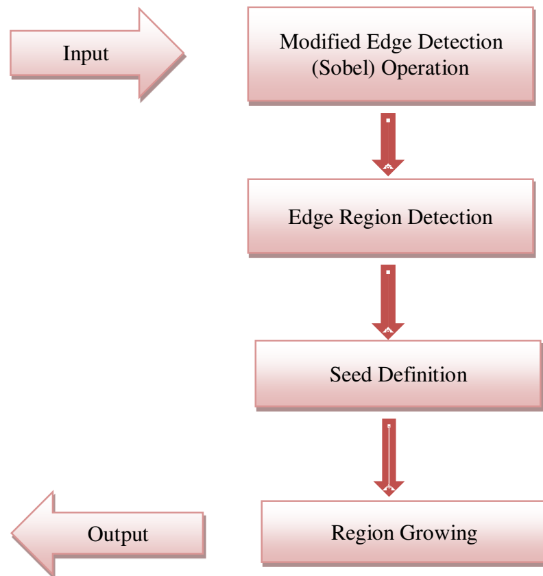
Figure 11 Sub steps of Segmentation Process
