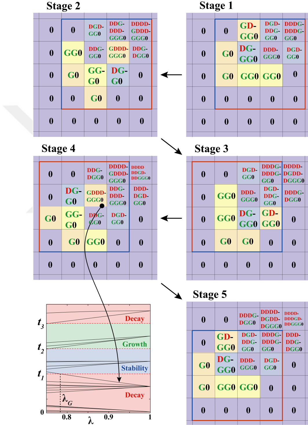
Figure 4.1: Five stages of evolution of the Glider in the Logistic GoL for \lambda = 0.8 . The set of operations is preserved for the initial and final stages. Bottom graph: Neighborhood sums versus \lambda . The first change in operation regions of sums occur at \lambda = \lambda_G , corresponds to the cell shown by the arrow.
