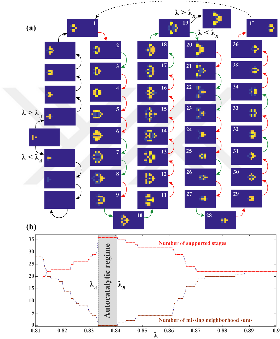
Figure 4.2: (a) Formation of period-36 propagator named Rayfish from simple initial conditions. The red arrows indicate the steps present also in Conway's GoL. 1^* and 1 denote the same but translated states. (b) Red lines represent the number of Rayfish stages that are dynamically reachable versus \lambda . The stages supported by the neighborhood sums form an autocatalytic loop only in the shaded interval. Outside this interval the neighborhood sums change their operation regions, as shown by the brown lines.
