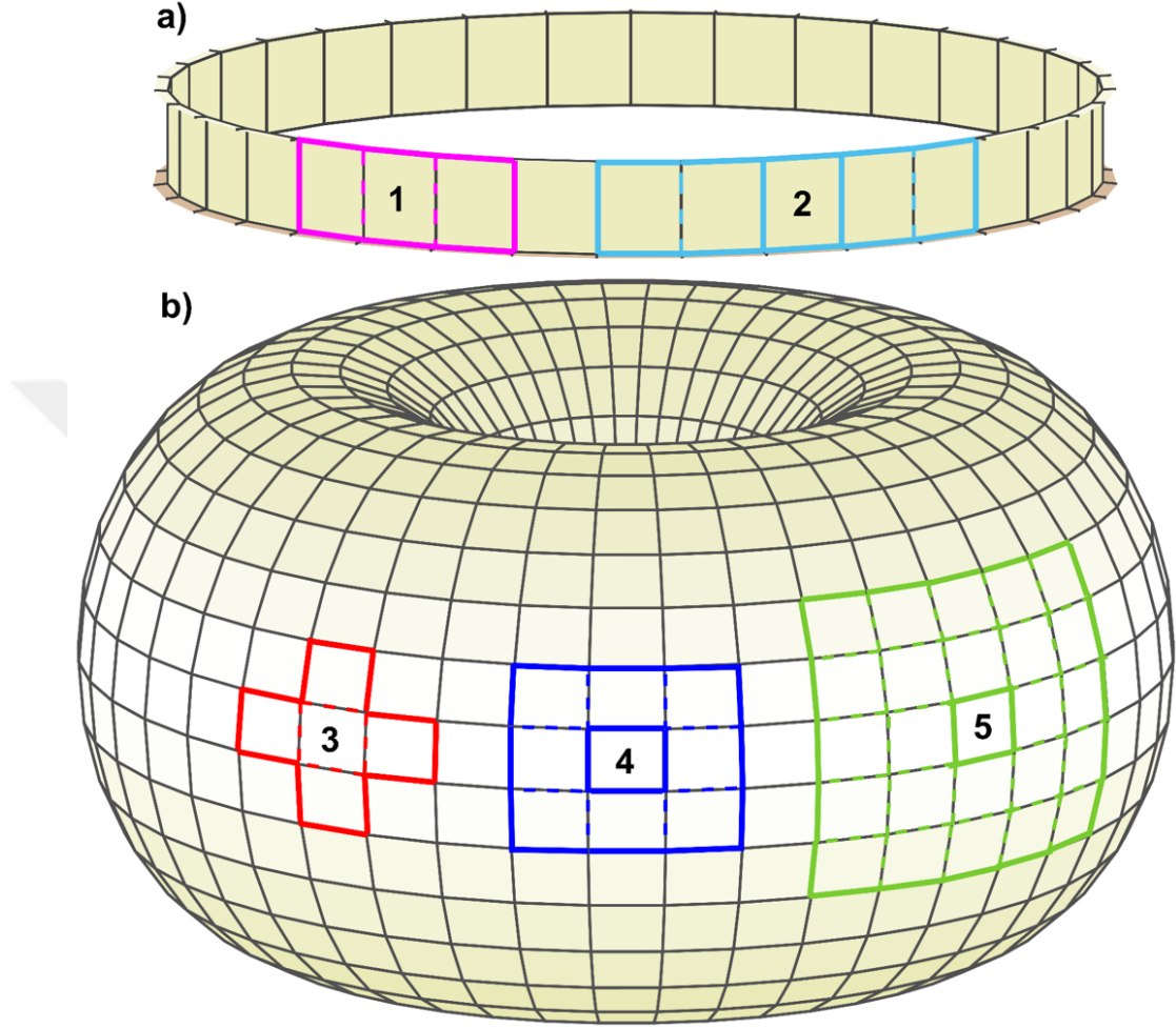
Figure 1.1: (a) One dimensional cellular space with periodic boundary conditions. 1 and 2 represent two different neighborhoods of D = 1 , \phi = 1 and \phi = 2 , respectively. (b) Two dimensional cellular space of square lattice and periodic boundary conditions. 3 represents the von Neumann neighborhood, 4 ( D = 2 , \phi = 1 ) is the Moore neighborhood and 5 is an example of larger neighborhoods ( D = 2 , \phi = 2 ).
