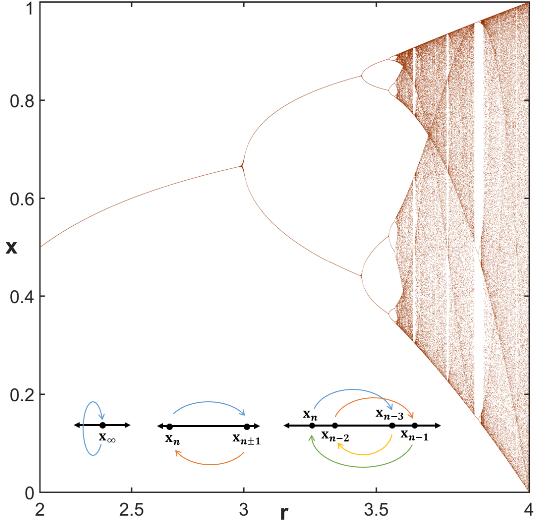
Figure 2.1: Population x versus tuning parameter r in the Logistic Map. From a single steady state solution the system reaches chaotic behavior after a series of period doubling bifurcations. Illustrative diagrams are shown in the bottom.
