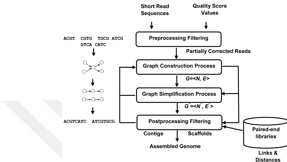
Figure 2.1: Schematic representation of the four stages of the next-generation genome assembly process (adapted from [2])
