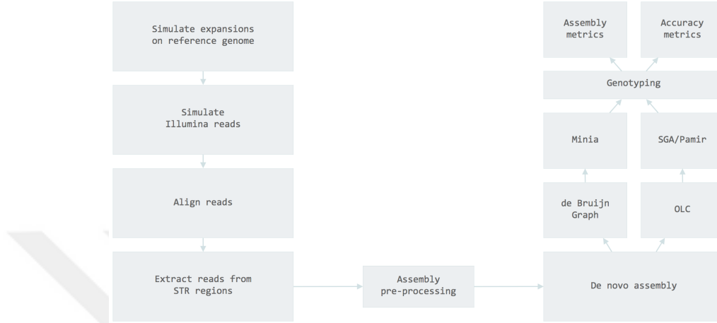
Figure 3.1: STR characterization pipeline
