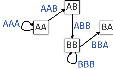
Figure 2.2: de Bruijn graph of AAABBBBA with k-mer length 3 (adapted from [3])
