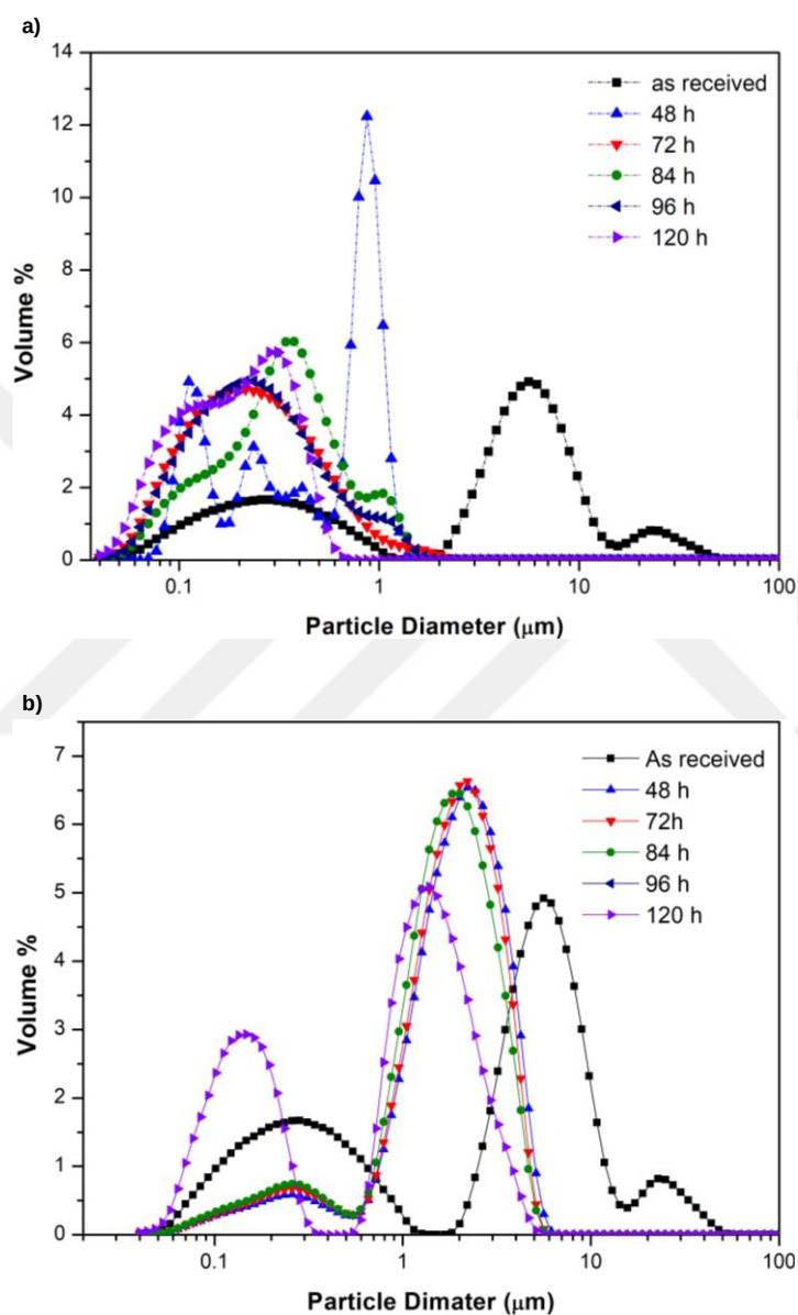
Figure 4.2. Particle size distribution of the LTA zeolite milled for 48,72,84,96 and 120 hours a) in ultrapure water b) in ethanol
