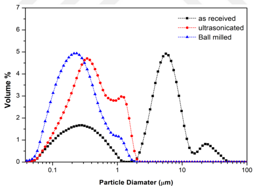
Figure 4.5. DLS Particle size distribution of as received and treated LTA powders by selected optimum process parameters. For Ball milling 72 hours at 50 rpm were employed and for an ultrasonic treatment were employed 5 minutes at 70 W in water.
