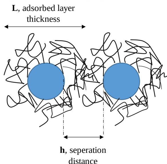
Figure 2.2. Schematic representation of the steric stabilization
