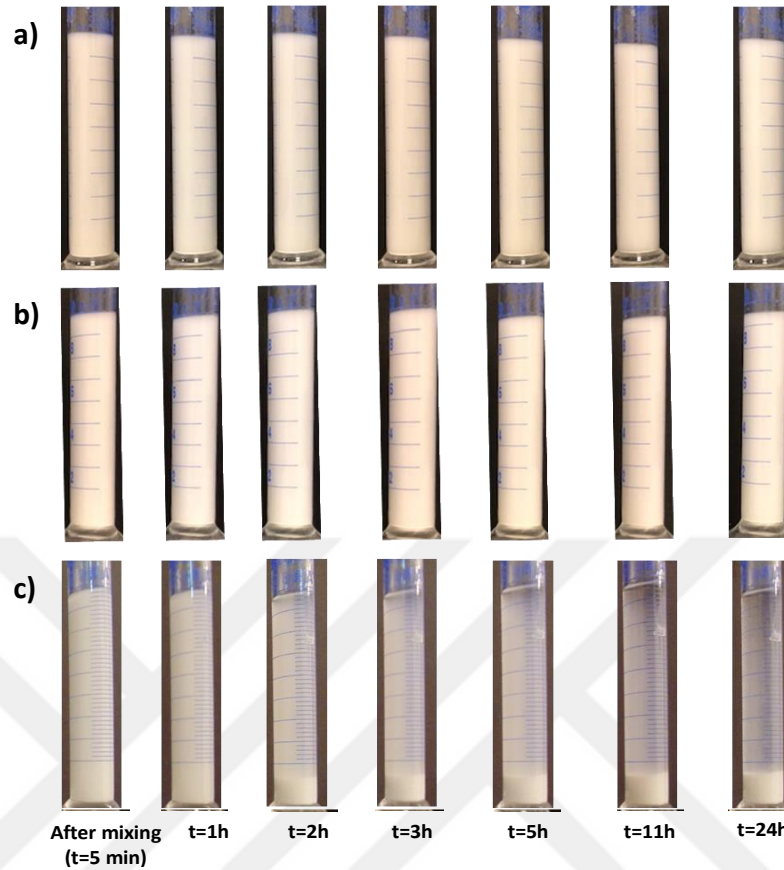
Figure 4.6. Sedimentation behavior of LTA type zeolites in ethanol:water is 30:70 in a, 40:60 in b and 50:50 in c, 1.5 wt% zeolites with respect to suspensions were used in each sample. The first image on the left-hand side is taken 5 min. after mixing LTA powders in ethanol-water mixtures.
