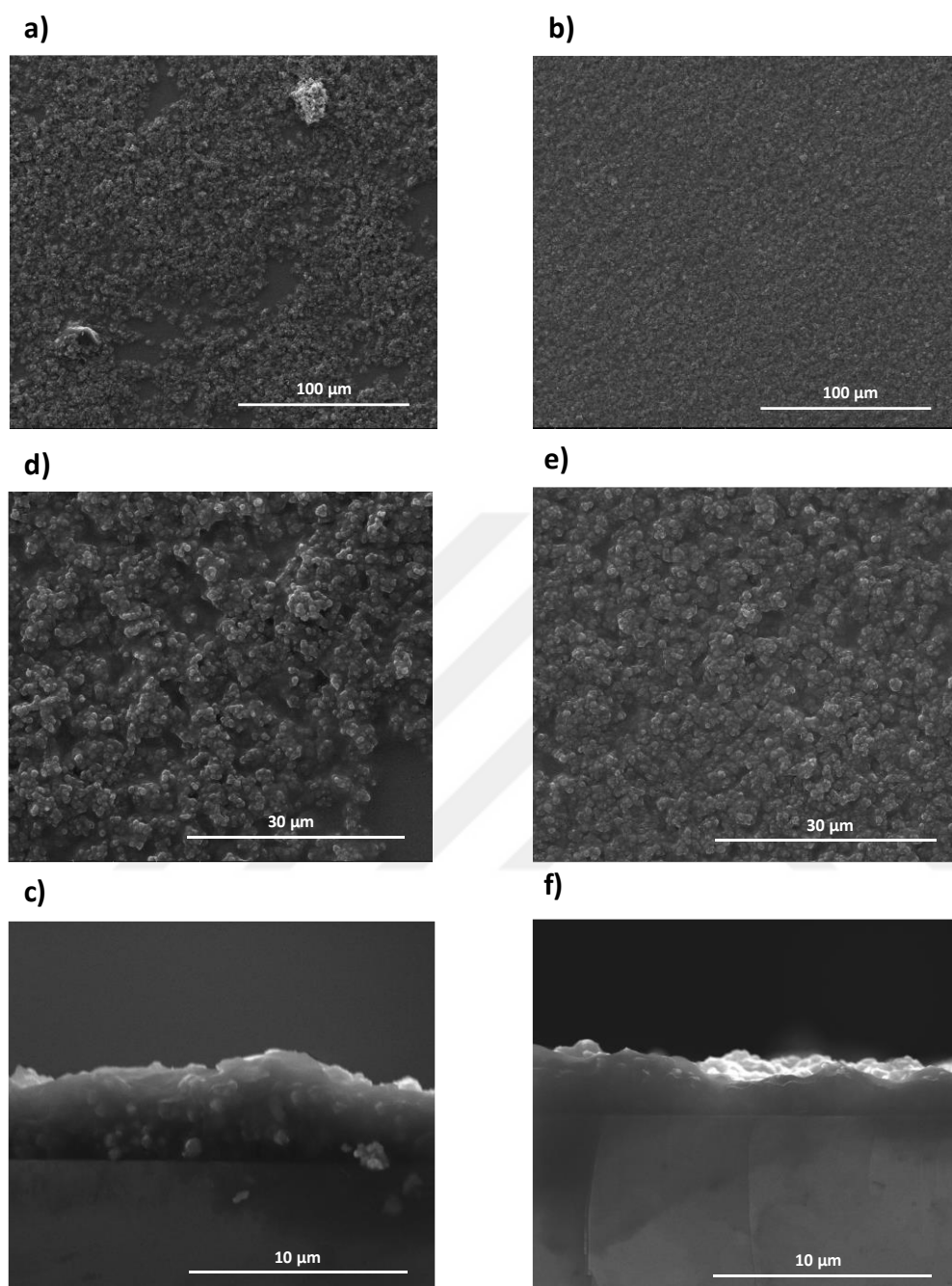
Figure 4.14. SEM micrographs of the LTA zeolite films by spin coating of the 10wt% zeolite powders in PVP added suspension in the absence (a,b, and c) and presence (d,e, and f) of PEG molecules in the ethanol-water (50:50 wt%) suspension on a Si wafer
