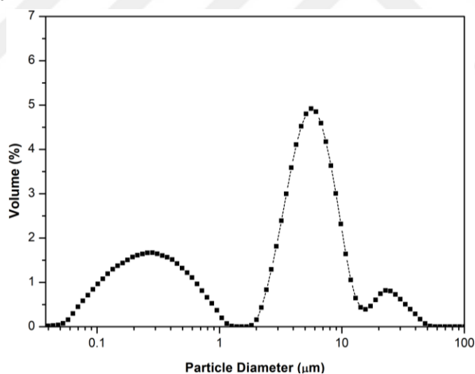
Figure 4.1. a) SEM micrographs and b) particle size distribution (by volume percentage) of as received LTA zeolite powder
