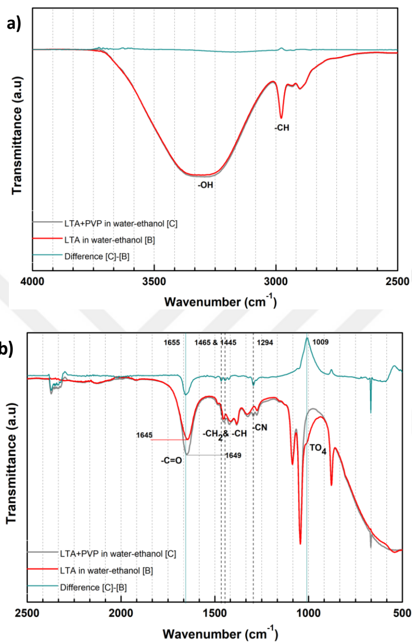
Figure 4.11. ATR-FTIR spectrum of zeolite suspensions in the absence (red spectrum) and the presence of PVP (gray spectrum). Green spectra are for the difference of the black and red spectrum. Samples contain 1.5 wt% of LTA powders with respect to suspension and 50:50 wt% of ethanol:water. The amount of PVP addition is the 10 wt% of zeolite powder. Spectrum is divided into two parts as the wavenumber range of 4000-2500 \text{cm}^{-1} (a), and 2500-500 \text{cm}^{-1} (b).
