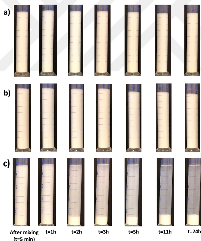
Figure 4.10. Sedimentation behavior of LTA zeolites in the presence of high molecular weight PVP in ethanol:water mixtures. 1.5 wt% zeolites with respect to suspension, 10wt% PVP with respect to zeolite powder were used. Ethanol to water ratio is a) 30:70, b) 40:60, and c) 50:50.
