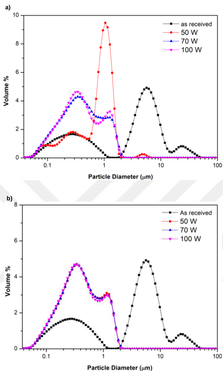
Figure 4.3. DLS particle size distribution of LTA zeolite in water as a function of ultrasonic treatment a) for 3 minutes treatment time b) for 5 minutes treatment time. 50, 70 and 100W powers were employed.
