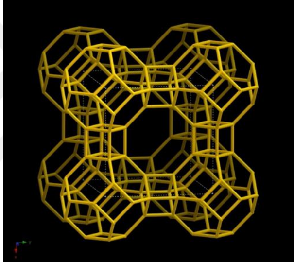
Figure 2.6. LTA zeolite viewed along [100] retrieved from IZA [65]
