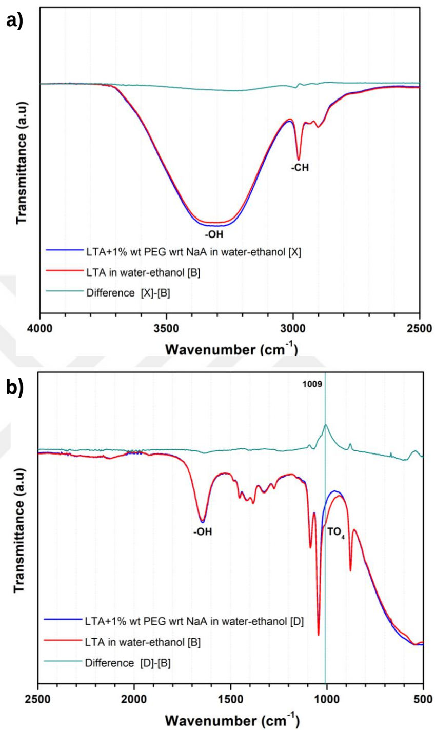
Figure 4.9. ATR-FTIR spectrum of zeolite suspensions in the absence (red spectrum) and the presence of PEG (blue spectrum). Spectrum is divided into two parts as the wavenumber range of 4000-2500 cm -1 (a), and 2500-500 cm -1 (b). Green spectra is for the difference of the blue and red spectrum.
