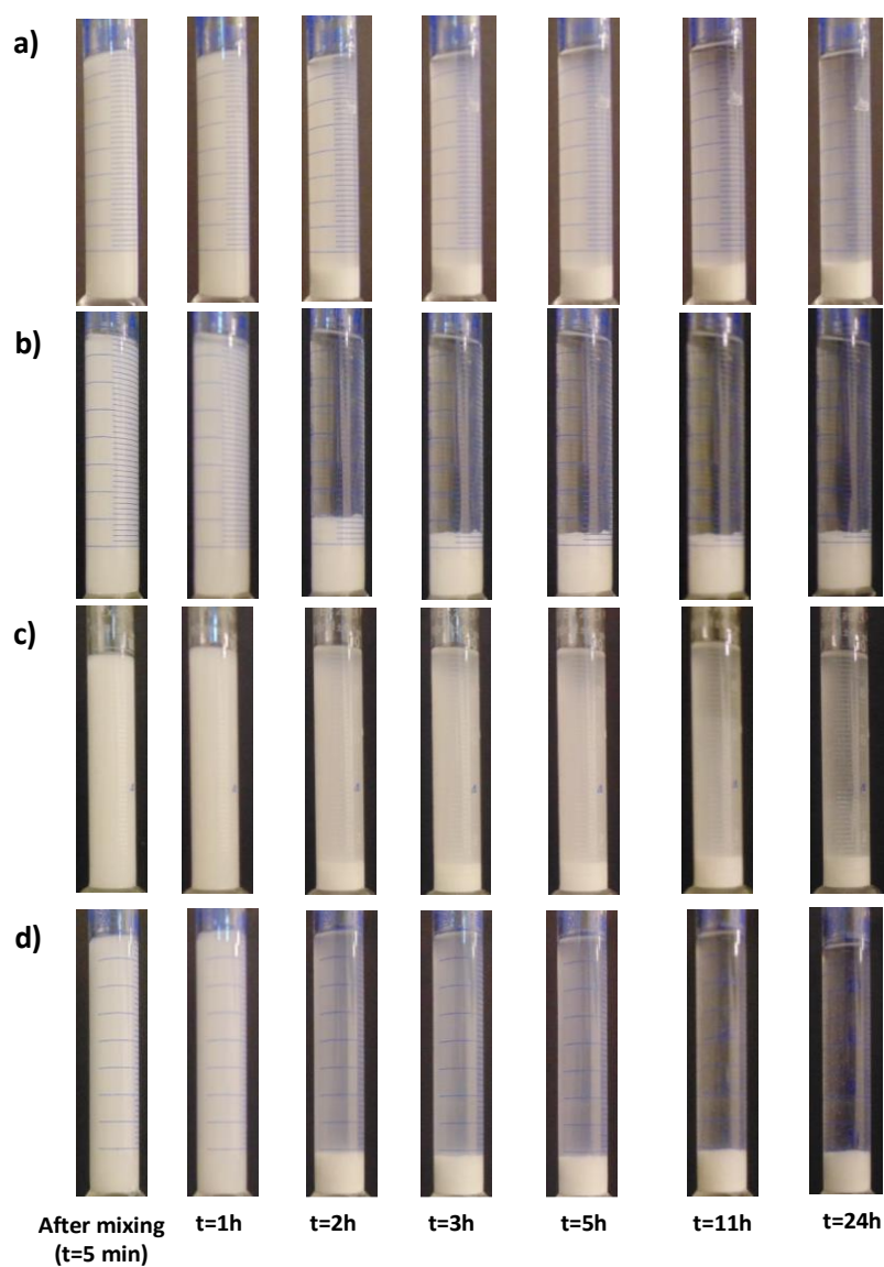
Figure 4.7. The effect of polyelectrolyte additions on the sedimentation behavior of LTA type zeolites in ethanol-water solutions in the: a) absence of additive; with addition of b) PAA; c) CTAB; and d) SLS. 1.5 wt% LTA zeolite used in ethanol-water mixture (50:50 wt%) for all samples and polymer concentration was 1 wt% of the zeolite powder.
