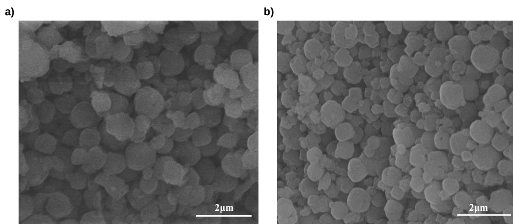
Figure 4.4. SEM micrographs of LTA powders a) powders after ball milling (72 hours at 50 rpm in water); b) powders after ultrasonic treatment (5 minutes at 70 W in water)
