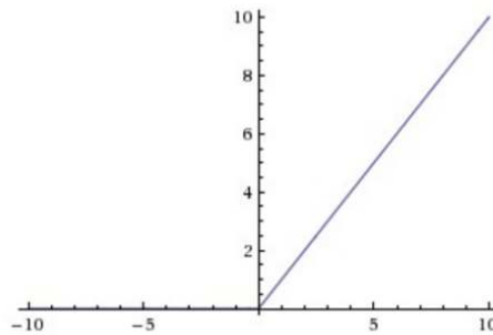
Figure 3.22 ReLU
