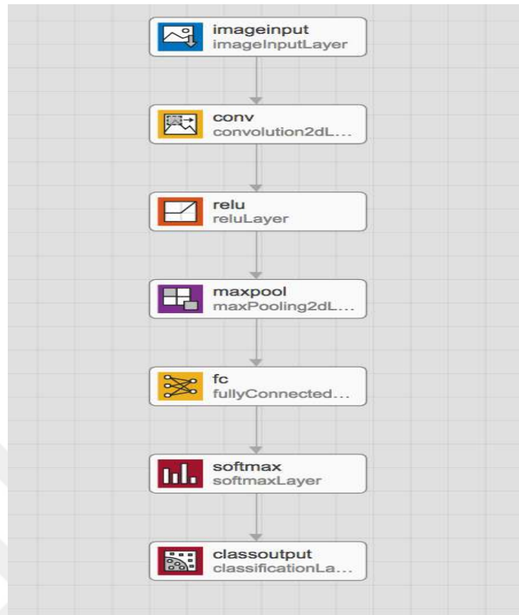
Figure 4.6 CNN layers
