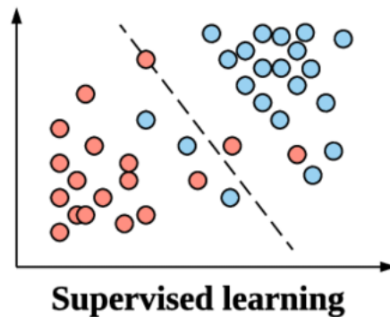
Figure 3.1 Supervised Learning
