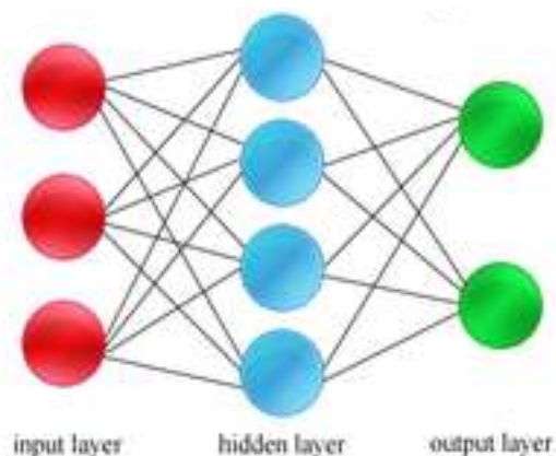
Figure 3.28 The NN
