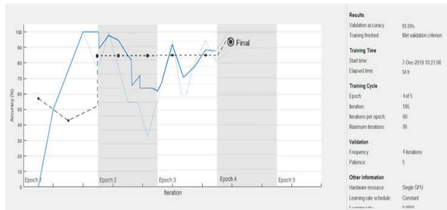
Figure 5.2 Training
