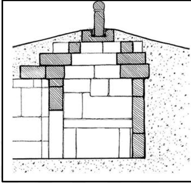
a.Hierapolis Tp92 no.lu Tmls.
