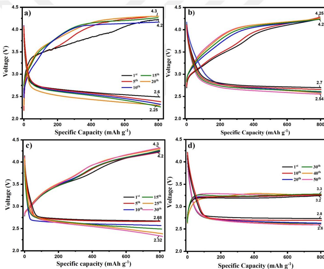
Figure 6.23. rGO (a), rGO@Pd (b), rGO@ \alpha\text{-MnO}_2 (c), and rGO@Pd@ \alpha\text{-MnO}_2 (d) cycling performance at fixed capacity of 800 mAh g -1 for 7 hours.
