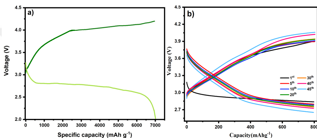
Figure 6.27. Full discharge and charge curves of v- \text{MnO}_2 /rGO (a) and its cycling performance at limited capacity 800 \text{mAh g}^{-1} (b).
