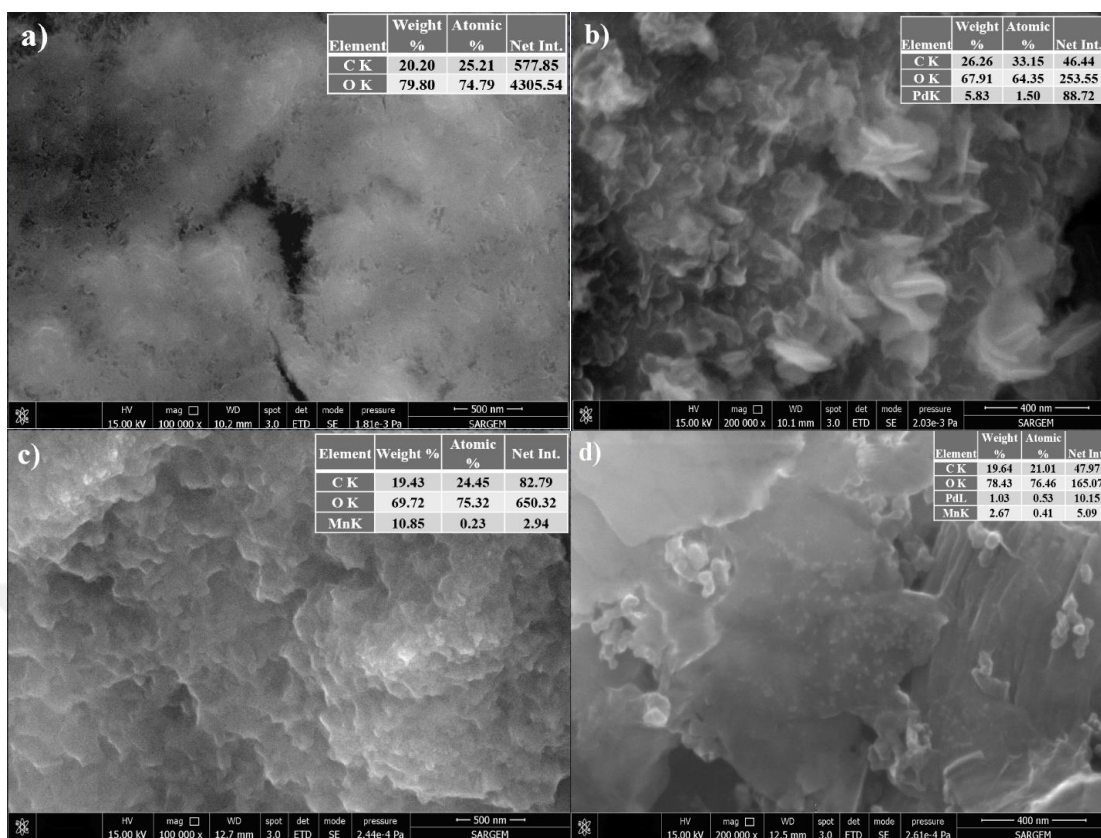
Figure 6.18. Surface analysis of electrodes after first discharge curve of a) rGO, b) rGO@Pd, c) rGO@ \alpha -MnO 2 , and d) rGO@Pd@ \alpha -MnO 2 nanocomposites air cathodes.
