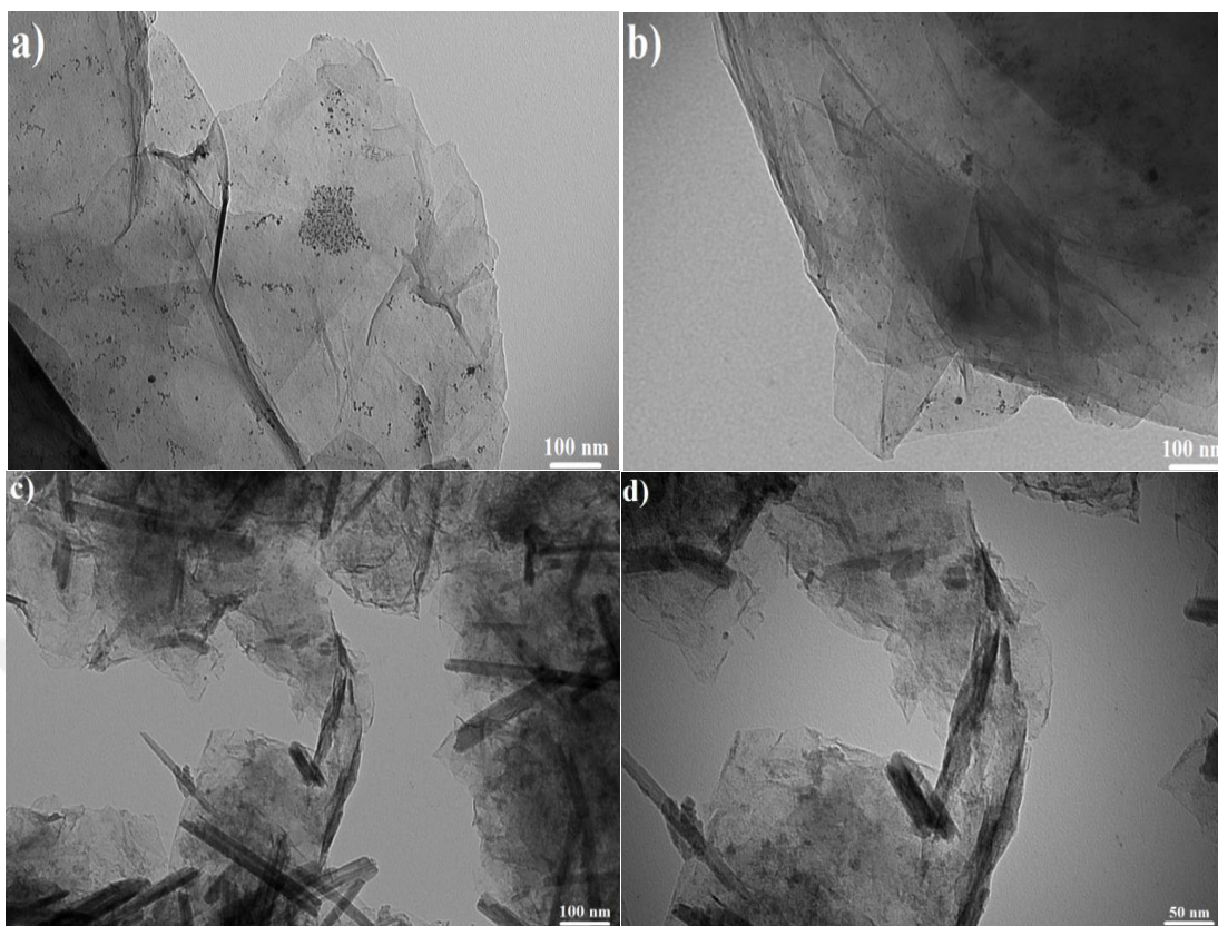
Figure 6.12. TEM images reveal the dispersion of Pd on rGO surface (a,b) and \alpha -MnO 2 nanowires anchored on rGO@Pd (c,d).
