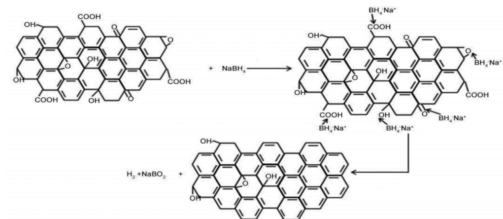
Figure 6.2. Schematic of the GO reduction mechanism by \text{NaBH}_4 .
