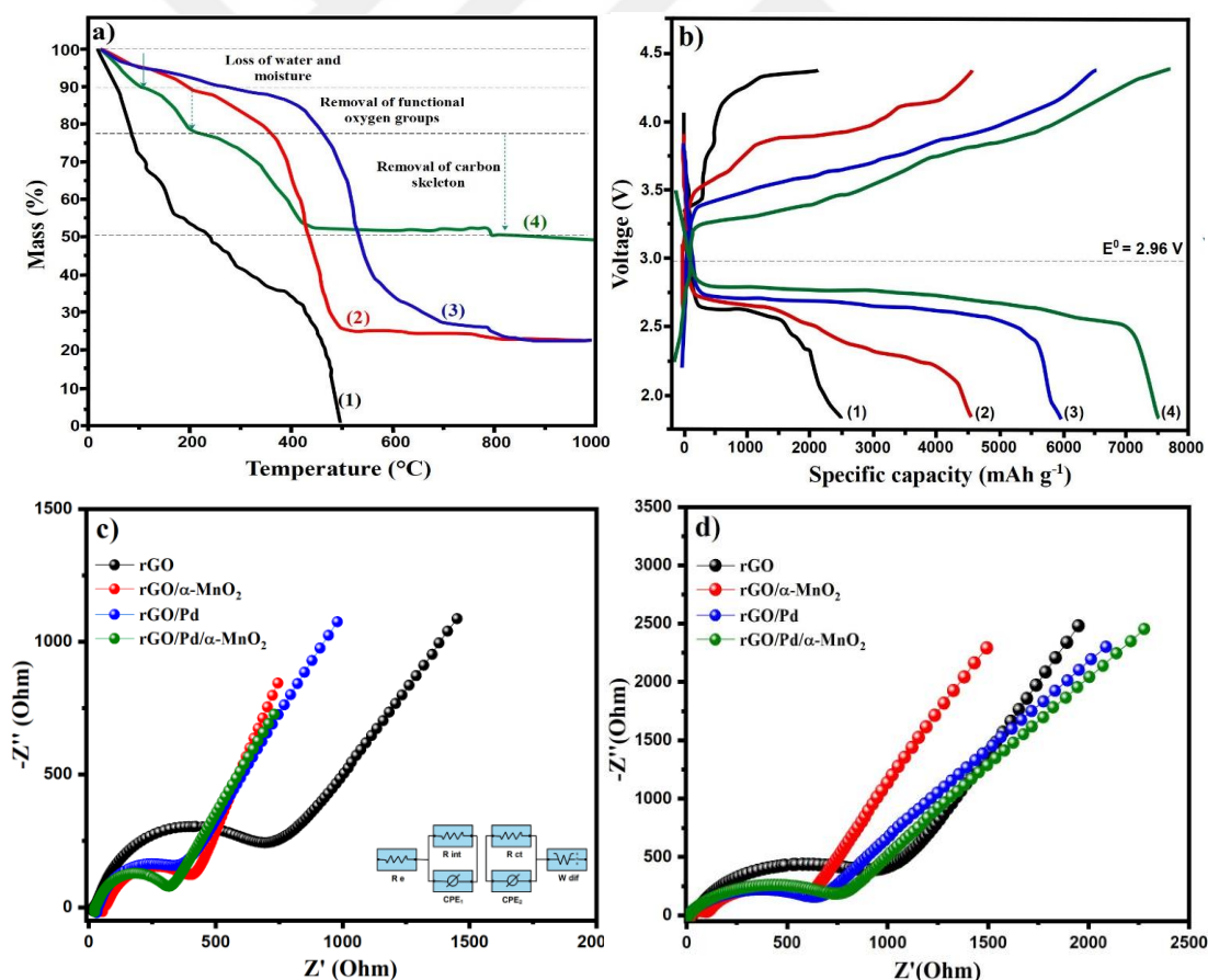
Figure 6.17. a) Thermal properties of rGO, \text{rGO@}\alpha\text{-MnO}_2 , \text{rGO@Pd} , and \text{rGO@Pd@}\alpha\text{-MnO}_2 hybrids (4). b) At a current density of 100 \text{ mA g}^{-1} , discharge/charge curves of rGO (1), \text{rGO@Pd} (2), \text{rGO@}\alpha\text{-MnO}_2 (3), and \text{rGO@Pd@}\alpha\text{-MnO}_2 (4) cathodes. The electrodes' electrochemical impedance data before (c) and after (d) first discharge.
