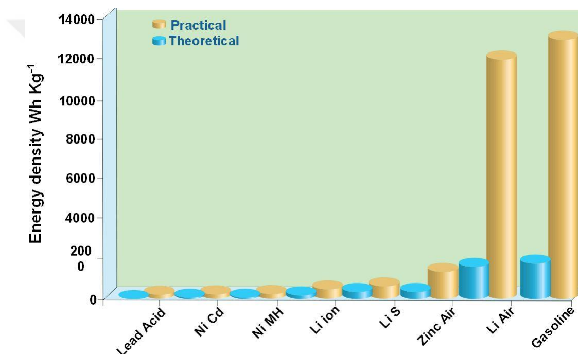
Figure 1.1. Comparison of gasoline the gravitational energy density Wh kg -1 for different types of rechargeable batteries.
