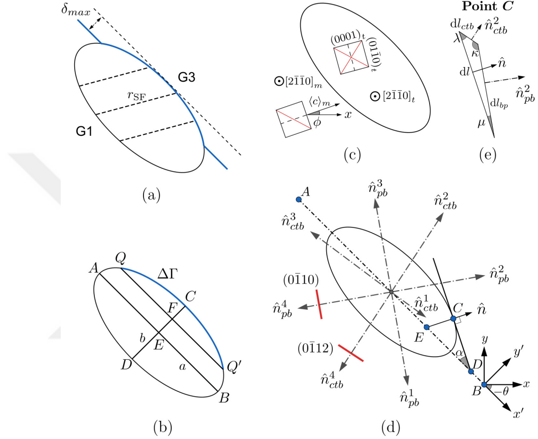
Figure 4.1. The sketches show (a) the bulging of the twin into the neighboring grain and the distribution of SFs inside the twin, (b) the \Delta\Gamma boundary modeled as the Q'Q arc, (c) crystallographic planes that contribute to twin boundary faceting, (d) orientations of the boundary plane normals for the twin lattice and (e) an example triangle construction for boundary decomposition at the representative point C .
