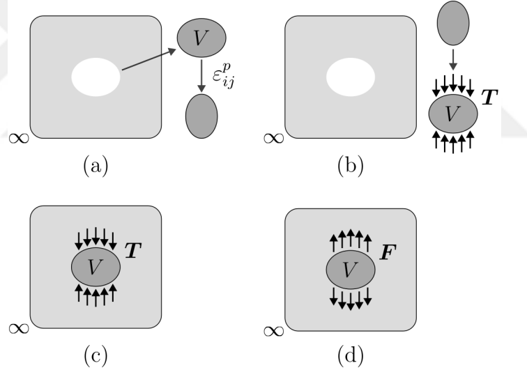
Figure 2.7. The steps of the Eshelby thought experiment. (a) A region (e.g. a twinned region) is cut from the medium and an eigenstrain is applied. (b) The shape of the region is restored to its original state by applying a traction on its surface. (c)
