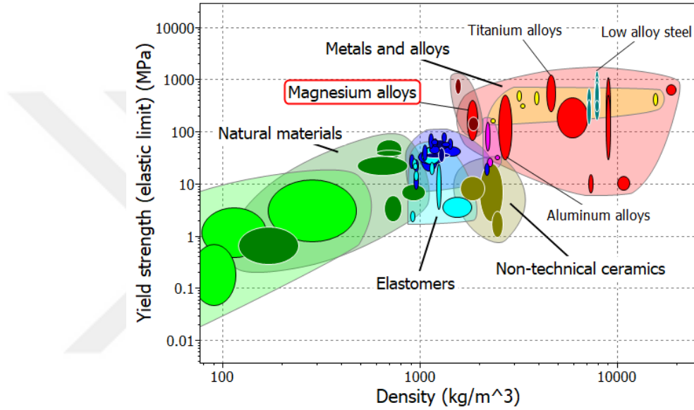
Figure 1.1. Strength vs. density mapping of engineering material families.
