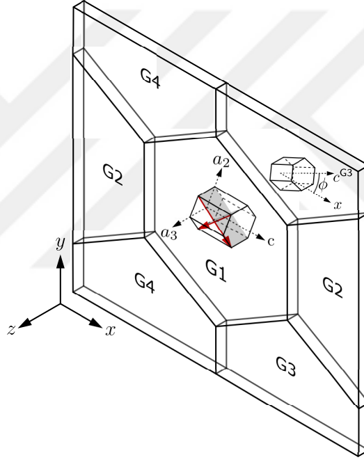
Figure 3.1. Schematic of the periodic quasi-2D simulation cell with honeycomb grains. The [\bar{1}120] crystal axes of all grains are aligned with the global z -axis. Grains 2, 3 and 4 are tilted by a rotation of \phi about the global z -axis. The (\bar{1}102) and (1\bar{1}02) planes associated with the activated \{10\bar{1}2\} tension twin system are highlighted in the central unit cell.
