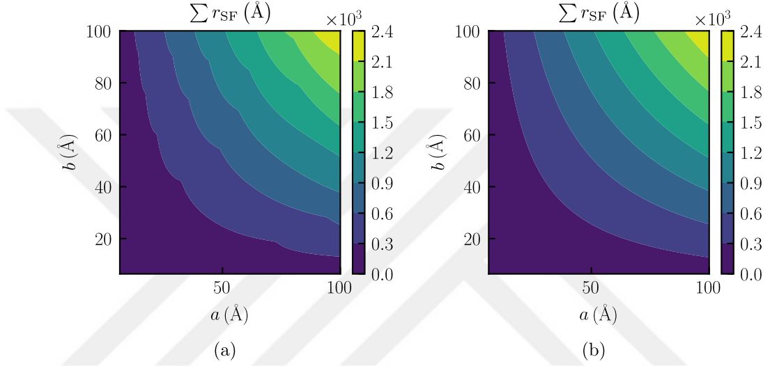
Figure 4.4. Contourplots of the length sum of stacking fault lines as estimated by the (a) explicit stacking fault and (b) statistical distribution of stacking faults approaches over a range of a and b .
