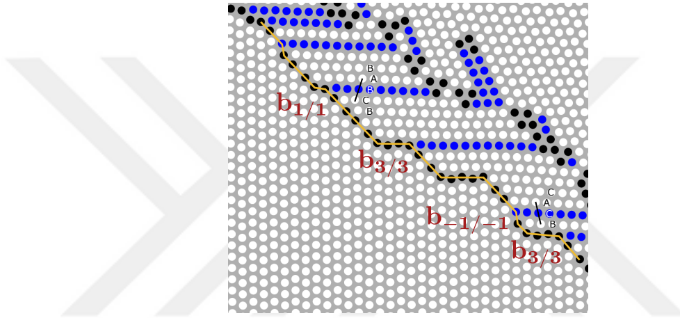
Figure 3.12. I_1 basal stacking faults inside the \{10\bar{1}2\} twin. Each SF is bounded by a defect pair that anchors the SF to the twin boundary on the left and the grain boundary on the right. Defects in the TB have disconnection Burgers vectors denoted by \mathbf{b}_{\pm\mu/\pm\kappa} , corresponding to two different changes in the stacking sequence. The stacking changes associated with \mathbf{b}_{1/1} and \mathbf{b}_{-1/-1} steps are identified.
