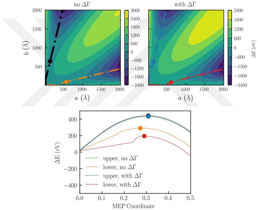
Figure 4.14. The alternative MEP paths between the origin and basin states at \sigma_{yy} = -0.95 GPa stress that include and exclude the contribution of the \gamma_{\Delta\Gamma}A_{\Delta\Gamma} term are shown. Below the potential energy plots is the energy profile along each MEP.
