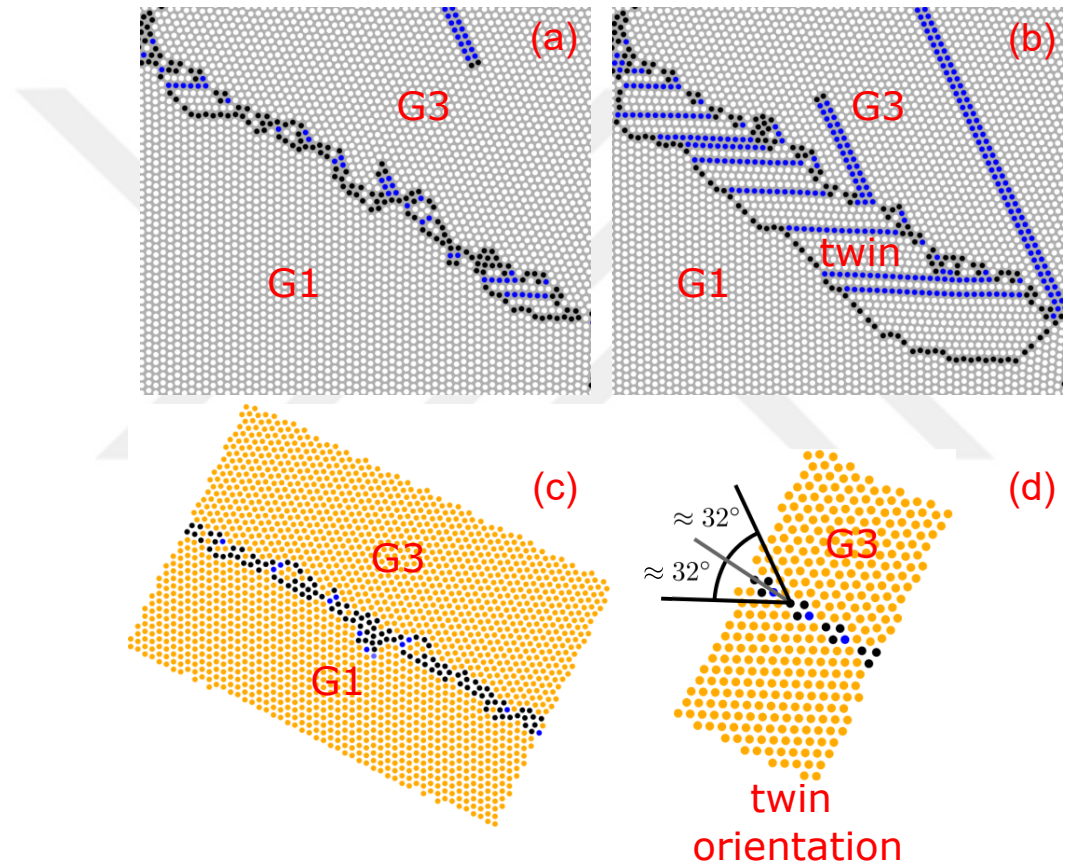
Figure 3.14. (a) Snapshot of the ATGB grain boundary between G1 and G3 at LP0. (b) The propagation of the twin transforms the twin-G3 GB into a (nearly) STGB. (c) The partially-relaxed ATGB structure between G1-G3 prior to equilibration. (d) A fully relaxed GB with identical grain boundary character to the twin-G3 GB.
