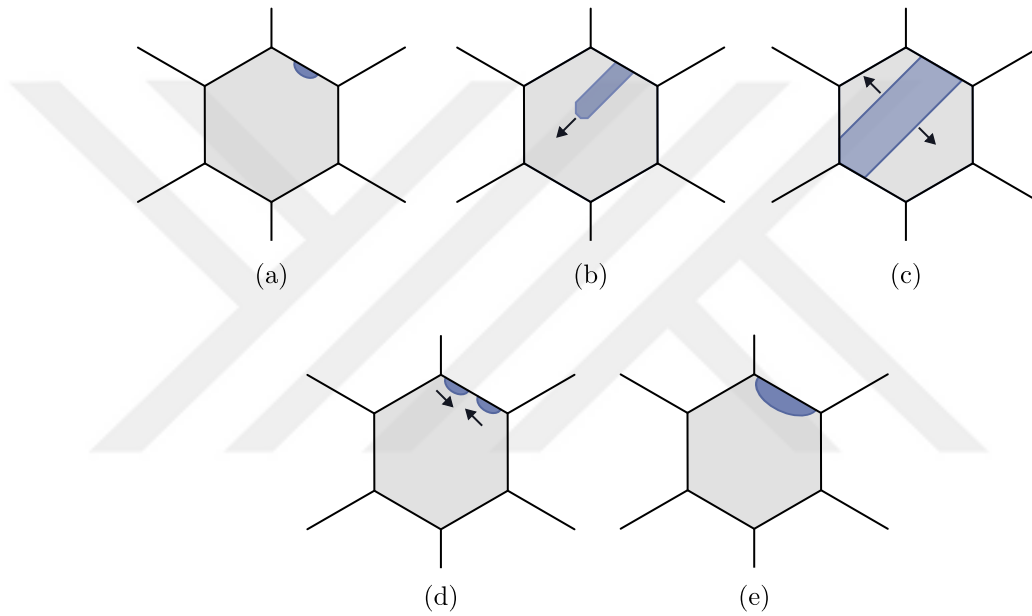
Figure 1.3. Sketches show (a-b-c) the nucleation, propagation and growth stages of deformation twinning. (d-e) Alternatively, multiple twin nuclei can nucleate from the same grain boundary. Depending on the character of the grain boundary, these nuclei can grow along the grain boundary and coalesce to generate a larger twin [79].
