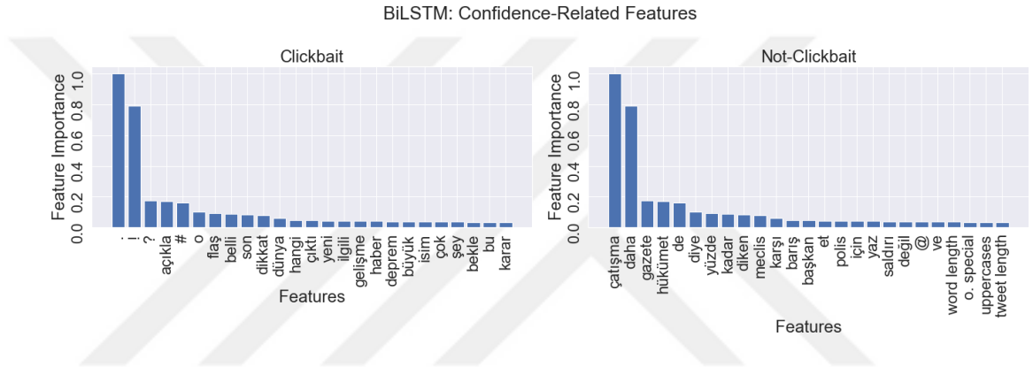
Figure 18: Confidence-based features of the BiLSTM model.
