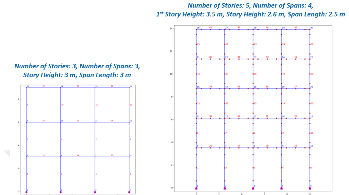
Figure 2.6. Example building models in the OpenSeesPy framework: 3- and 5-story buildings.
