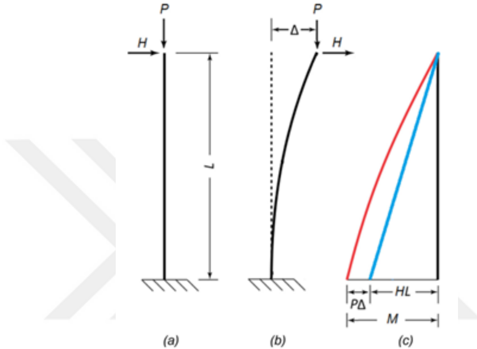
Figure 2.13. P-Delta effect: (a) undeformed configuration, (b) deformed configuration, (c) bending moment distribution (Burgos and Silva, 2023).
