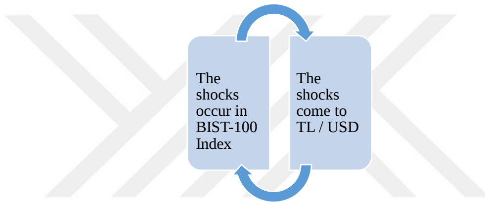
Figure 3.17 Impulse Response Test Result
