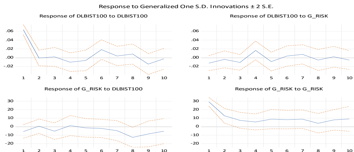
Figure 3.13 Impulse response ( BIST-100 & GR )
