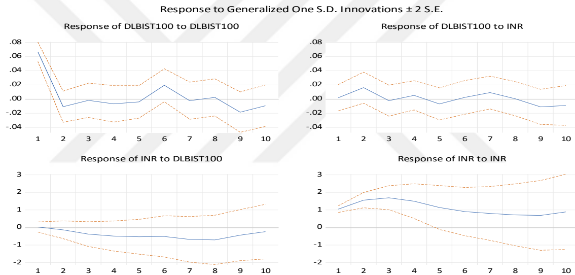
Figure 3.15 Impulse response (BIST-100 & INR)
