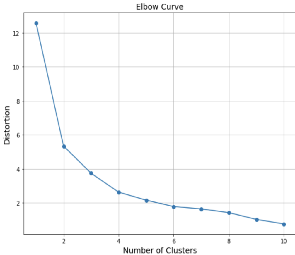
Figure 2.8: Elbow Curve
