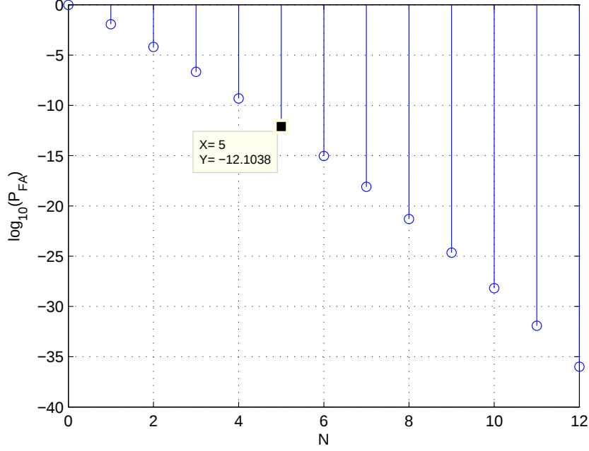
Figure 3.1: Probability of false alarm versus N for the N out K fusion rule.
