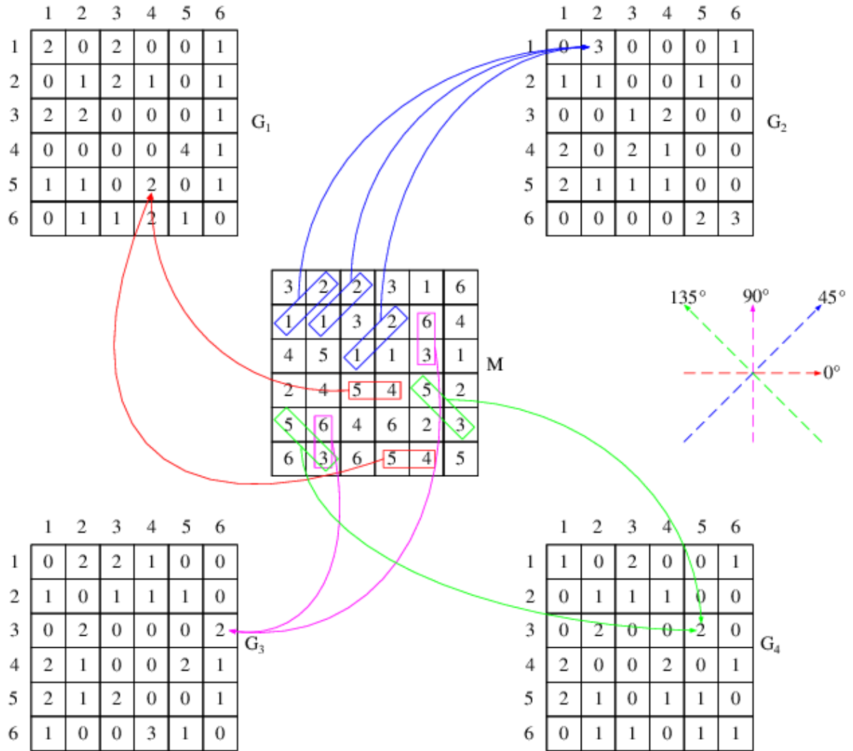
Figure 3.3: Example calculation of the GLCM matrix. G_1 is a horizontal calculation of the GLCM matrix. G_2 is a diagonal up calculation of the GLCM matrix. G_3 is a vertical calculation of the GLCM matrix, and G_4 is the diagonal down calculation of the GLCM matrix [8].
