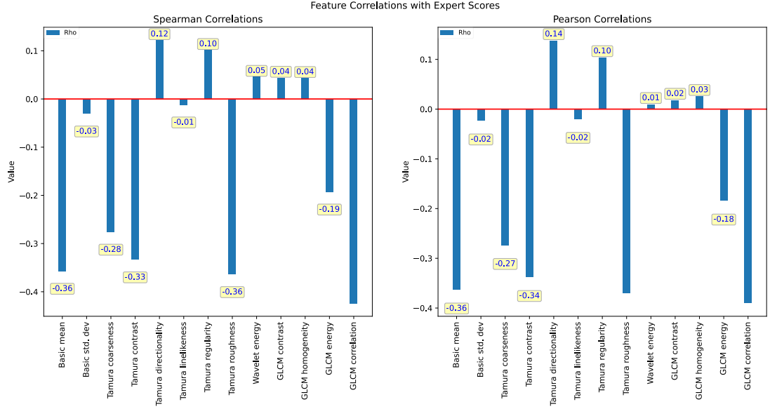
Figure 5.2: Feature correlation results for pilling assessment.
