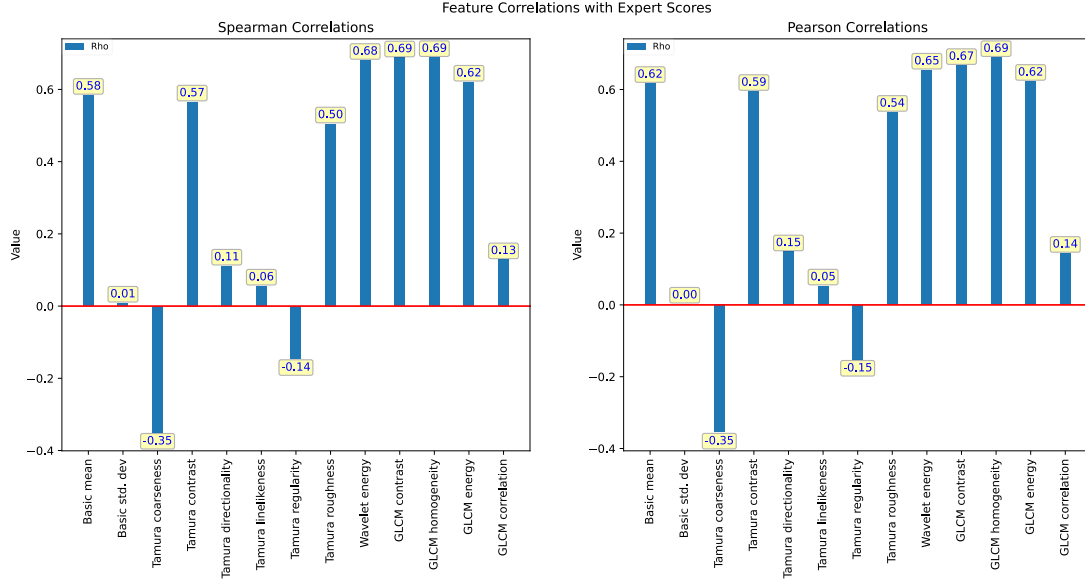
Figure 5.1: Feature correlation results for softness assessment.
