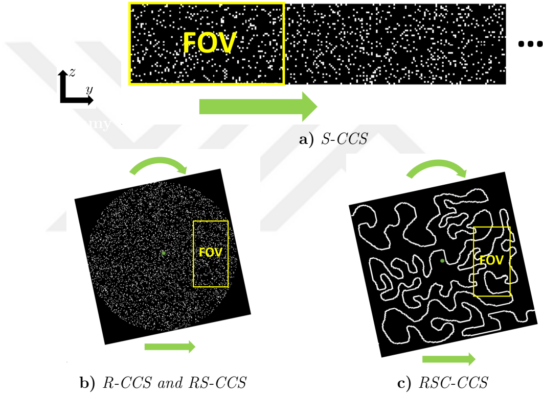
Figure 4.2: Different implementations of CCSs. a) Sliding CCS ( S -CCS) filled randomly with MNPs and slid through the FOV. The length of the CCS is determined by the number of measurements and the amount of shift between two consecutive measurements. b) Rotating CCS ( R -CCS) filled randomly with MNPs and rotated about its center. The R -CCS can be slid after a 360^\circ turn, and rotated about a different axis, which is named as a Rotating and Sliding CCS ( RS -CCS). c) Rotating and sliding connected CCS ( RSC -CCS), where the MNPs are connectively distributed for a very practical implementation.
