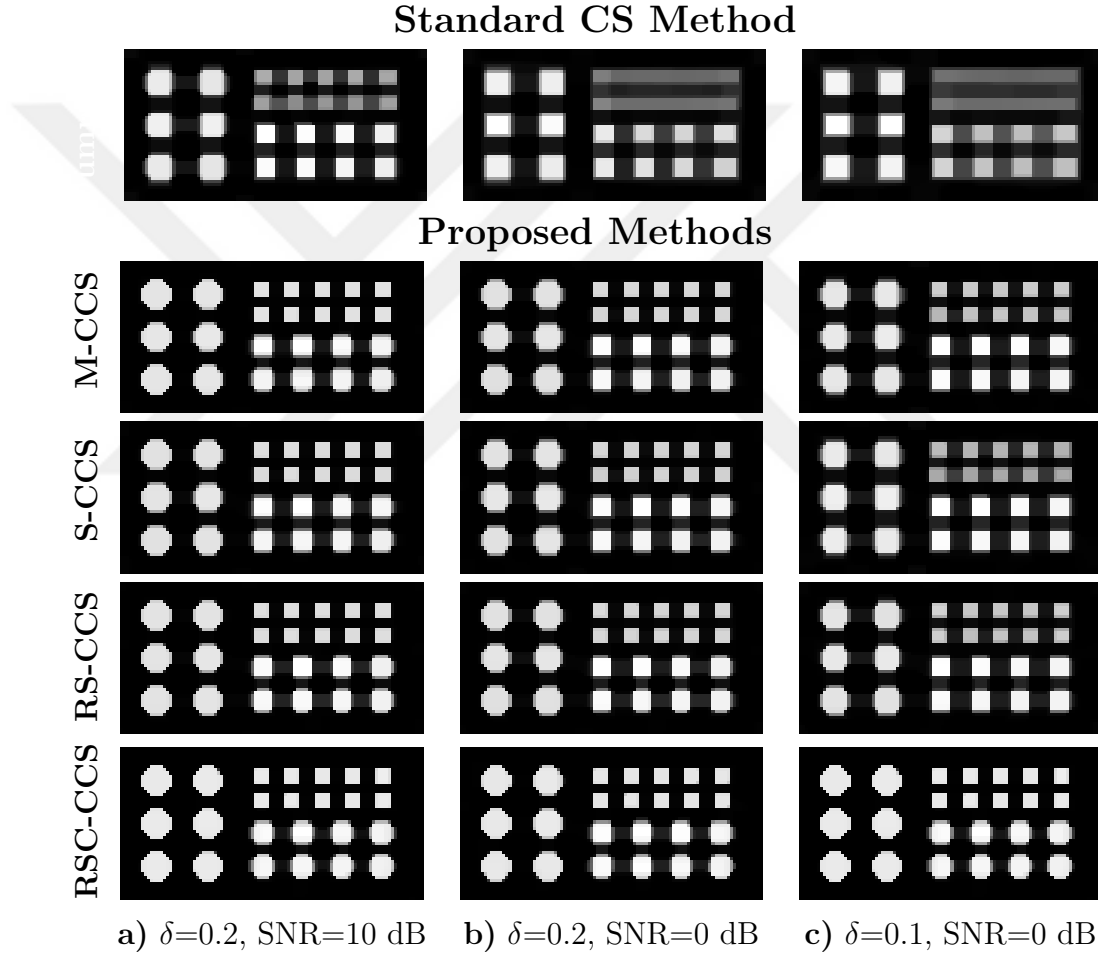
Figure 4.10: Reconstructed images with system matrices reconstructed via M-CCS, RS-CCS, RSC-CCS, S-CCS (with 5 grid sliding step) types of CCSs, for a) \delta = 0.2 and 10 dB SNR, b) \delta = 0.2 and 0 dB SNR, and c) \delta = 0.1 and 0 dB SNR scenarios. The filling rate of the CCSs were 0.1.
