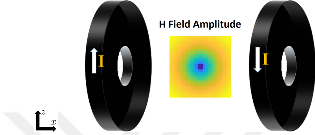
Figure 2.1: Maxwell coil pair to generate a FFP (blue region) in the FOV.
