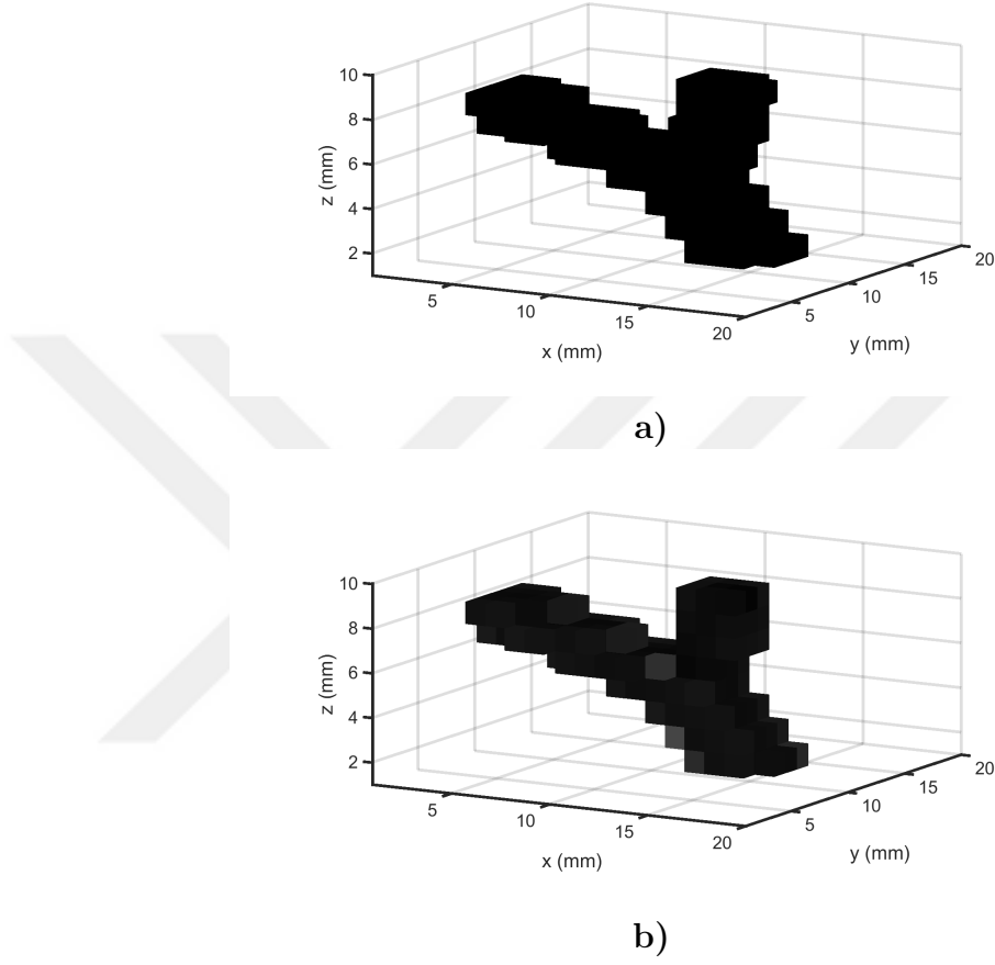
Figure 3.3: a) The reference object and b) the reconstructed object in noise-free environment with 100 iterations of ADMM.
