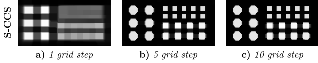
Figure 4.11: Image reconstruction results for the S-CCS with a) 1 grid sliding step , b) 5 grid sliding step , and c) 10 grid sliding step . \delta = 0.2 , SNR = 10 dB, and filling rate = 0.1.
