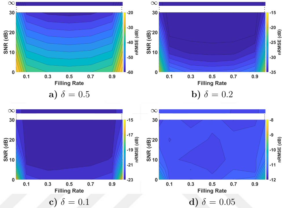
Figure 4.5: Contour plots of the nRMSE of the estimated system matrices for different filling rates and \delta 's for the M-CCS case. For the filling rates, the following values were used: 1/800 , 0.1, 0.3, 0.5, 0.7, 0.9, and 799/800 .
