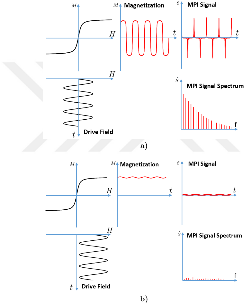
Figure 2.2: MPI signal encoding for the cases a) the MNP sample is in the FFP and b) the MNP sample is outside of the FFP, with its magnetization saturated. The MPI signal, which is proportional to the time derivative of the magnetization, is given on the right side of the figures, together with its spectrum.
