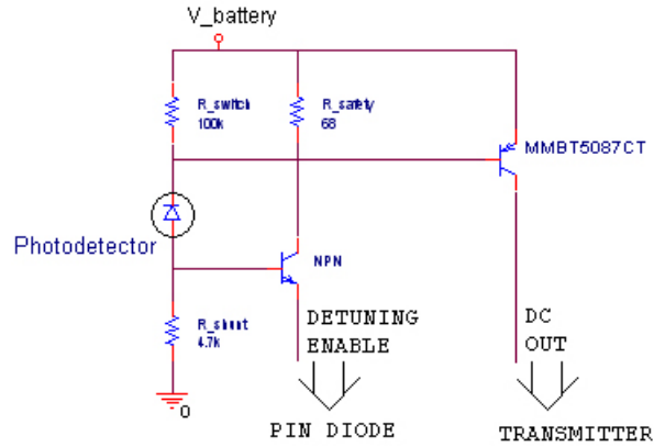
Figure 3.12: 3-state power circuitry: Increasing the light falling onto the photodetector triggers the PNP transistor which switches the rest of the circuit. Further intensification of the light also puts NPN transistor into ACT state - turning on the active tuning.
