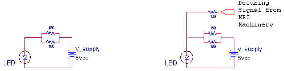
(a) Simple External Control Circuitry (b) Switching External Control Circuitry
