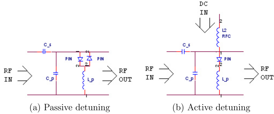
Figure 3.3: Types of detuning: Passive detuning relies on the self-biasing of two back-to-back PIN diodes by incoming high-power RF; whereas active detuning uses an external circuitry for the activation and deactivation of a single PIN diode.
