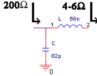
Figure B.2: Schematics of the L-match between the preamplifier and laser diode matching was required for efficient power transfer. The matching circuit of 68nH-82pF transforms the input impedance of the laser diode from several Ohms to around 200Ω.
