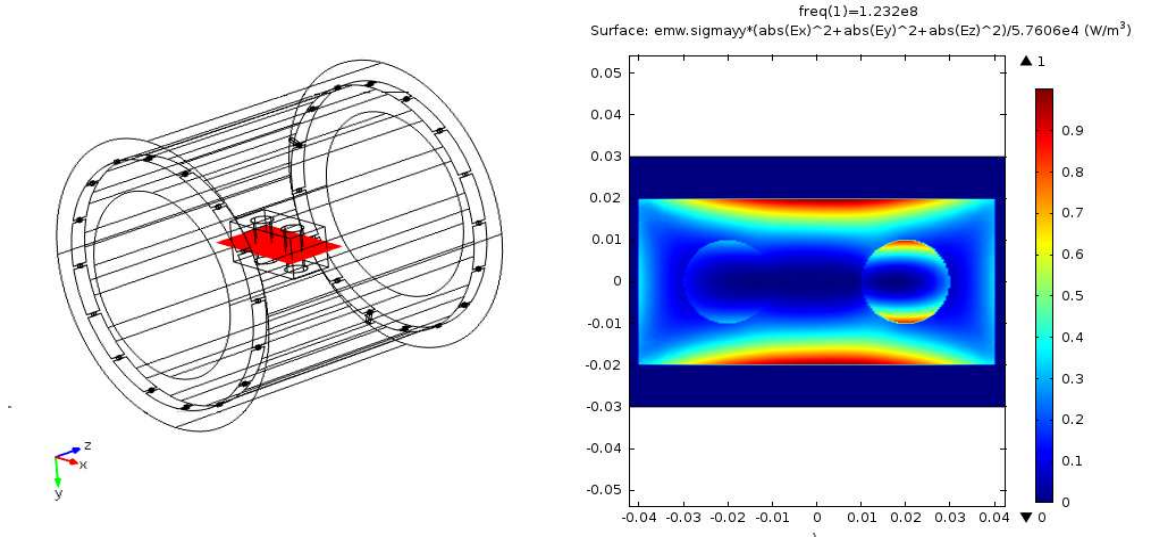
Figure 3.15: Normalized SAR distribution image (right) at the slice given on the left with a red color
