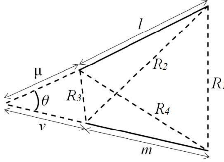
Figure 2.4: Schematic drawing for mutual inductance calculation between two conductive elements in the same plane
