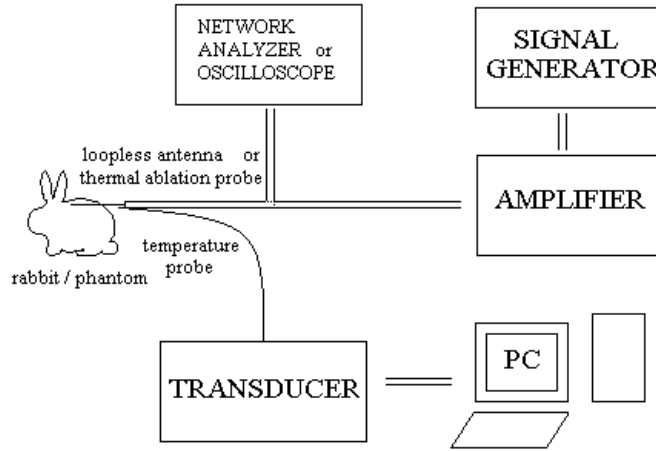
Figure 3.2: experiment setup: A loopless coil or a thermal ablation probe, fed via a signal generator and amplifier, is inserted into the tissue. A network analyzer or an oscilloscope is placed before the coil. An impedance measurement is performed to calculate power delivered to the subject. Identical experiments are performed where the rabbit is replaced with a gel phantom. A fiber-optic probe is attached to the antennas for temperature measurement.
