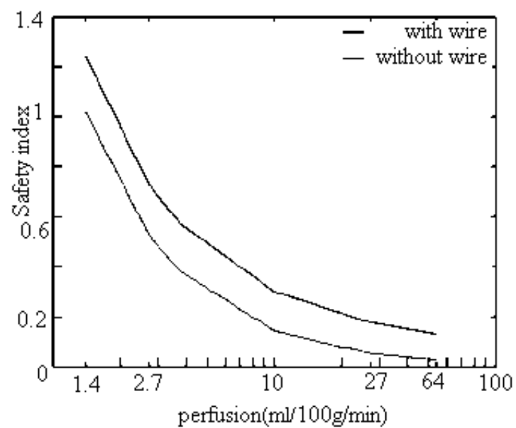
Figure 2.3: a 10-cm insulated wire (diameter = 0.5 mm, insulation thickness = 75\text{ }\mu\text{m} ). Safety index for each wire is compared to the wire-free safety index [15]
