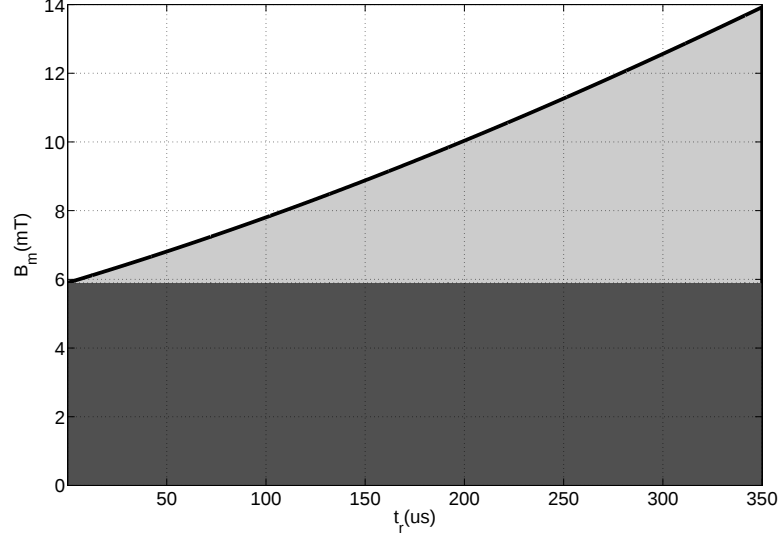
Figure 1.2: Magnetic field at stimulation vs. rise time [Eq.1.1] indicating PNS won't occur under specific magnetic field amplitude regardless of its frequency or rise time (dark gray area).
