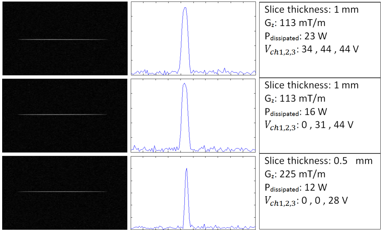
Figure 3.11: 2D coronal slice selection at xy plane along with center line plot and properties of each mode from top to bottom for large, mid-size and small VOI with fixed RF duration ( 800 \mu s ).
