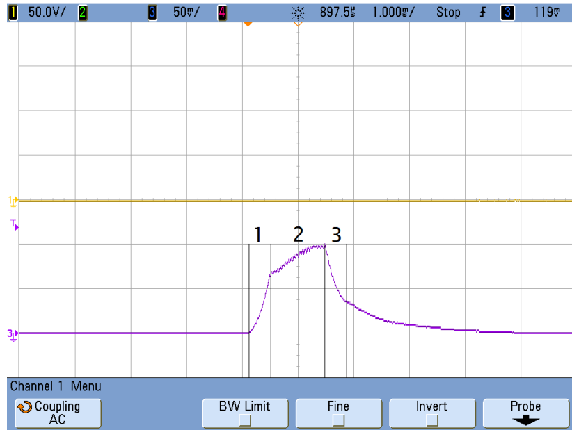
Figure 3.8: DC voltage (100 V) and current waveform (10mV/A scale) at the input of the GPA, while driving the coil with 730 \mu H inductance and 1.82 \Omega resistance by 26 A flat top current, with specified ramp up, flat top and ramp down regions as 1, 2 and 3, respectively.
