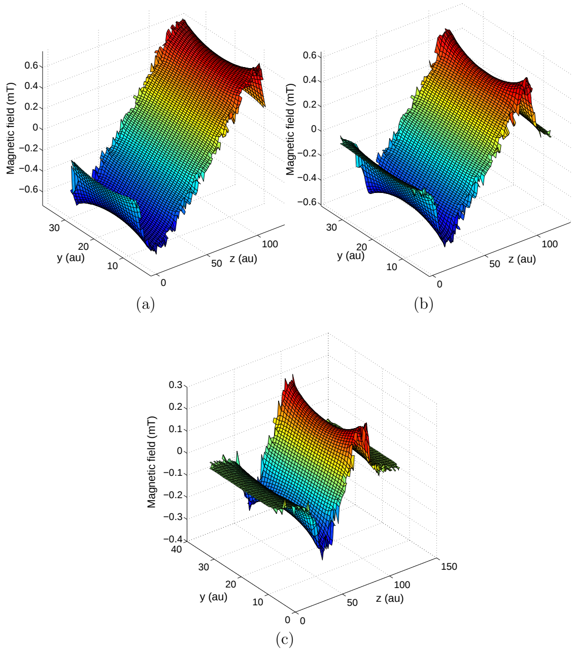
Figure 3.10: Measured magnetic field amplitude in yz plane for a: 0.29 : 0.2 : 0.11 A, b: 0 : 0.26 : 0.09 A, c: 0 : 0 : 0.15 A for outer, middle and inner channels, respectively with variable VOI similar to the simulation.
