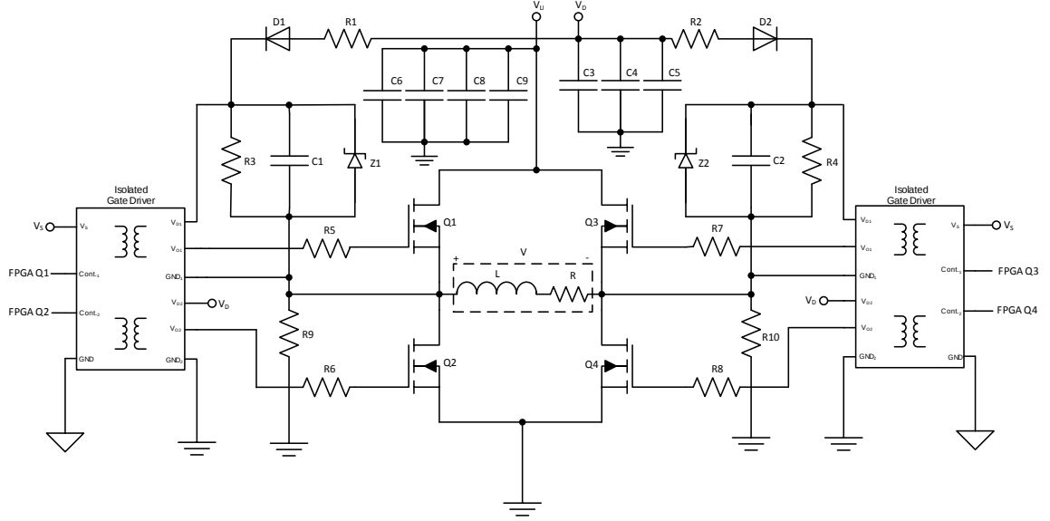
Figure 2.6: Circuit diagram of H-bridge GPA to drive our costume gradient coil.
