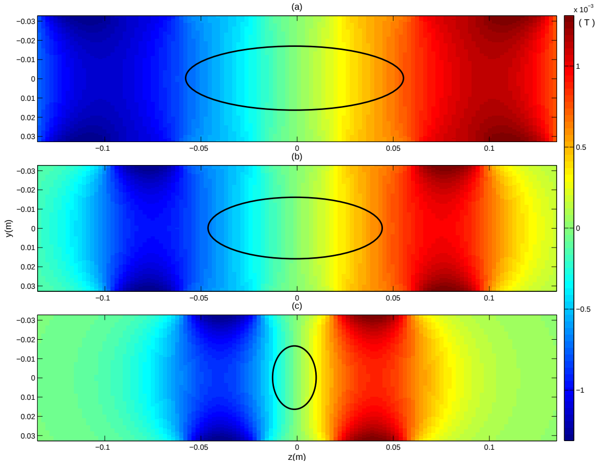
Figure 3.3: Linear magnetic field in yz plane for 587 \text{ cm}^3 (a), 441 \text{ cm}^3 (b) and 110 \text{ cm}^3 (c) of VOI.
