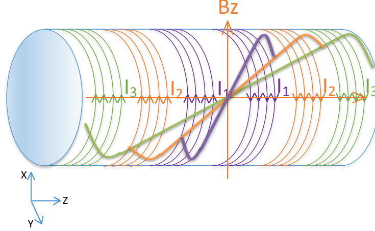
Figure 2.1: Proposed array configuration for the z-gradient coil gives flexibility in generating the desired current density for each section hence improving performance in terms of PNS by linear magnetic field generation in smaller regions.
