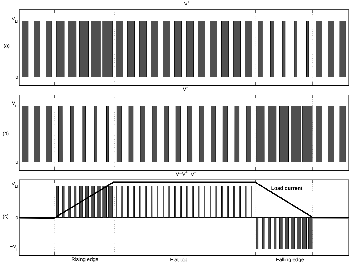
Figure 2.5: Typical PWM pulses for right (a) and left (b) half bridges required to get desired duty cycle on the load to get the trapezoidal load current (c).
