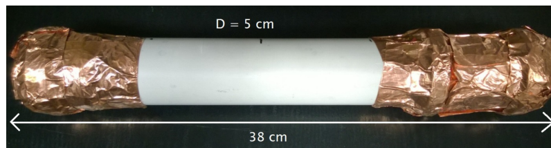
Figure 2.12: Cylindrical phantom shielded to prevent excitation of unwanted regions.
