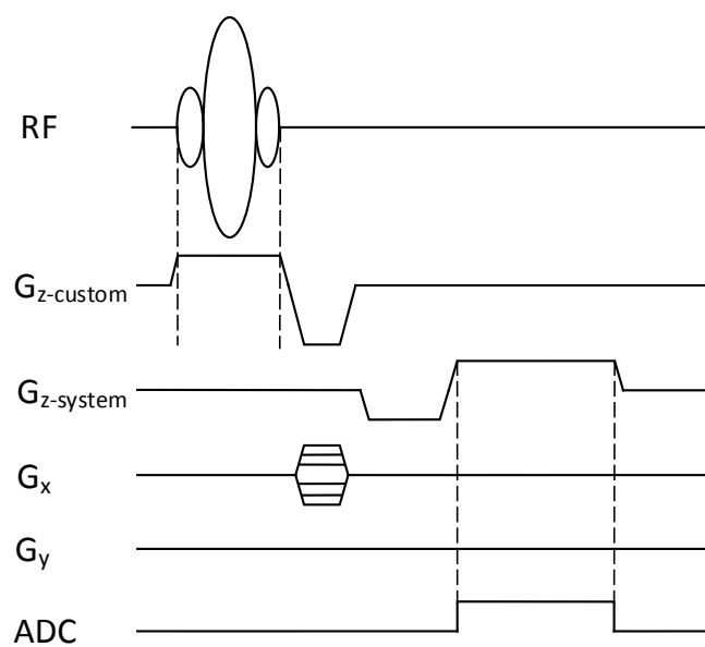
Figure 2.13: Pulse sequence for 2D slice selection using custom coil and read-out using system gradient.
