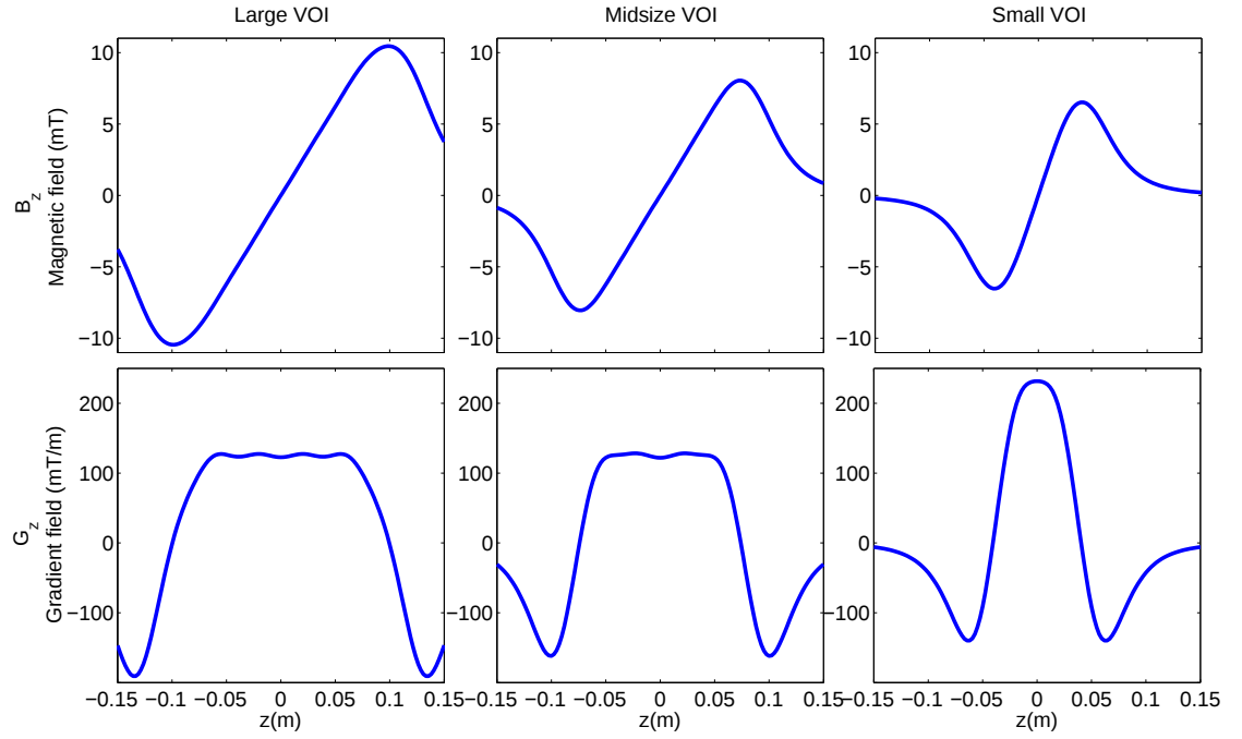
Figure 3.2: The magnetic field and its derivative on the z axis with a: currents ratios of 3.1 : 2.3 : 1 A, b: 0 : 3.1 : 1 A, c: 0 : 0 : 3.1 A for outer, middle and inner channels, respectively applying 30 A as maximum current.
