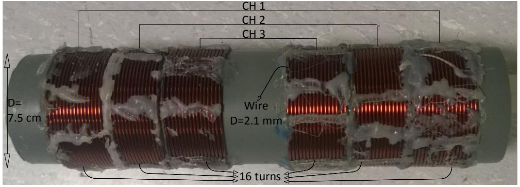
Figure 2.2: The z-gradient coil prototype with specified turn number for each channel and former diameter.
