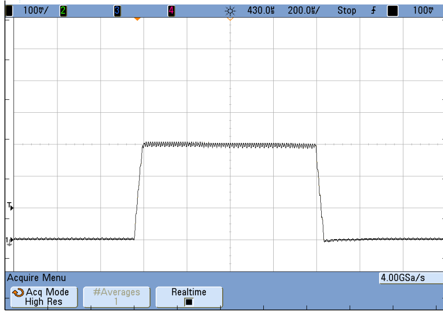
Figure 3.6: Measured current waveform passing through the custom coil by a current probe at 10 mV/A .
