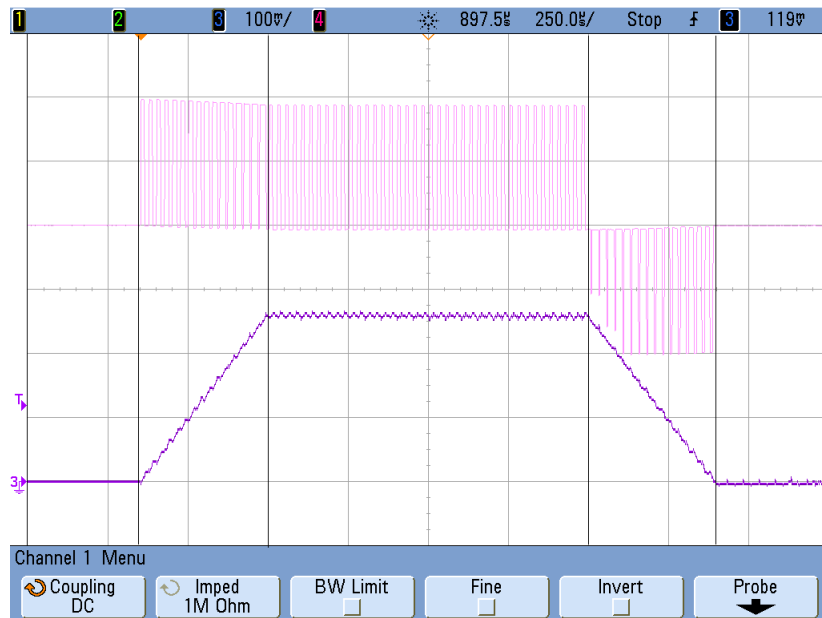
Figure 3.7: Measured current and voltage of a coil with 730 \mu H inductance and 1.82 \Omega resistance and 26 A flat top current value.
