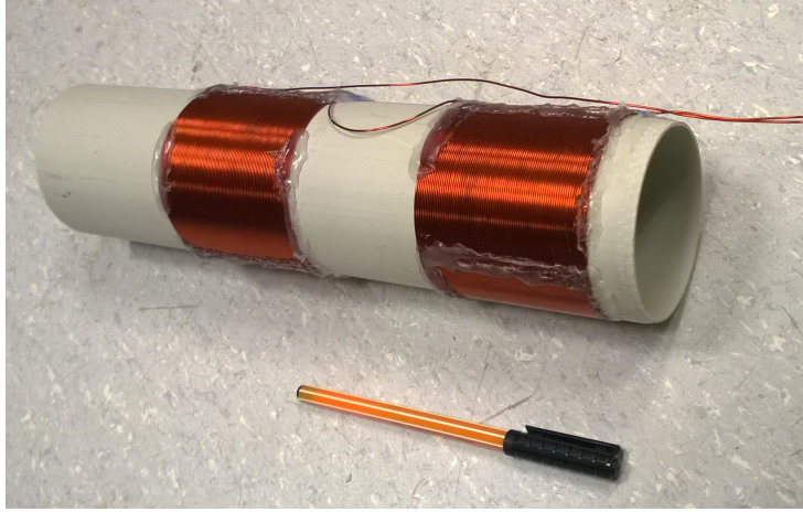
Figure 2.9: Gradient coil with high inductance and impedance in order to test the GPA and measure its efficiency.
