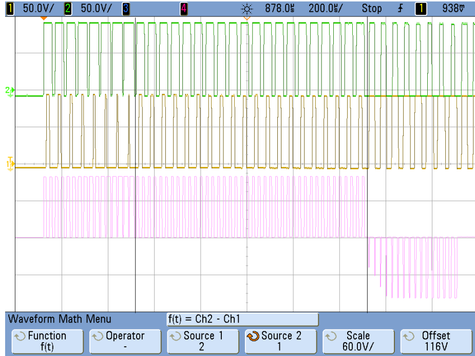
Figure 3.5: Floating Voltage at the output of the GPA (Ch1, Ch2) and their subtraction (bottom) as PWM pulses seen by the load.
