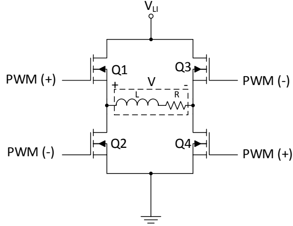
Figure 2.4: H-bridge amplifier driving the coil modeled with an inductor and total DC and AC resistance consisting of four switches with the line voltage V_{LI} and control signals responsible for applying either positive (+) or negative (-) voltage on the load.
