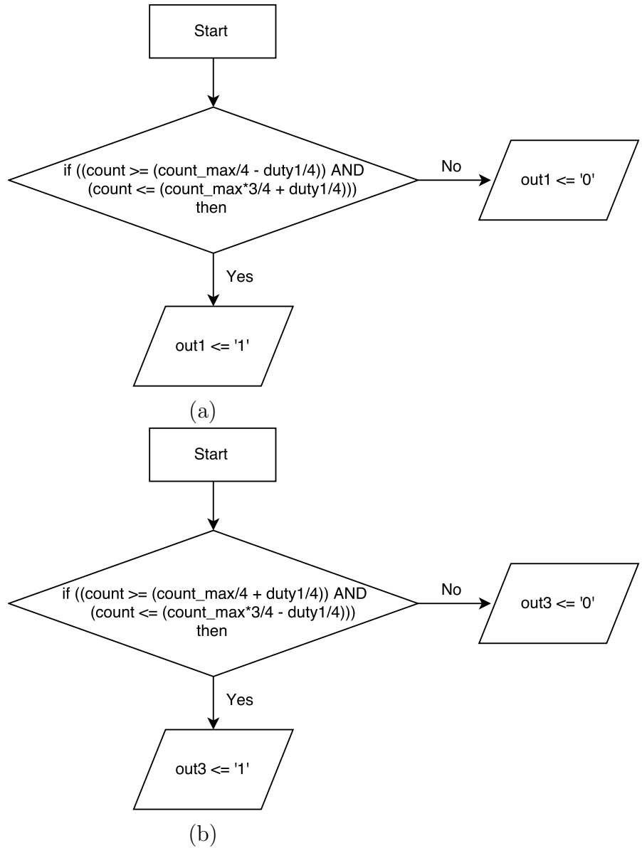
Figure 2.11: Signal generation flow chart for D^+ (a) and D^- (b) duty cycles for Q1 and Q3 switches, respectively.
