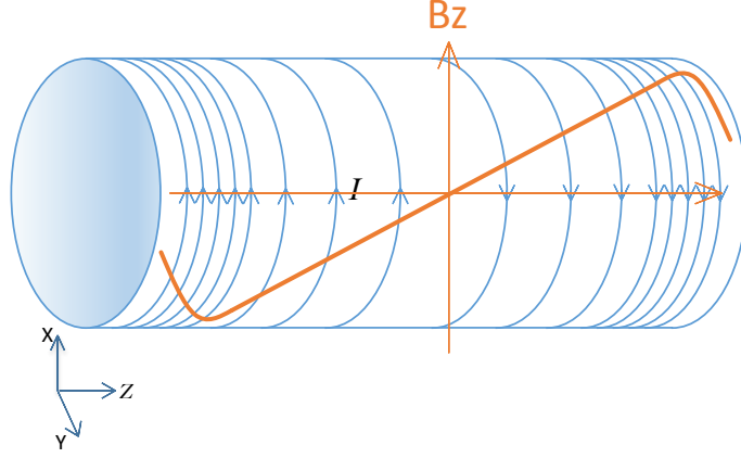
Figure 1.1: Conventional gradient coil for z-direction with discrete wires positioned to approximate current density at those paths carrying same current to generate linear magnetic field inside the desired region.
