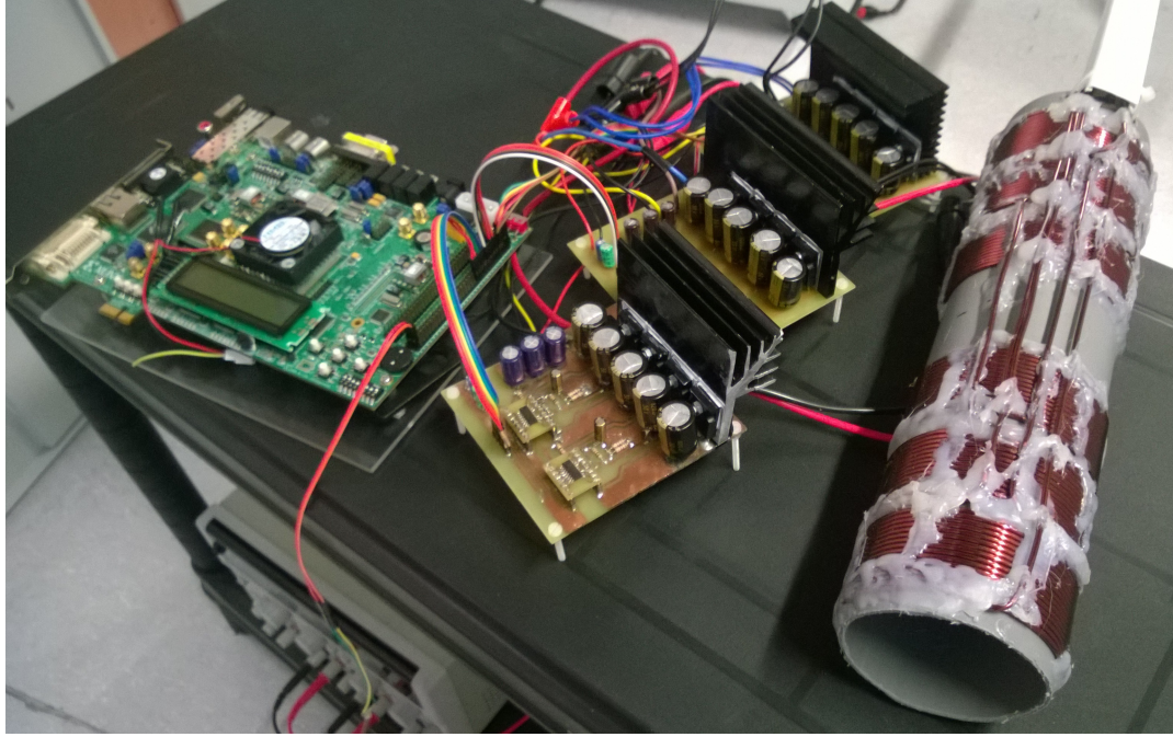
Figure 2.7: Winded gradient coil along with custom made GPAs controlled by an FPGA which is synced with MRI.
