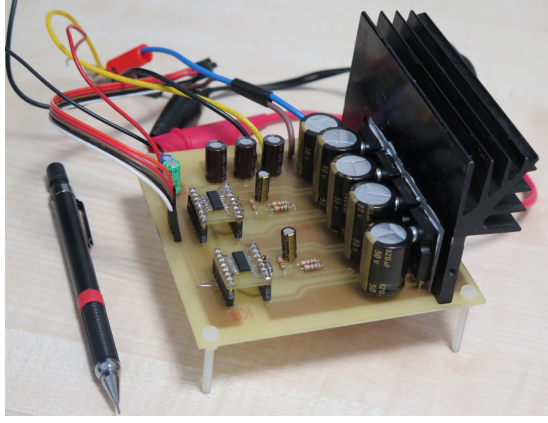
Figure 2.8: GPA prototype with isolated logic and high current side grounds.
