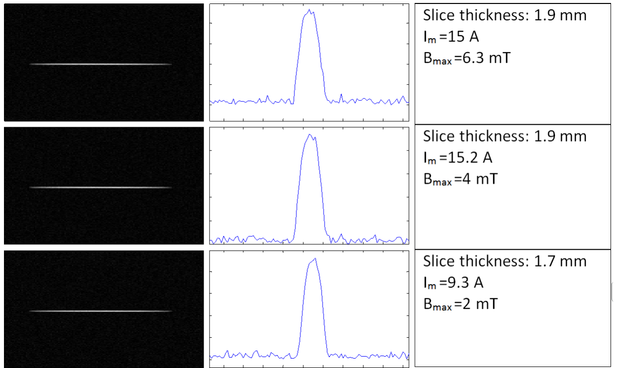
Figure 3.12: 2D coronal slice selection at xy plane along with center line plot for almost equal slice thickness from top to bottom for large, mid-size and small VOI with fixed RF duration ( 800 \mu s ) showing B_{max} change for each case.
