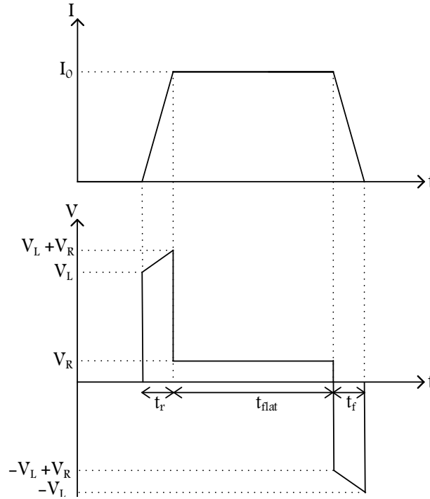
Figure 2.3: Typical gradient current waveform and required voltages to generate it.
