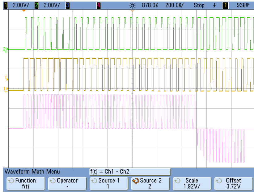
Figure 3.4: PWM pulses at the output of the FPGA for left (Ch1) and right (Ch2) half-bridges for high side switches and their subtraction as desired duty cycle (bottom) for a trapezoidal current.
