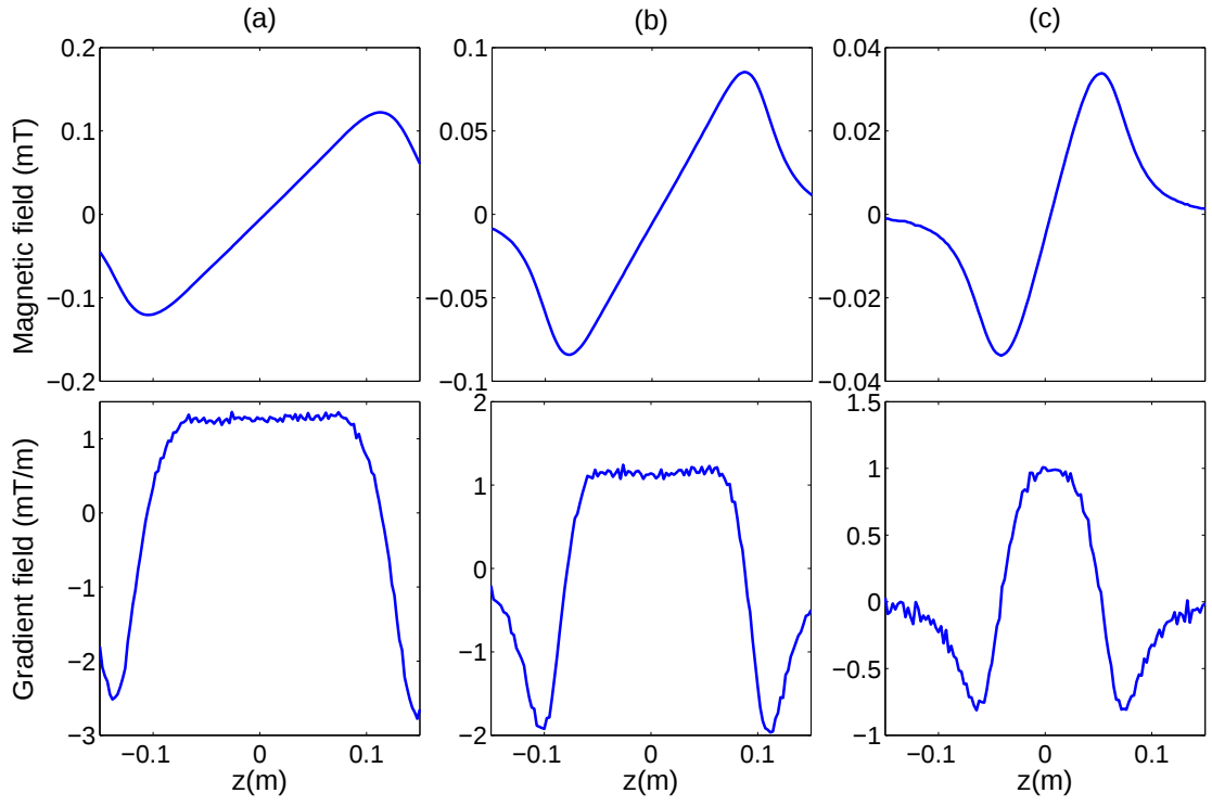
Figure 3.9: Measured magnetic fields and its derivative for a: 0.29 : 0.2 : 0.11 A, b: 0 : 0.26 : 0.09 A, c: 0 : 0 : 0.15 A for outer, middle and inner channels, respectively.
