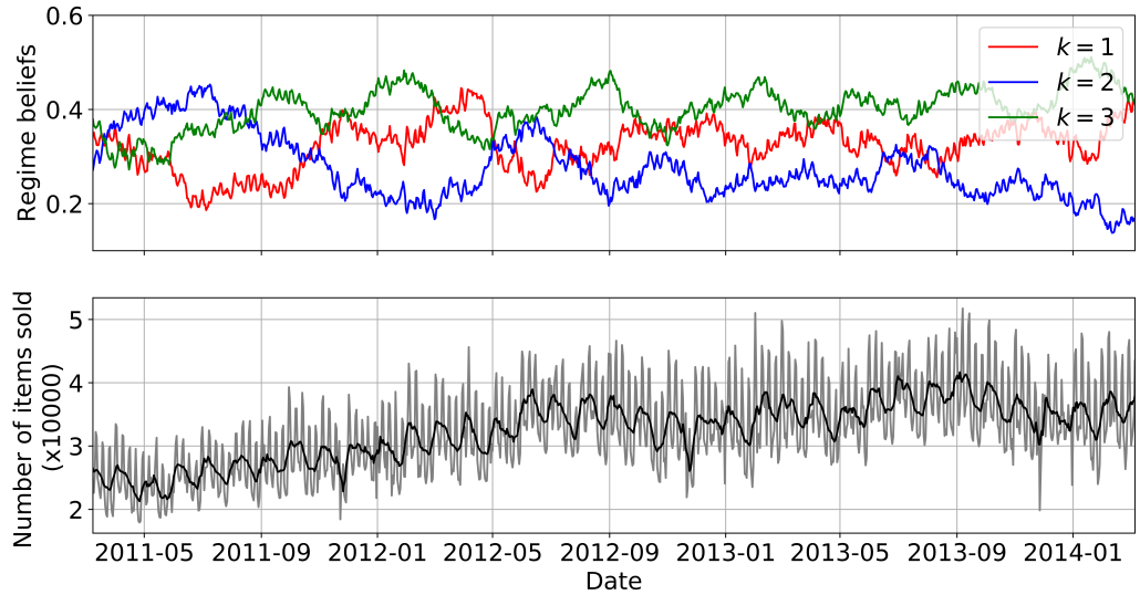
(b) Filtered regime beliefs of Markovian RNN and data sequence for Sales dataset
