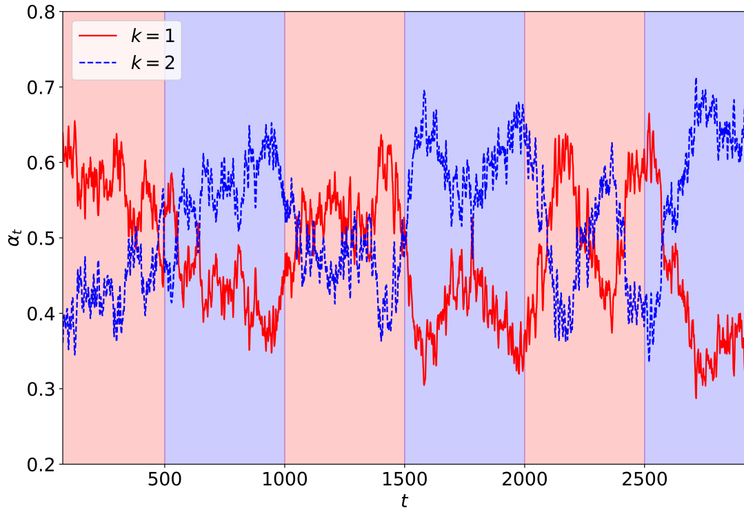
Figure 4.2: Regime beliefs of Markovian RNN for AR process sequence with deterministic switching. Here, background colors represent the real regime value, where red color is used for the first regime and blue color is used for the second regime. Our model can properly distinguish between the two regimes except a short-term undesired switch around t = 2300 , thus the resulting regime belief values are consistent with the real regimes.
