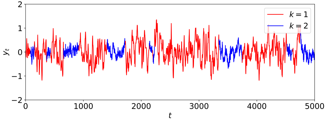
(b) AR(3) process with two regimes and Markovian switching
