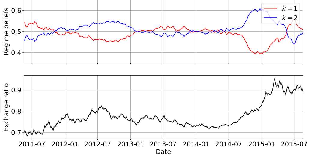
(a) Filtered regime beliefs of Markovian RNN and data sequence for USD/EUR dataset
