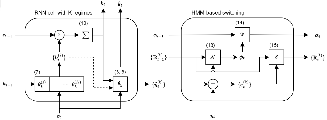
Figure 3.1: Detailed schematic of the Markovian RNN cell. Here, \mathbf{x}_t , \mathbf{y}_t and \hat{\mathbf{y}}_t are the input, target and prediction vectors for the t^{th} time step. \alpha_t and \mathbf{h}_t are the belief state and hidden state vectors respectively. \mathbf{R}_t^{(k)} is the error covariance matrix for the k^{th} regime.
