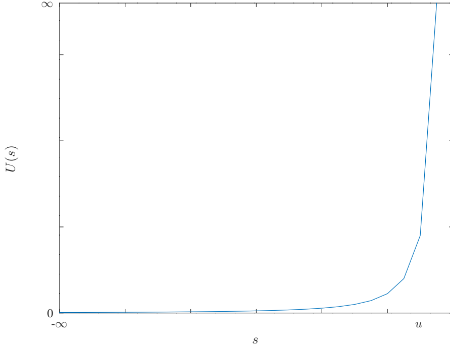
Figure 6.1: Graph of the function U(s)
