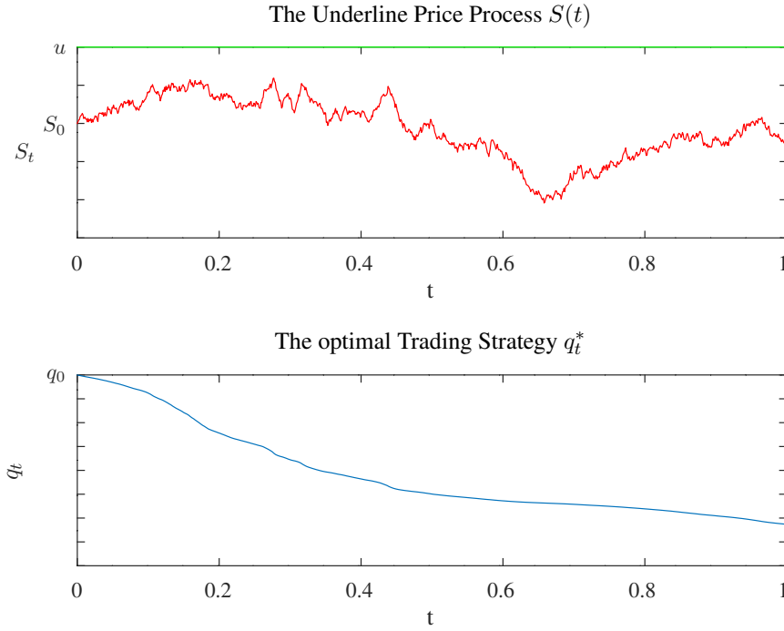
Figure 6.3: Trading Strategy q_t does not liquidate completely as the process S remains below u
