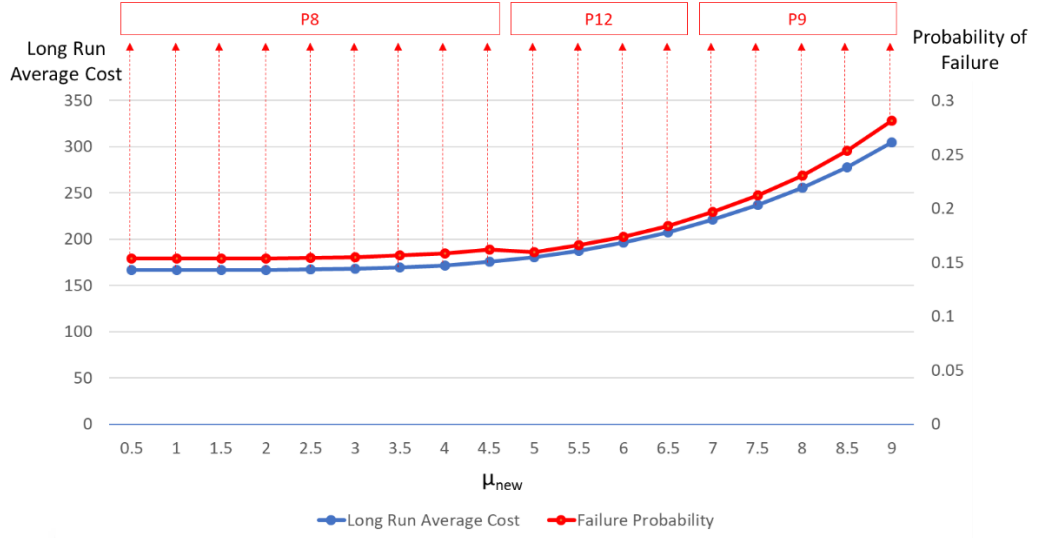
Figure 4.4: Optimal cost, failure probability \pi_F and policy change against \mu_{new} for MMSSR
