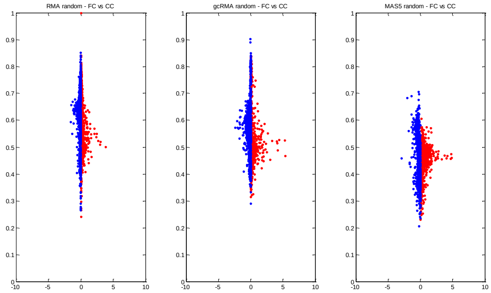
Figure 33. Fold change versus clustering coefficient for the networks of random data. Red dots represent upregulated genes.
