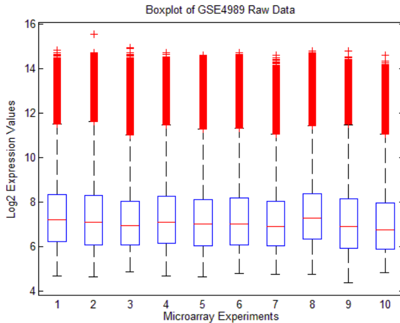
Figure 1. Data distribution of each array before preprocessing
