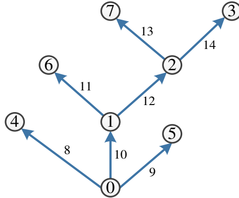
Figure 3.3: Spanning tree of the digraph
