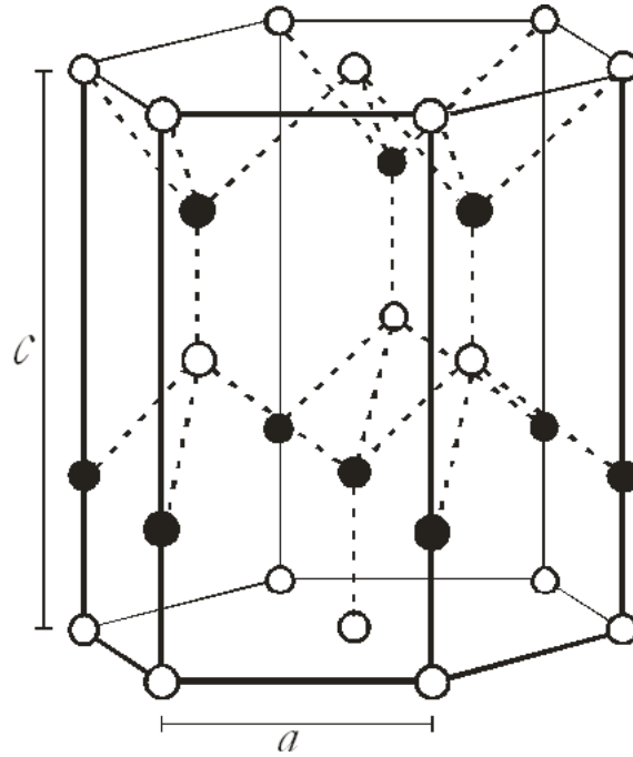
Figure 2.1: Wurtzite crystal of GaN. White atoms can either be Ga or N, depending on the polarity (After Ref. [9]).
