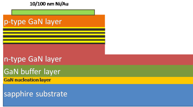
Figure 4.12: Device after p-contact formation.
