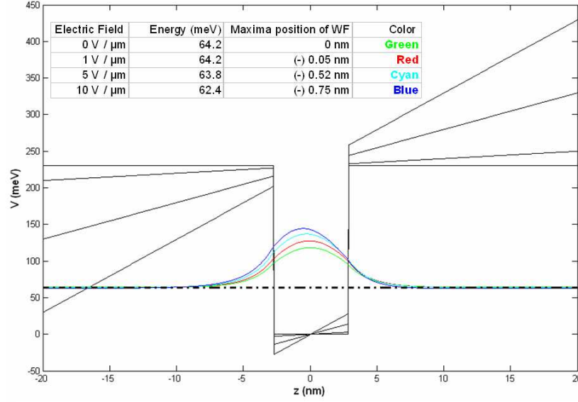
Figure 3.9: Associated electron eigenstates and energy eigenvalues for \text{Al}_{0.3}\text{Ga}_{0.7}\text{As}/\text{GaAs} quantum structure obtained by our TMM based simulation tool (wavefunctions are normalized to different values for visualization purposes).
