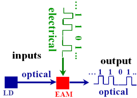
Figure 1.2: Electroabsorption modulator device concept (After Ref. [7]).
