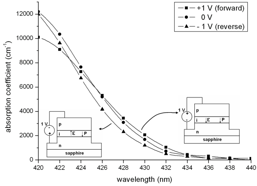
Figure 4.20: Field direction dependent demonstration of reversed and traditional quantum confined Stark effect. E denotes the external electric field and P denotes the polarization-induced electrostatic field inside the quantum well.
