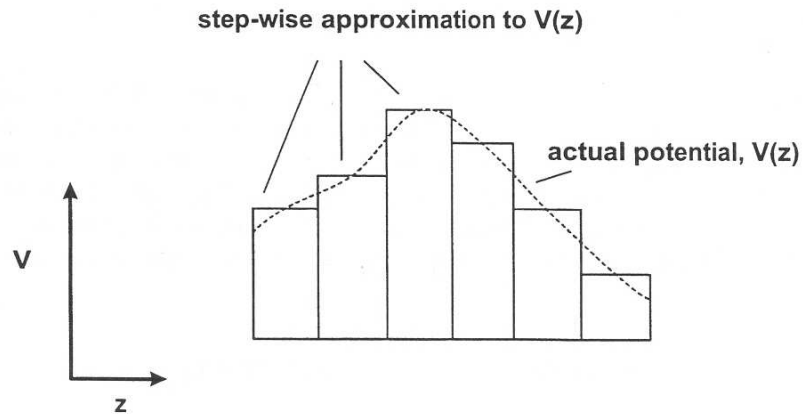
Figure A.1: Discretization of potential profiles in TMM.
