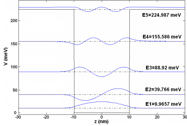
Figure 3.8: Associated energy eigenstates for quantum structure 2, obtained by our TMM based simulation tool.
