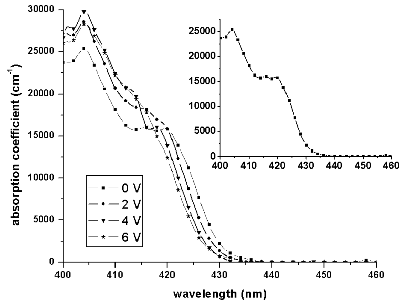
Figure 4.18: Electroabsorption spectra of 4 nm/4 nm InGaN/GaN quantum modulators. Inset shows the 0 V absorption curve separately.
