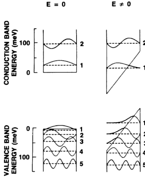
Figure 3.4: Basic concept of quantum confined Stark effect. (After Ref. [14])
