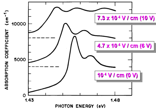
Figure 3.5: Optical absorption spectra for AlGaAs/GaAs quantum well structure for various electric fields applied perpendicular to quantum well layers measured at room temperature. The spectra are shifted vertically to dashed levels for clarity. (After Ref. [14])
