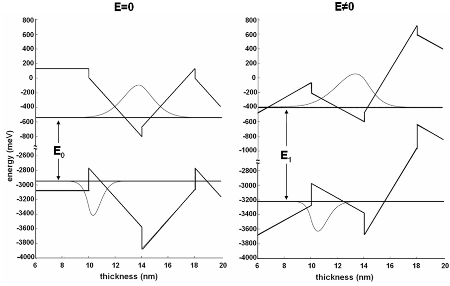
Figure 4.1: Wavefunctions of In_{0.1}Ga_{0.9}N/GaN quantum structures that we calculate using TMM for zero and non-zero external electric field cases.
