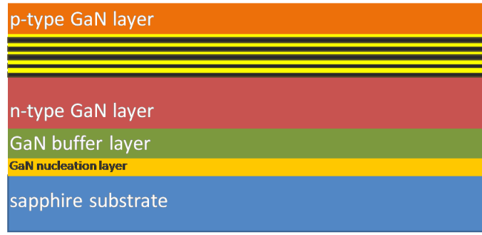
Figure 4.10: Device after cleaning.
