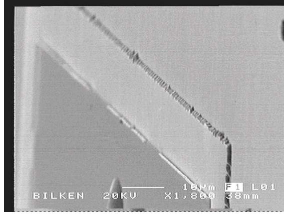
Figure 5.2: Scanning electron micrograph obliquely taken from one of our devices (etched in RIE).
