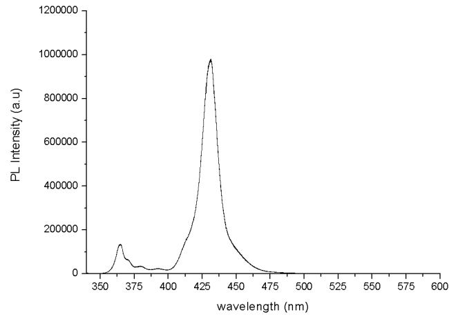
Figure 4.7: Photoluminescence spectrum of one of our epi-wafers
