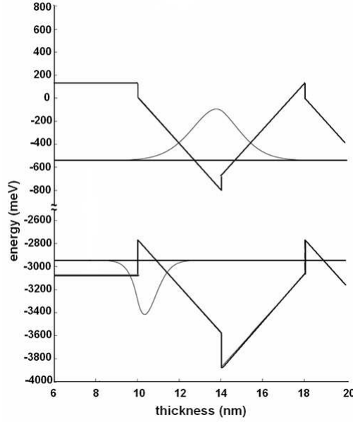
Figure 2.3: A representative band diagram of In_{0.1}Ga_{0.9}N/GaN quantum zigzag structure we obtained by combining the available material parameters and electric field calculations.
