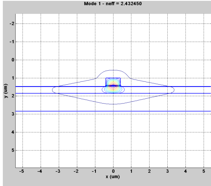
Figure 5.1: Dominant mode E-field profile for one of our rib waveguide designs (in collaboration with M. Yorulmaz of our group).
