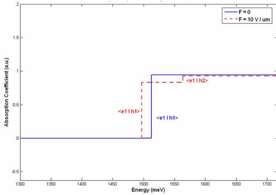
Figure 3.10: Absorption spectra for Al_{0.3}Ga_{0.7}As/GaAs quantum structure for different external electric field intensities obtained by our TMM based simulation tool.
