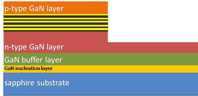
Figure 4.11: Device after mesa etching.
