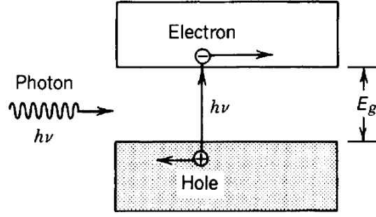
Figure 3.1: Band-to-band absorption in semiconductors (After Ref. [15]).
