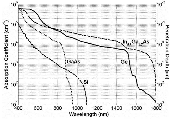
Figure 1.1: Absorption spectra and penetration depth of various semiconductors (After Ref. [5]).
