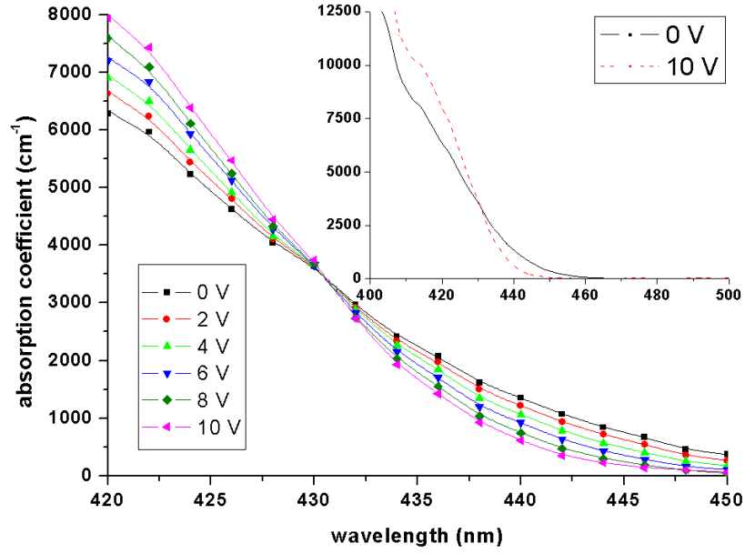
Figure 4.21: Electroabsorption spectra of 2.5 nm/7.5 nm InGaN/GaN heterostructure. Inset shows the 0 V and 10 V absorption curves separately.
