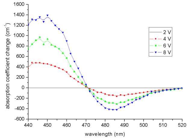
Figure 4.24: Absorption coefficient change with respect to 2 V absorption for the device optimized for 485 nm wavelength of operation.
