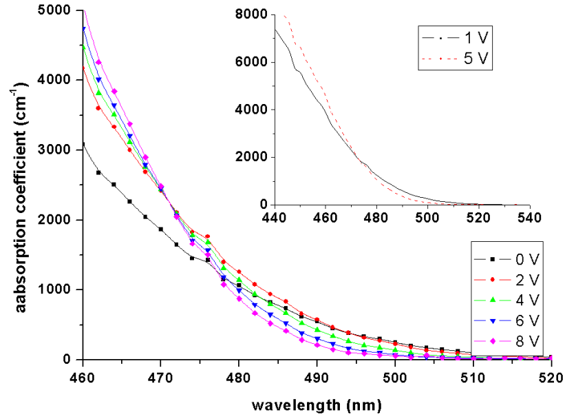
Figure 4.23: Electroabsorption spectra of the device that operates 485 nm for various reverse bias voltage levels. Inset shows the same of 1 V and 5 V bias in a wider spectrum showing a low level of excitonic effects.
