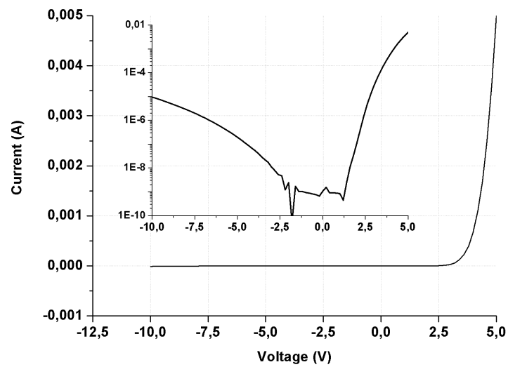
Figure 4.15: IV curve of one of our modulators, inset shows the semilog scale IV characteristics.
