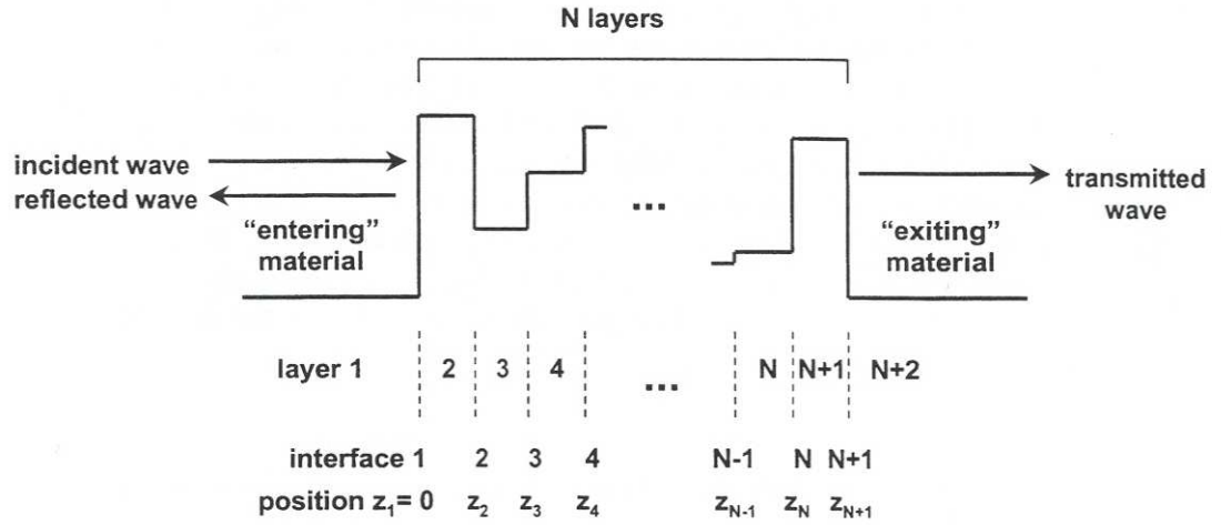
Figure A.2: Transfer matrix method nomenclature (After Ref. [14]).
