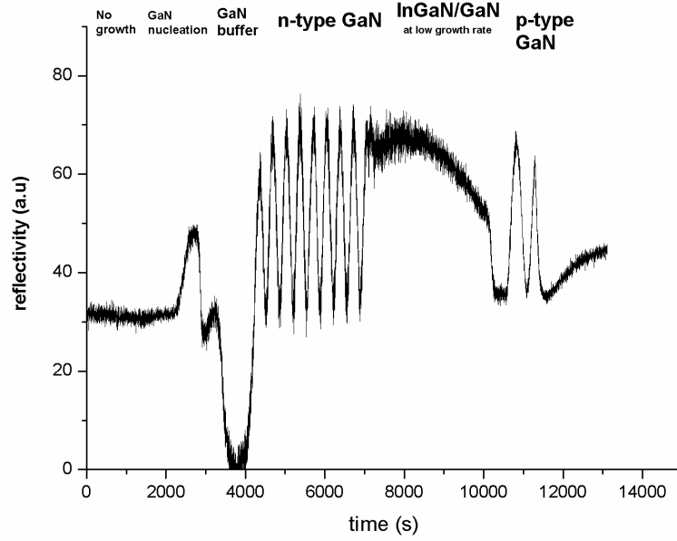
Figure 4.5: In-situ reflectivity measurement results for InGaN/GaN quantum electroabsorption modulator wafer at \lambda=541.4 nm where the wafer is transparent.
