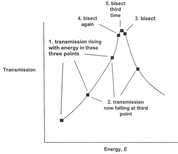
Figure 3.6: Implementation of the tunneling resonance method using bisection method (After Ref. [14]).
