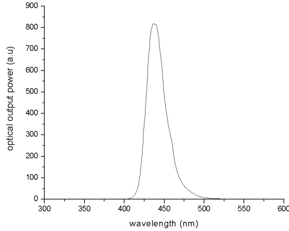
Figure 4.16: Electroluminescence spectrum of one of our modulators.
