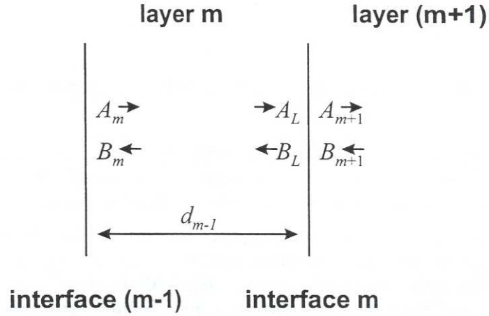
Figure A.3: Definition of waves for an arbitrary layer in TMM (After Ref. [14])
