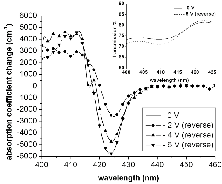
Figure 4.19: Absorption coefficient change with respect to 0 V absorption. Inset shows the transmission spectrum for 0 and 5 V reverse bias.
