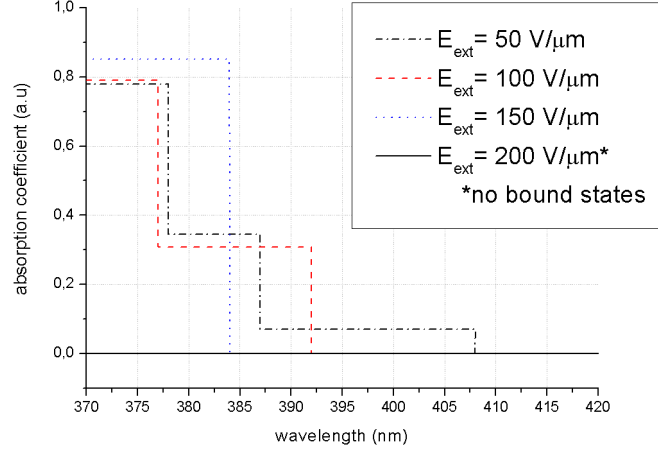
Figure 4.2: Absorption spectra for In_{0.1}Ga_{0.1}N/GaN quantum structures that we calculate using TMM.
