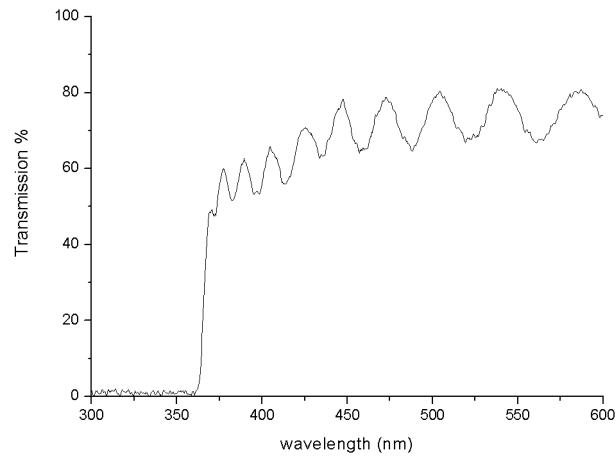
Figure 4.8: A typical wafer transmission spectrum for our InGaN/GaN quantum electroabsorption modulators.
