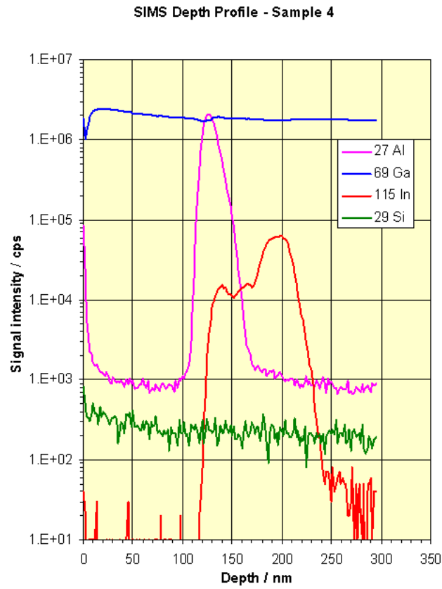
Figure 4.9: SIMS analysis results of one of our wafers with 15 InGa N/ GaN quantum well/barrier structures.
