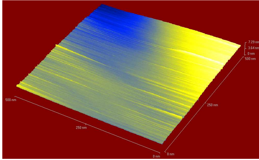
Figure 4.6: 0.5 \mu m \times 0.5 \mu m atomic force microscope image taken from one of our wafers.
