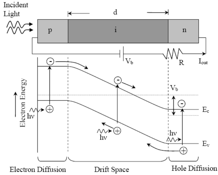
Figure 3.1: Band-to-band absorption in semiconductors (After Ref. [15]).
