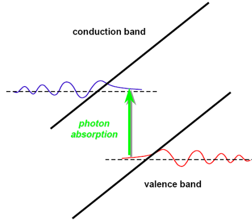
Figure 3.3: Basic concept of Franz-Keldysh effect (After Ref. [14])
