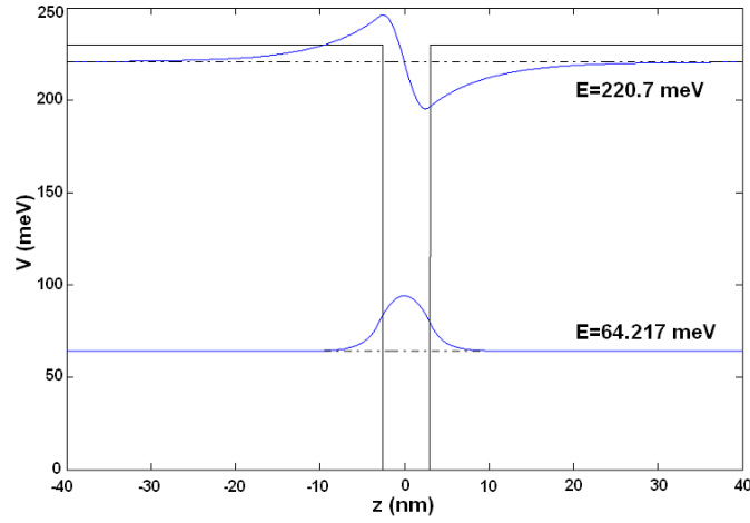
Figure 3.7: Associated energy eigenstates for Quantum Structure 1, obtained by our TMM-based simulation tool.
