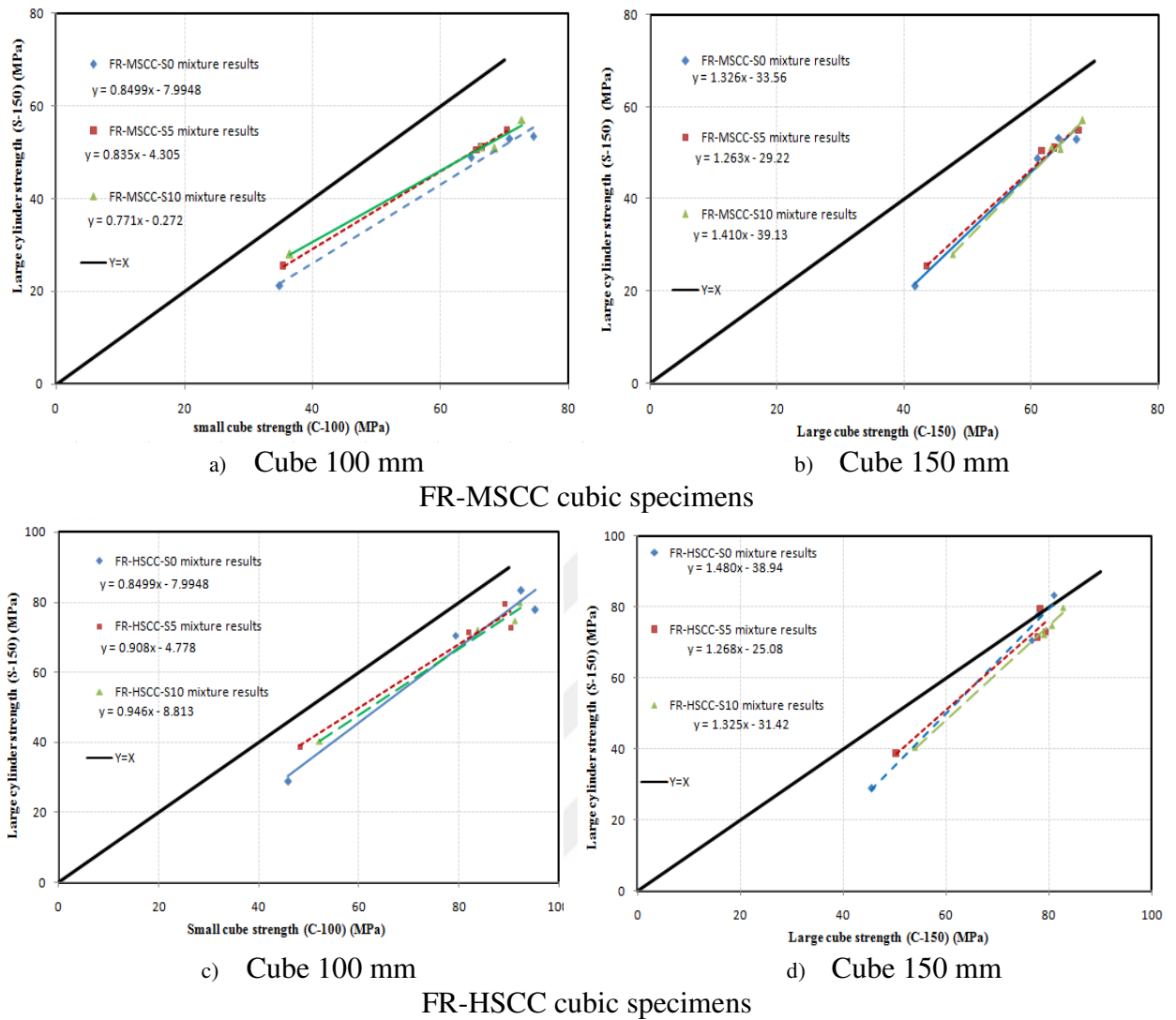
Figure 6.14 Relationship between compressive strengths of the 150 × 300 mm cylinder and cubic specimens before and after exposure to elevated temperatures.
