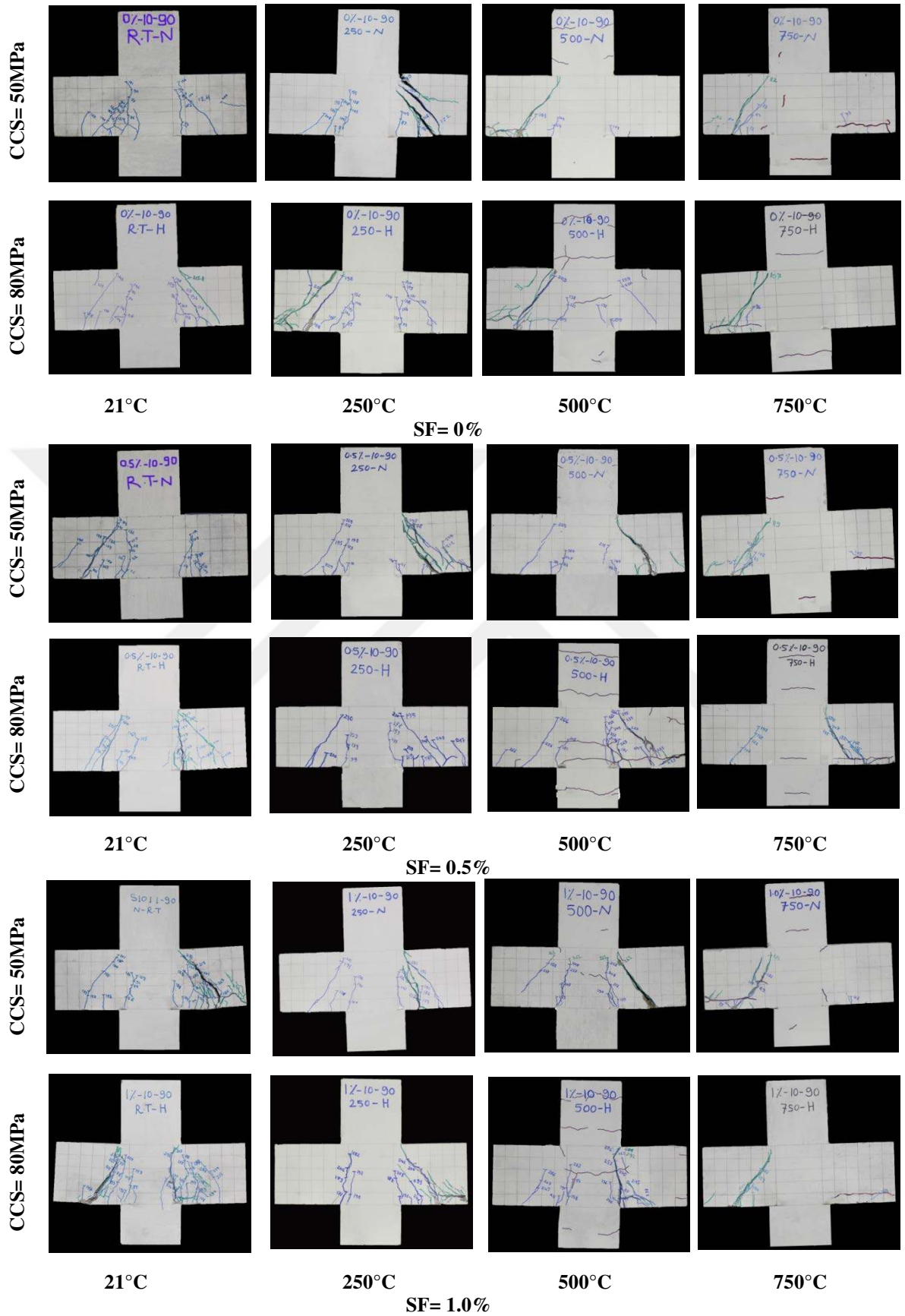
Figure 7.4 Failure modes for RC-corbels with the different values of concrete compressive strength (CCS)
