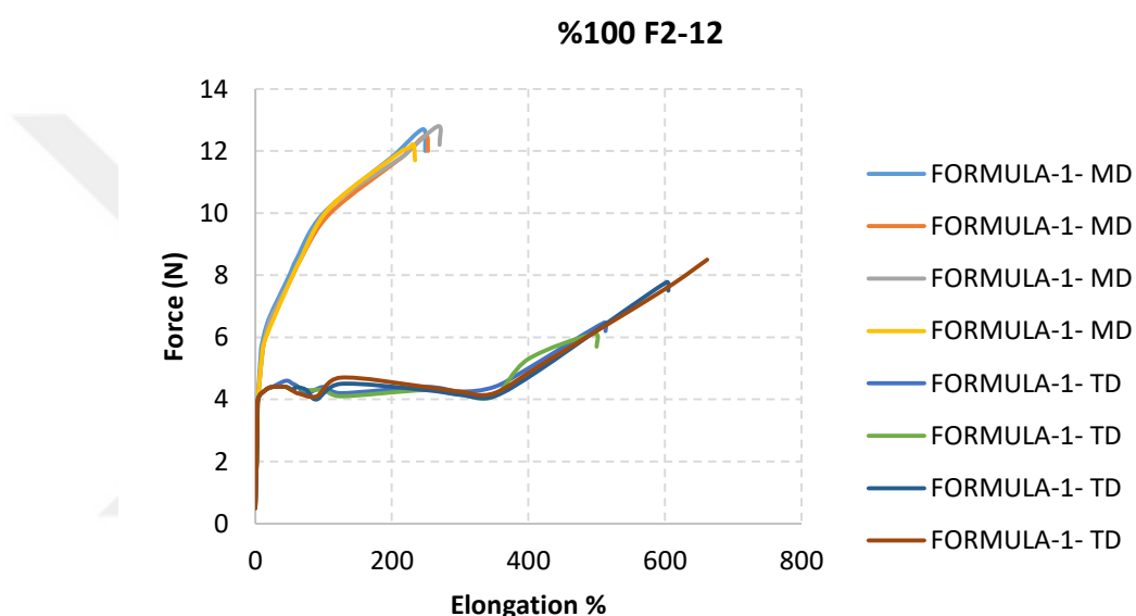
Figure 4.5 %100 F2-12 (pure LDPE film) Force-Elongation Diagram
