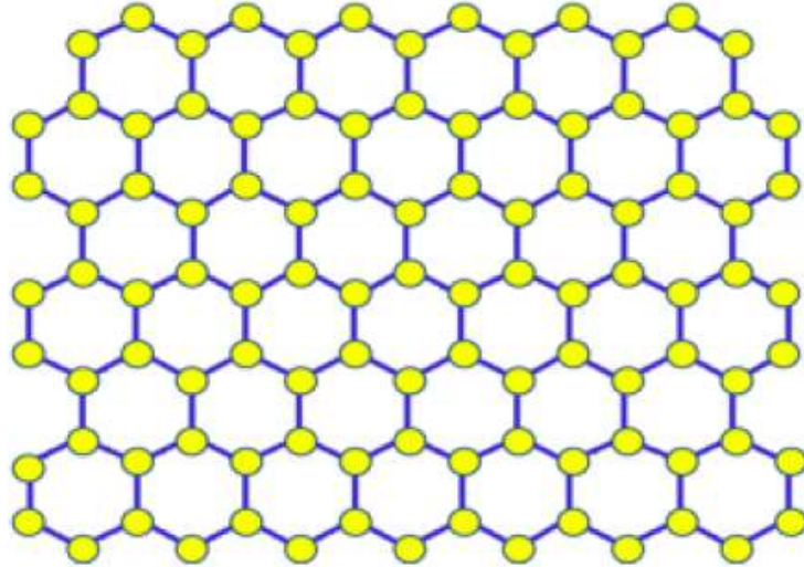
Figure 1.1 Graphene structure [3]
