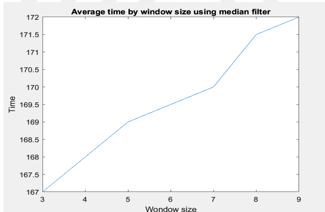
Figure 4.3. Average time by window size using a median filter
