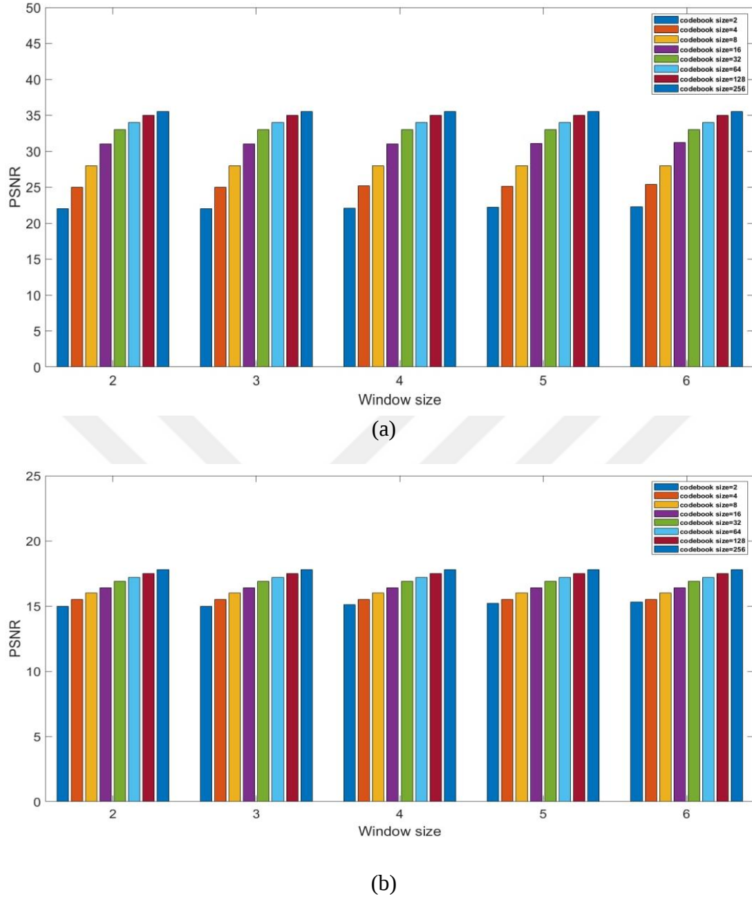
Figure 4.6. Average PSNR per window size for different codebook sizes. (a) Third level and (b) second level
