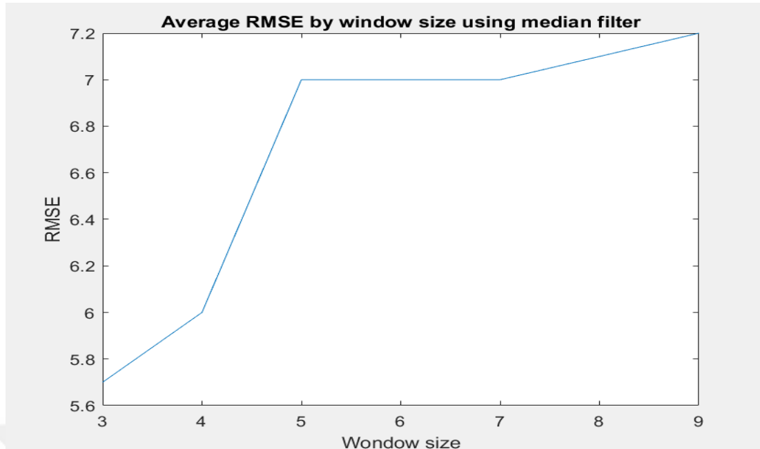
Figure 4.2. Average RMSE by window size using a median filter
