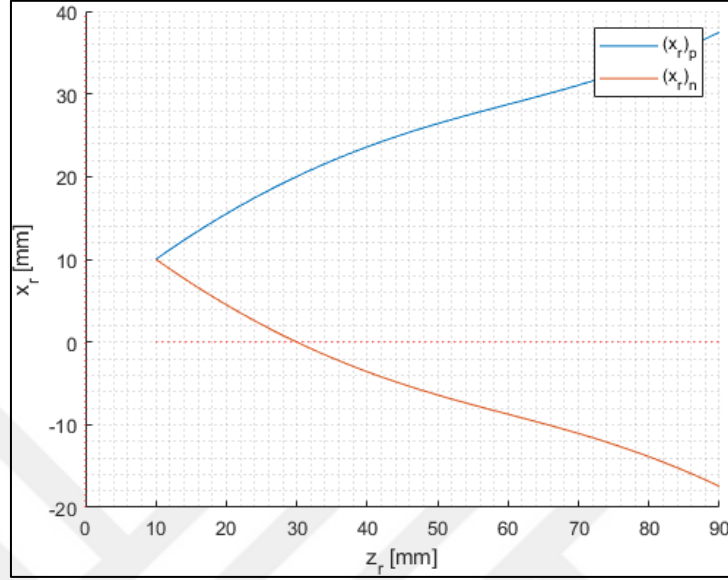
Figure 3.35. Solutions for (x_r)_p and (x_r)_n (for (x_r)_i = 10 , (z_r)_i = 10 )
