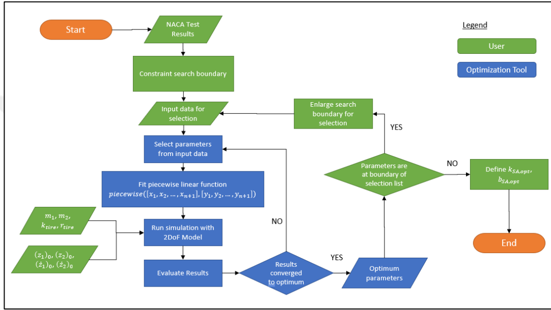
Figure 4.20. Optimization procedure using y_i as decision variables for “piecewise”
