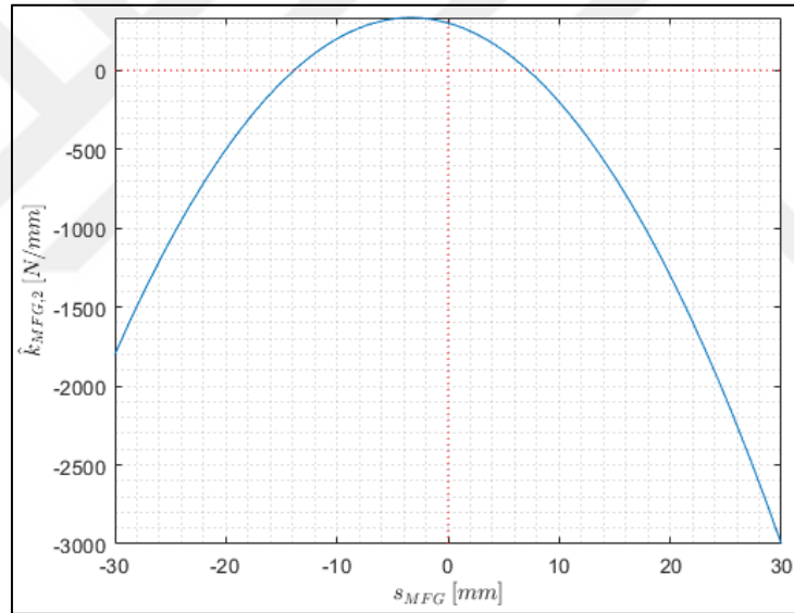
Figure 3.13. Spring stiffness for Spring Case 2
