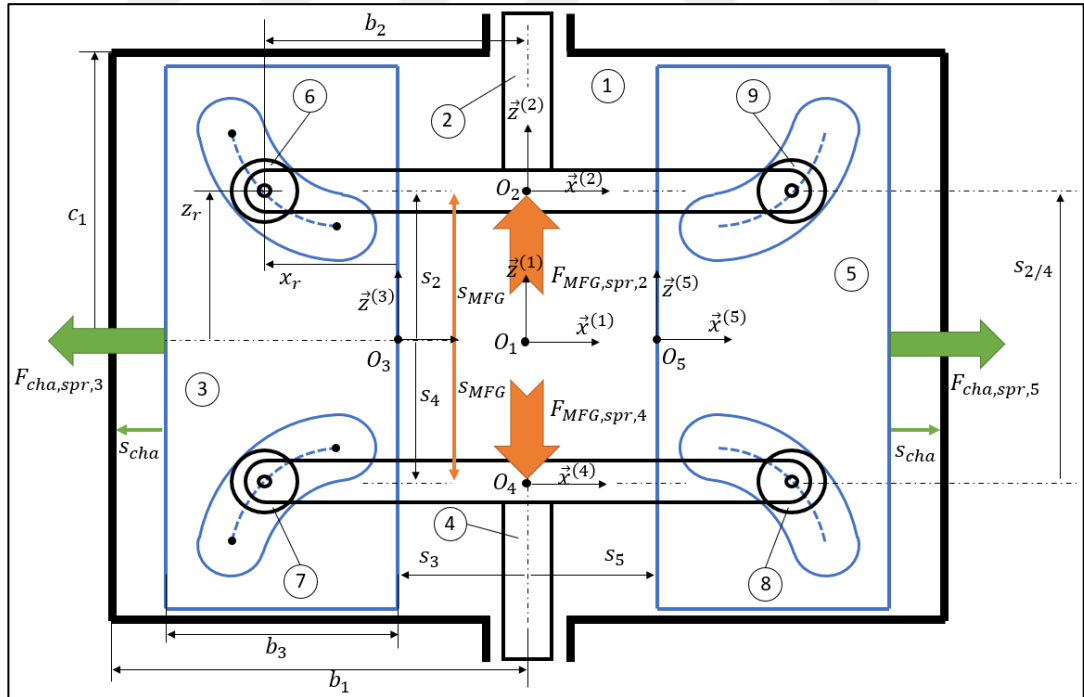
Figure 3.5. Spring forces acting on MFGS
