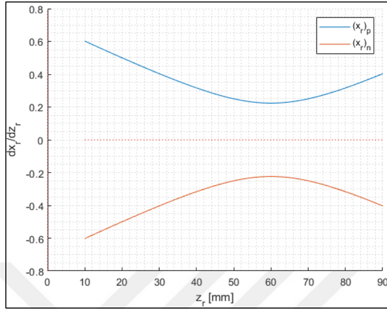
Figure 3.39. Velocity influence coefficient, \frac{dx_r}{dz_r} , for (x_r)_p and (x_r)_n
