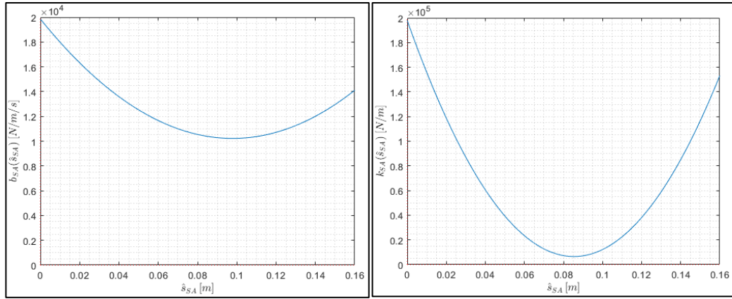
Figure 4.30. 2 nd order polynomial fitting of; b_{SA}(\hat{s}_{SA}) (left), k_{SA}(\hat{s}_{SA}) (right)
