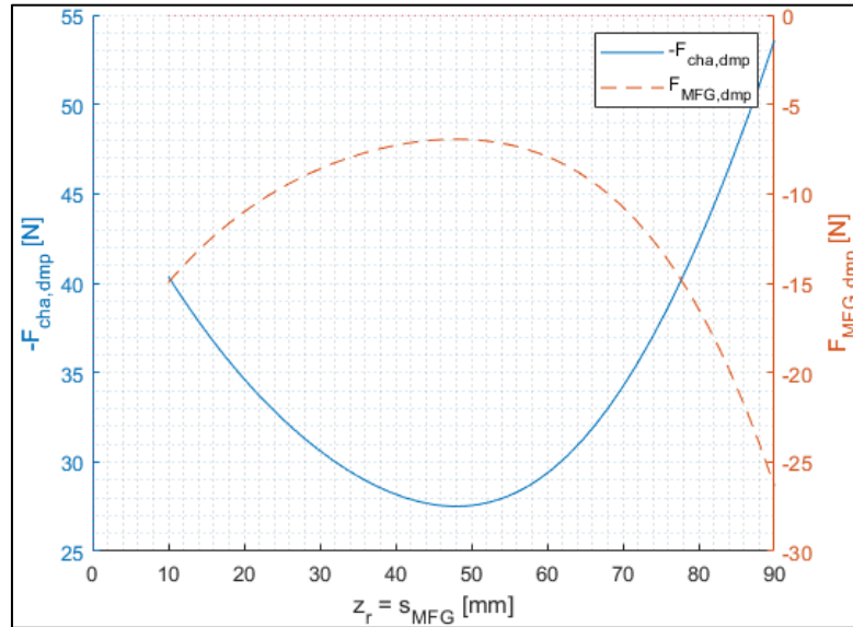
Figure 5.25. F_{MFG,dmp} and -F_{cha,dmp} w.r.t. s_{MFG}
