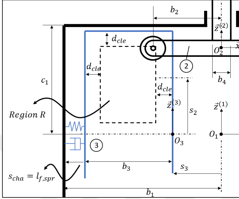
Figure 5.11. Determination b_1 in relation with l_{f,spr}
