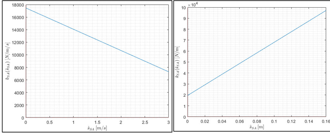
Figure 4.22. 1 st order polynomial fitting of; b_{SA}(\dot{\delta}_{SA}) (left), k_{SA}(\hat{\delta}_{SA}) (right)
