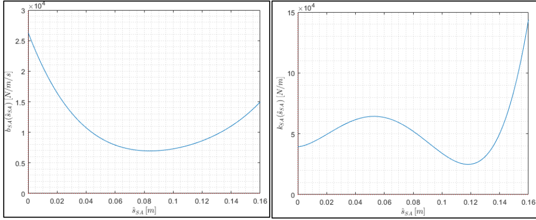
Figure 4.34. 4 th order polynomial fitting of; b_{SA}(\hat{s}_{SA}) (left), k_{SA}(\hat{s}_{SA}) (right)
