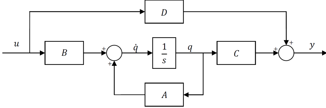
Figure 2.3: Block diagram representation of state space
