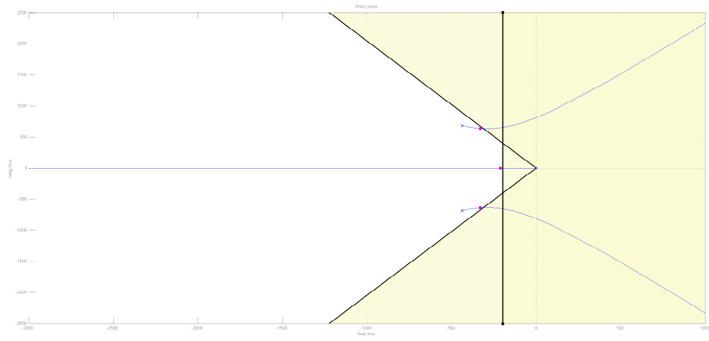
Figure 3.30: Root Locus Diagram for Pole Placement Based Position Control in terms of ITAE index
